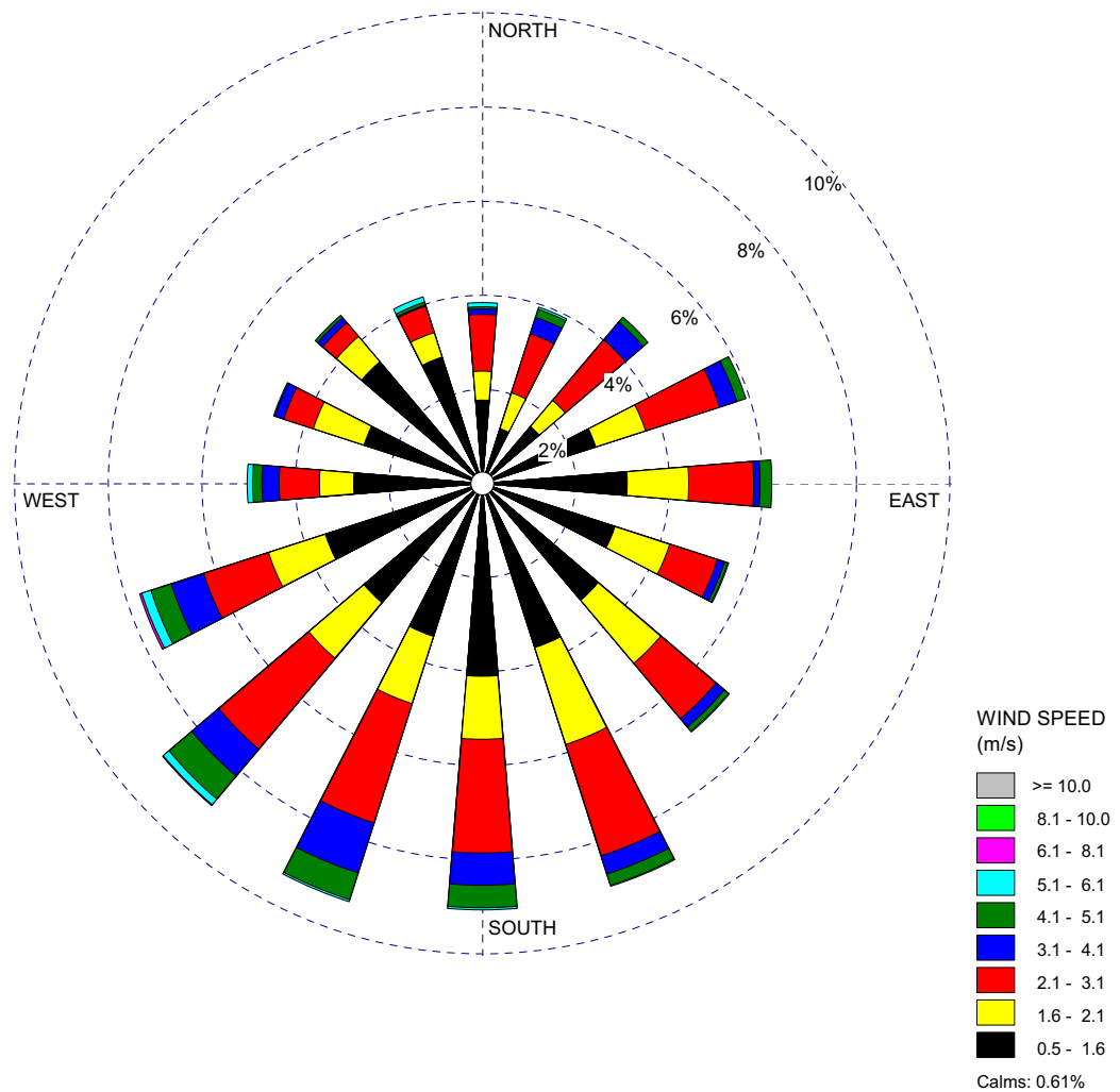
Figure 2.7-5. 10-Meter Level Composite Wind Rose for the Units 2 and 3 Monitoring Program (January 1, 2007–December 31, 2008) — Summer
