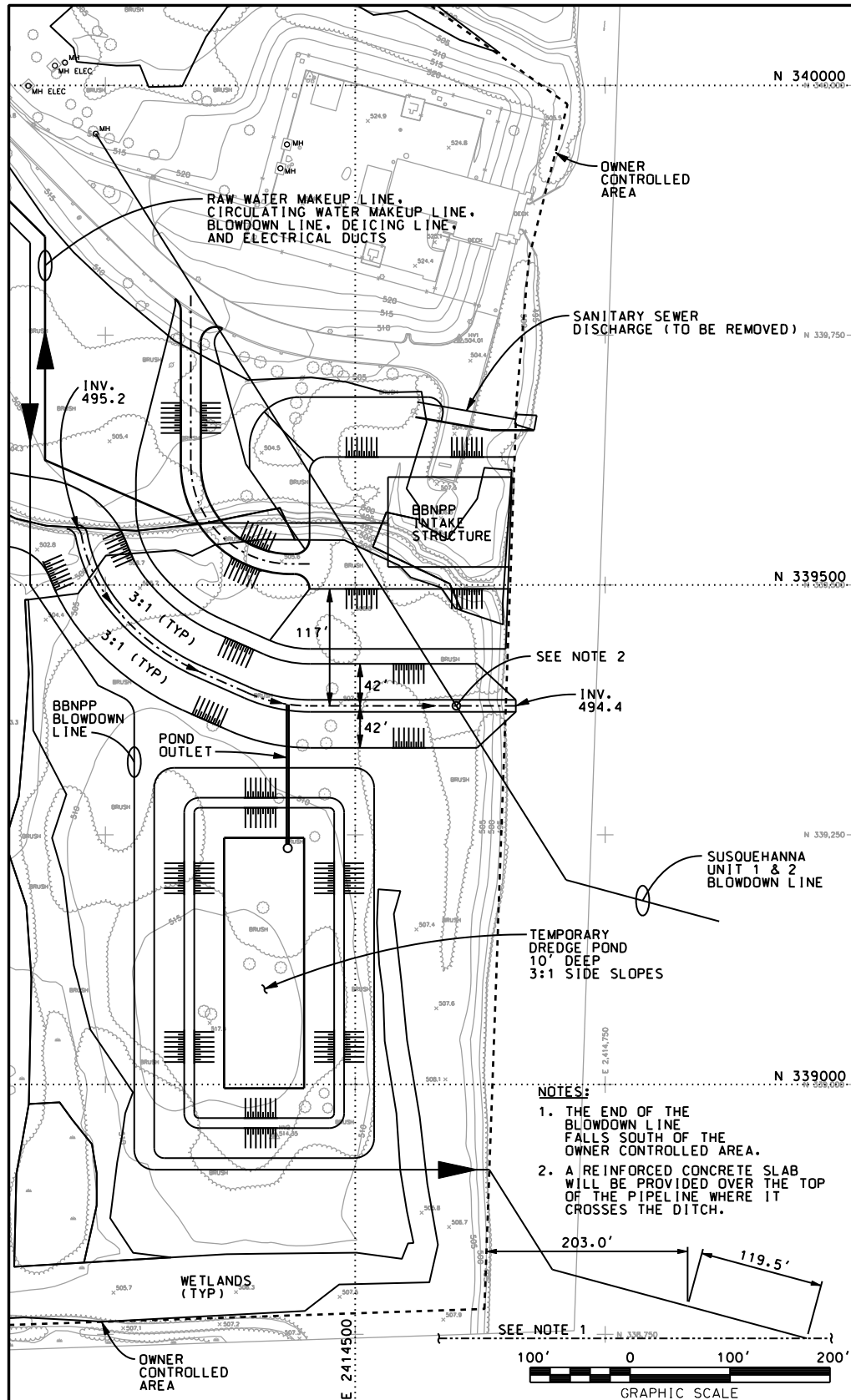
Figure 3.4-3—Circulating Water System Intake/Discharge Structure Location Plan
