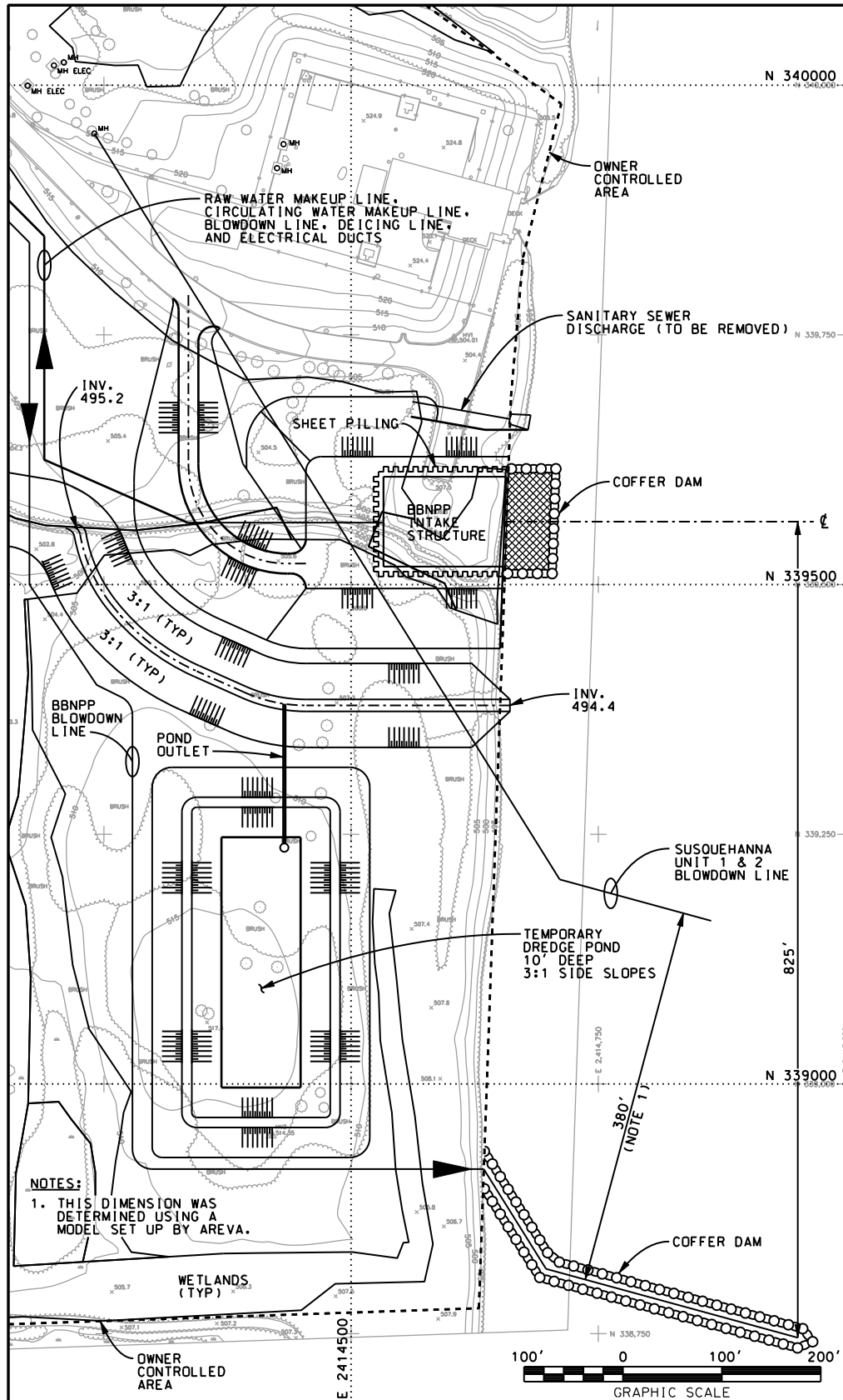
Figure 3.4-11—CWS Makeup Water Intake Structure Construction Cofferdam
