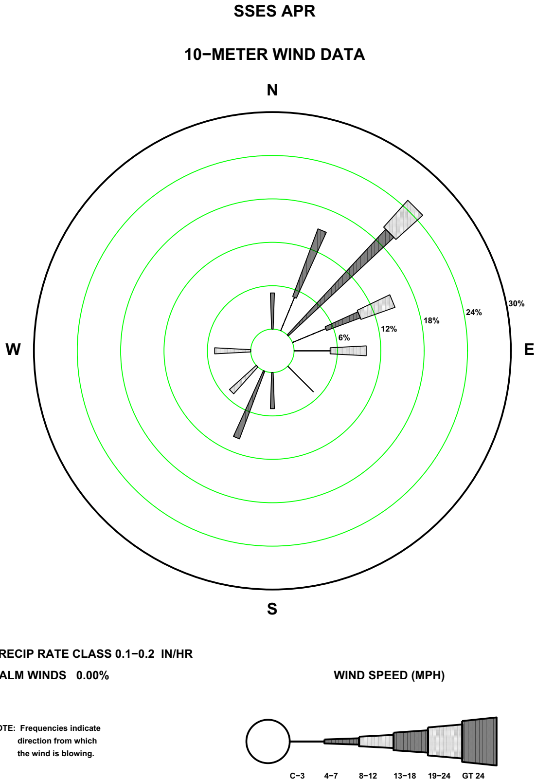
Figure 2.7-34—SSES 10 m April Precipitation Rate Wind Rose
