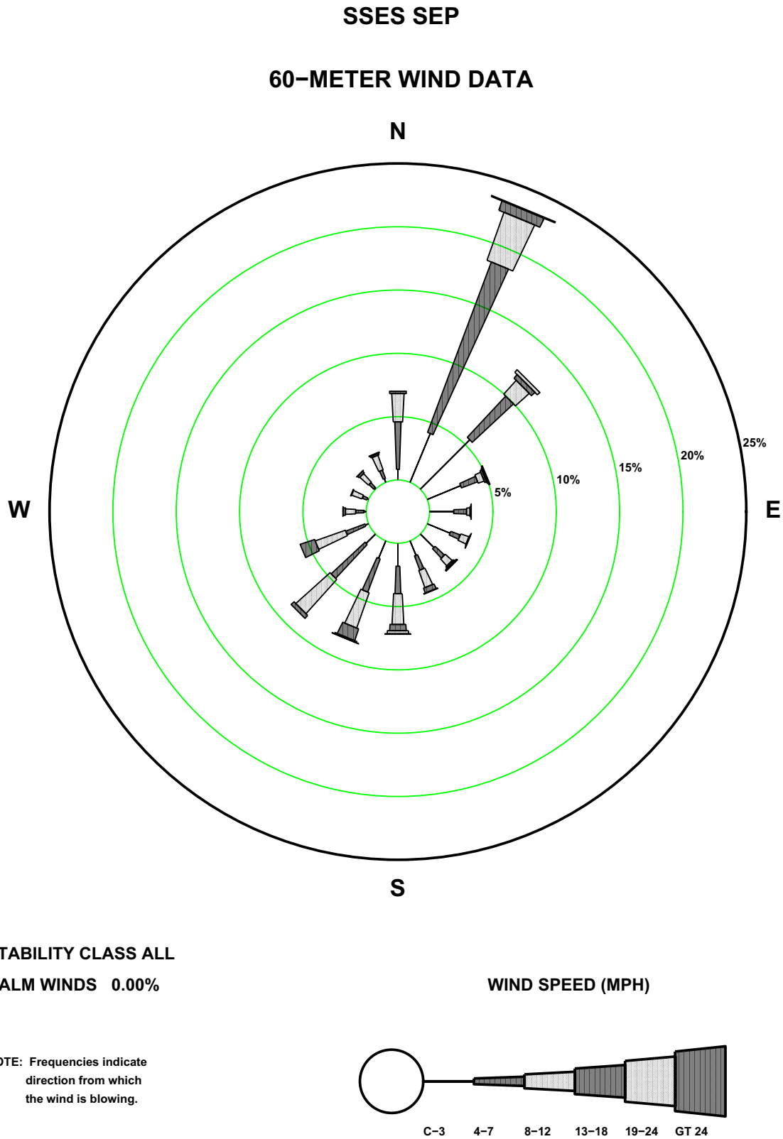
Figure 2.7-85—SSES 60m September Wind Rose
