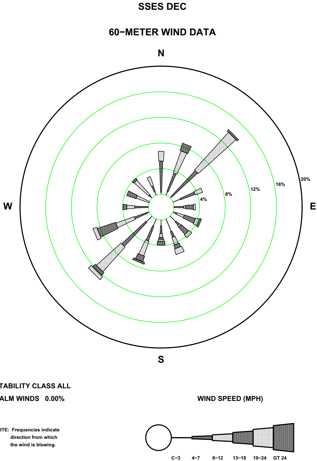
Figure 2.7-29—SSES 60 m December Precipitation Wind Rose
