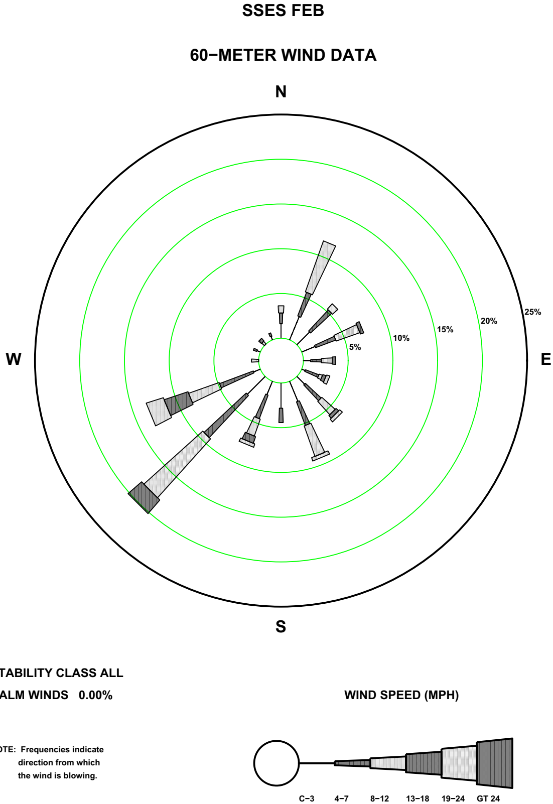
Figure 2.7-19—SSES 60 m February Precipitation Wind Rose
