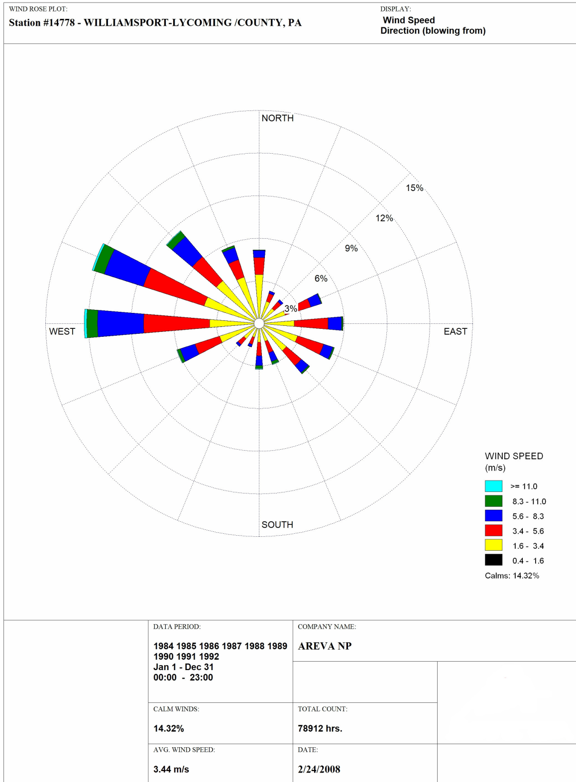
Figure 2.7-91—Williamsport, PA, Wind Rose
