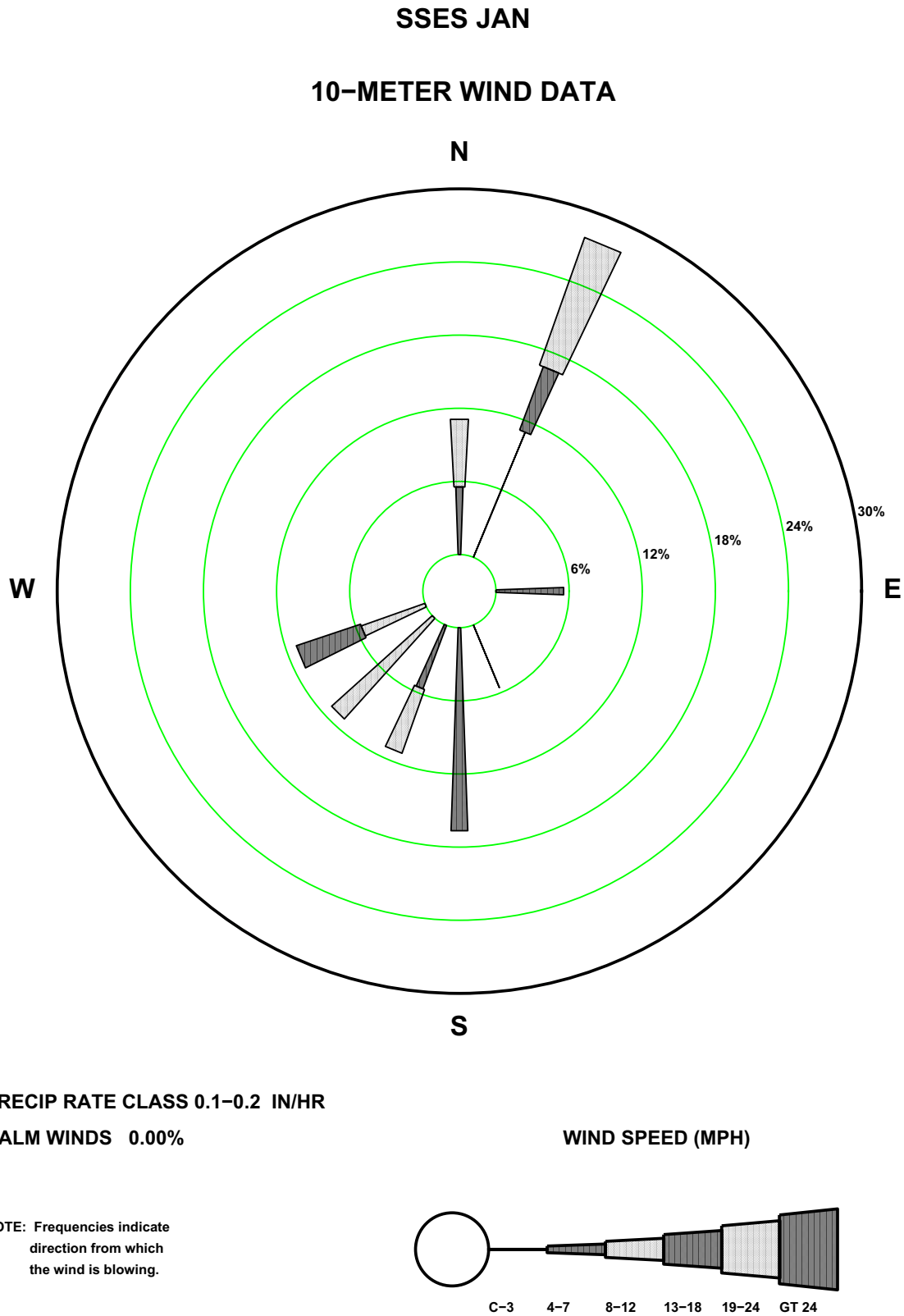
Figure 2.7-31—SSES 10 m January Precipitation Rate Wind Rose
