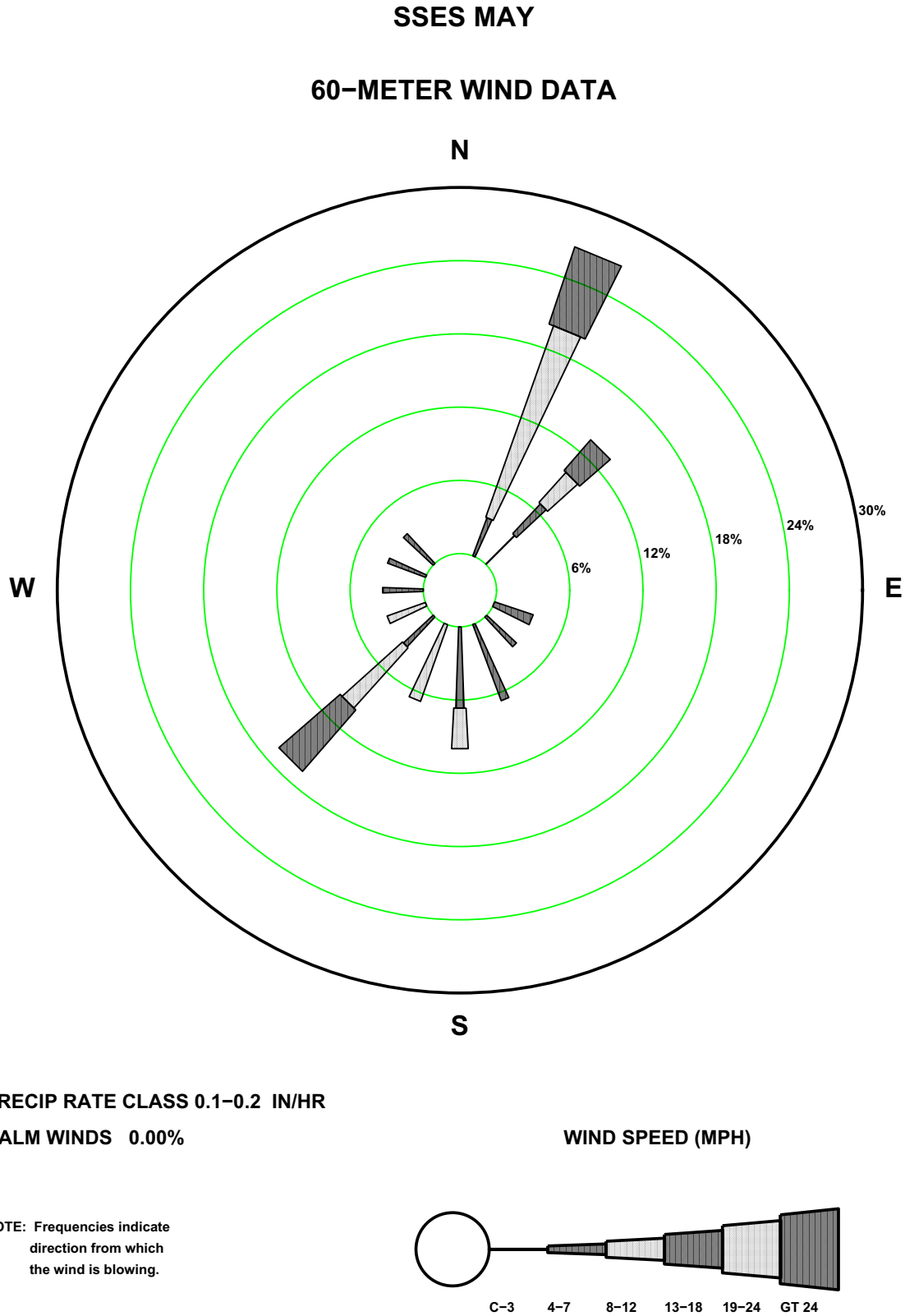
Figure 2.7-47—SSES 60 m May Precipitation Rate Wind Rose
