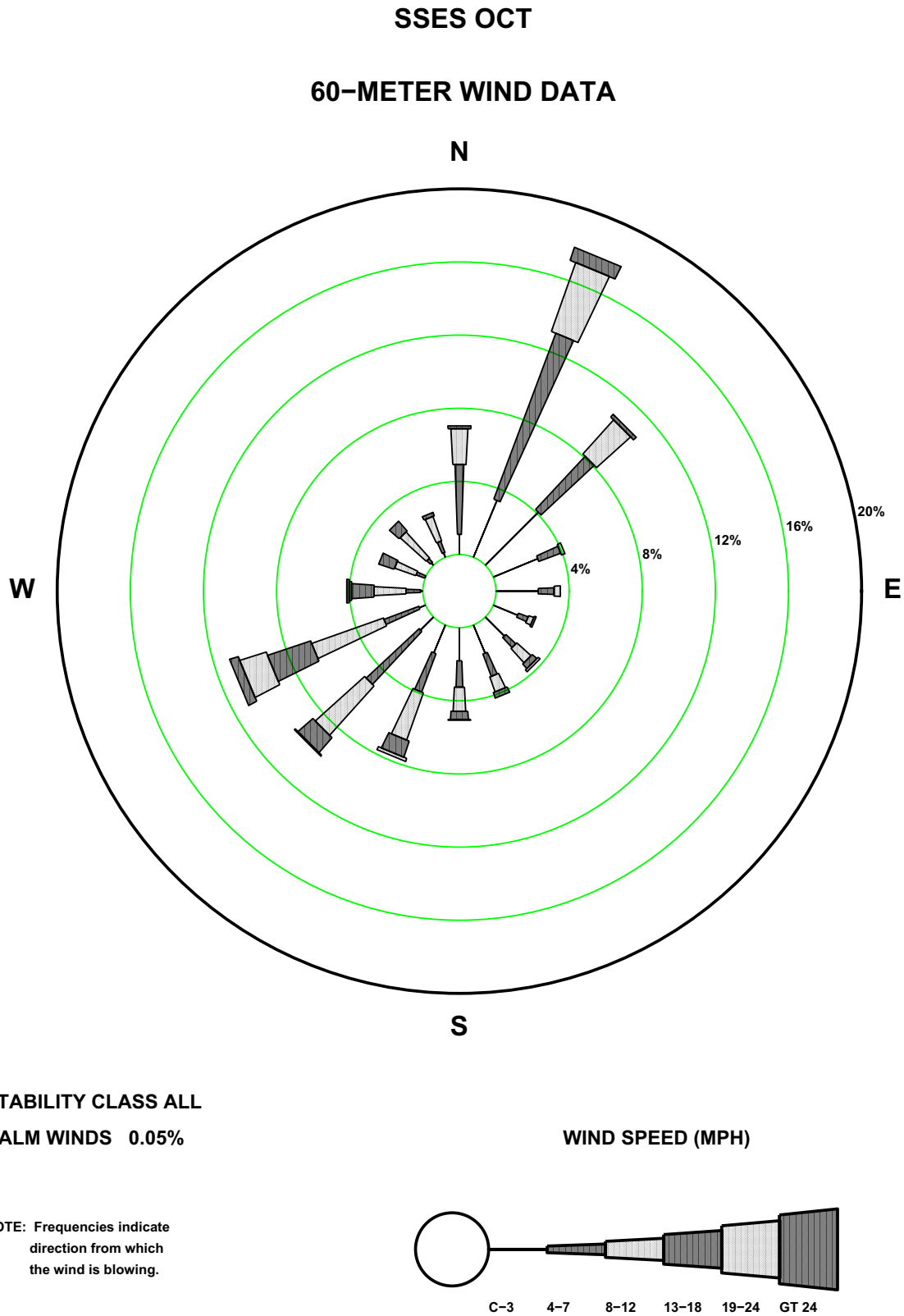
Figure 2.7-86—SSES 60m October Wind Rose
