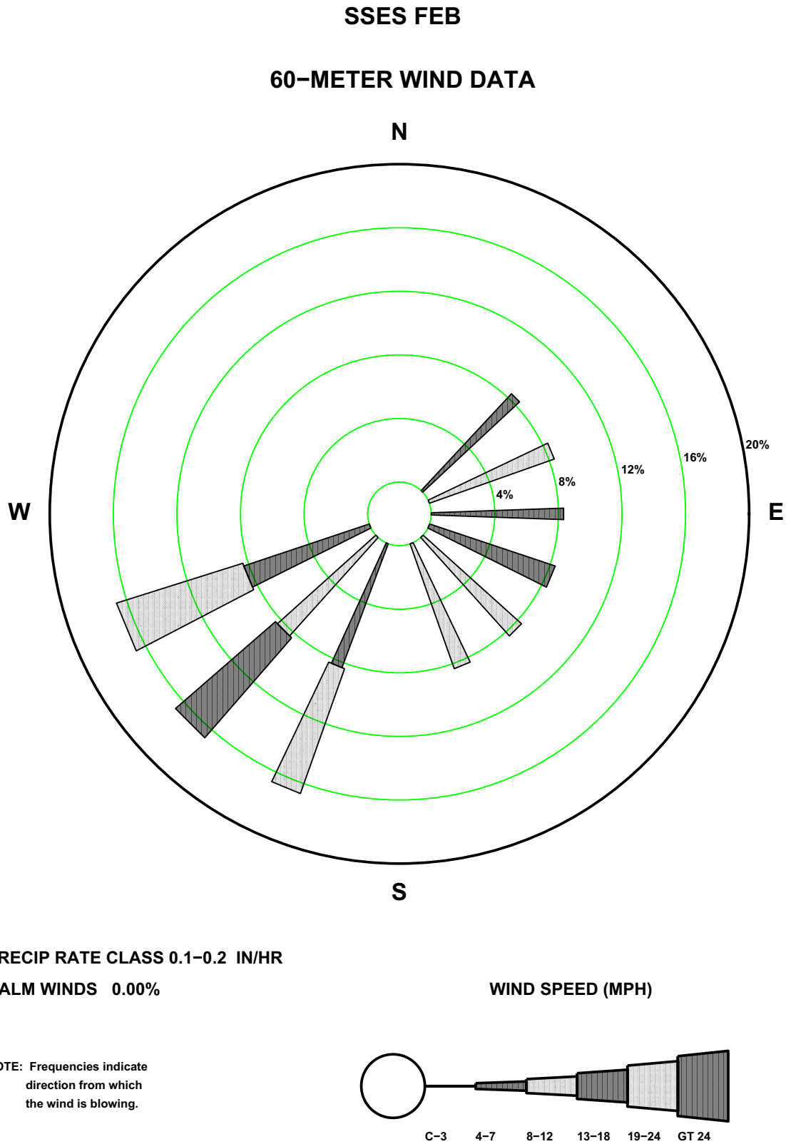
Figure 2.7-44—SSES 60 m February Precipitation Rate Wind Rose
