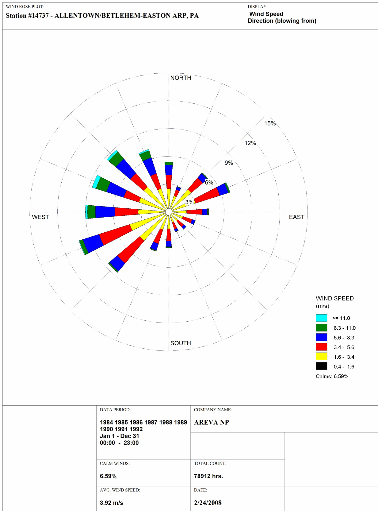
Figure 2.7-90—Allentown, PA, Wind Rose
