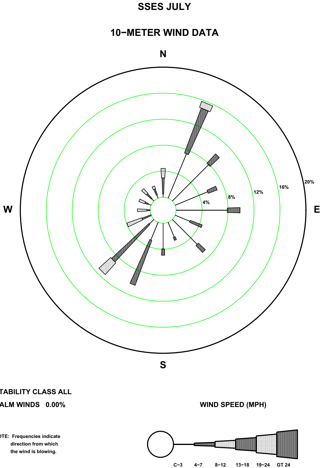
Figure 2.7-11—SSES 10 m July Precipitation Wind Rose
