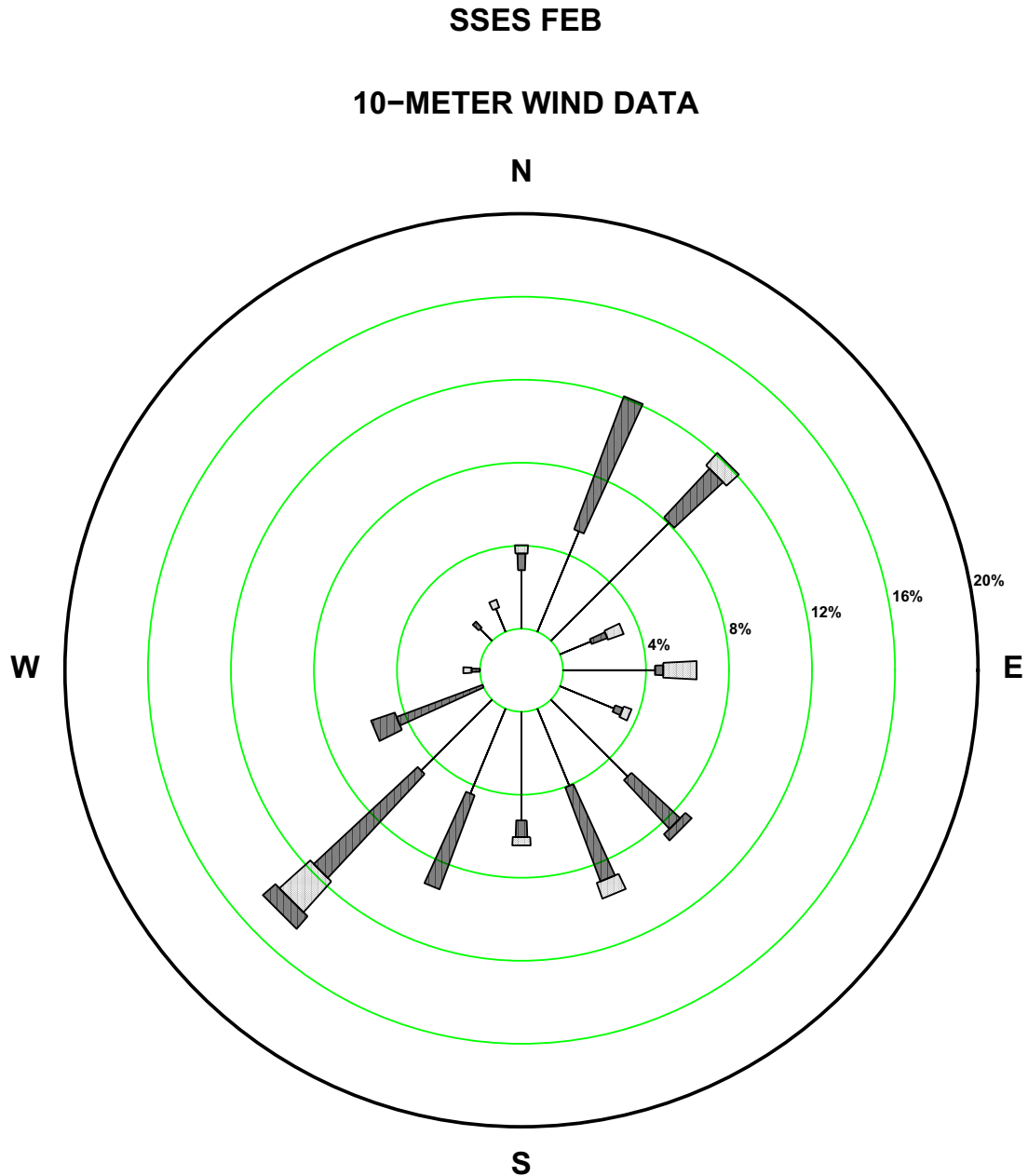
Figure 2.7-6—SSES 10 m February Precipitation Wind Rose
