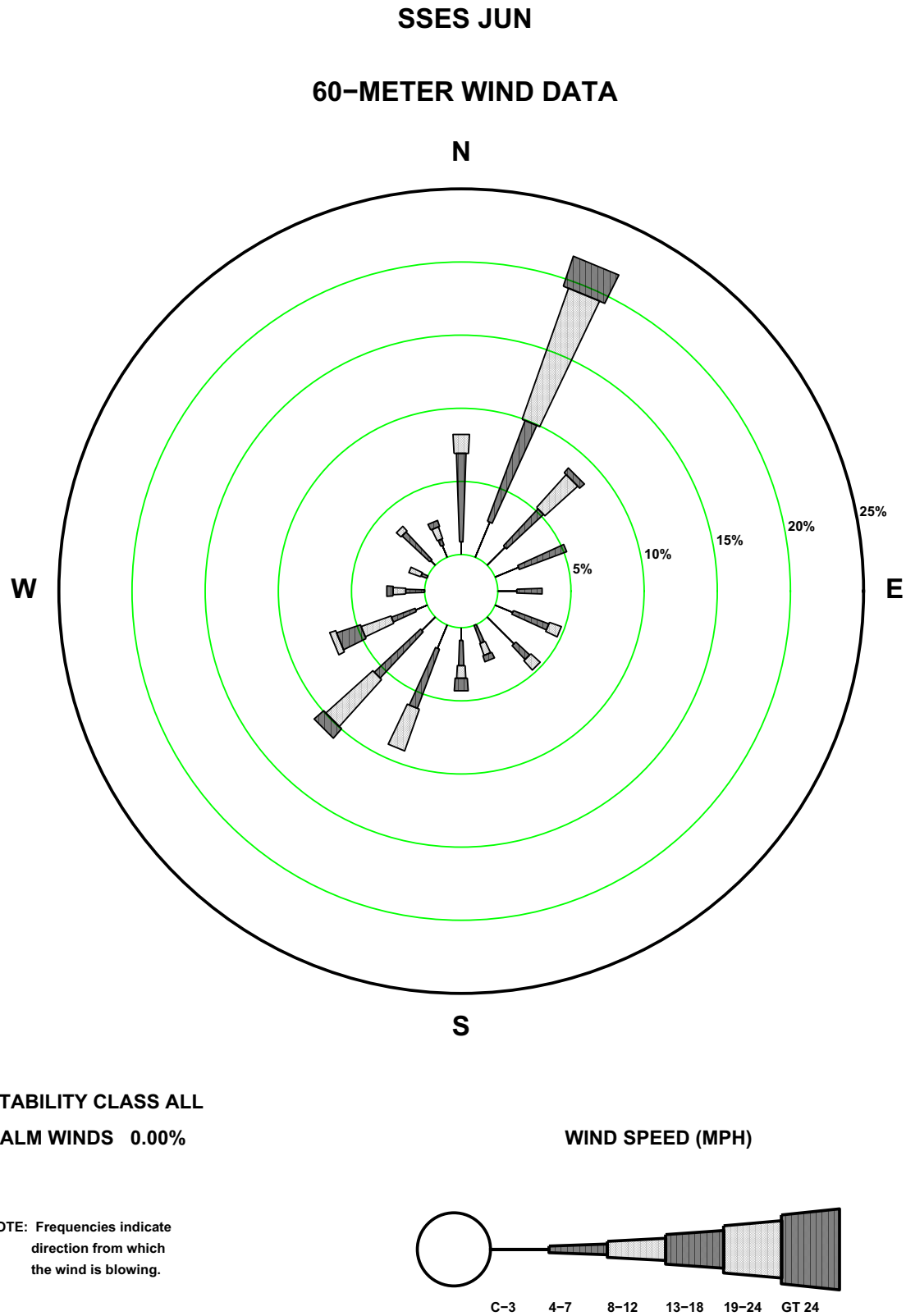
Figure 2.7-23—SSES 60 m June Precipitation Wind Rose
