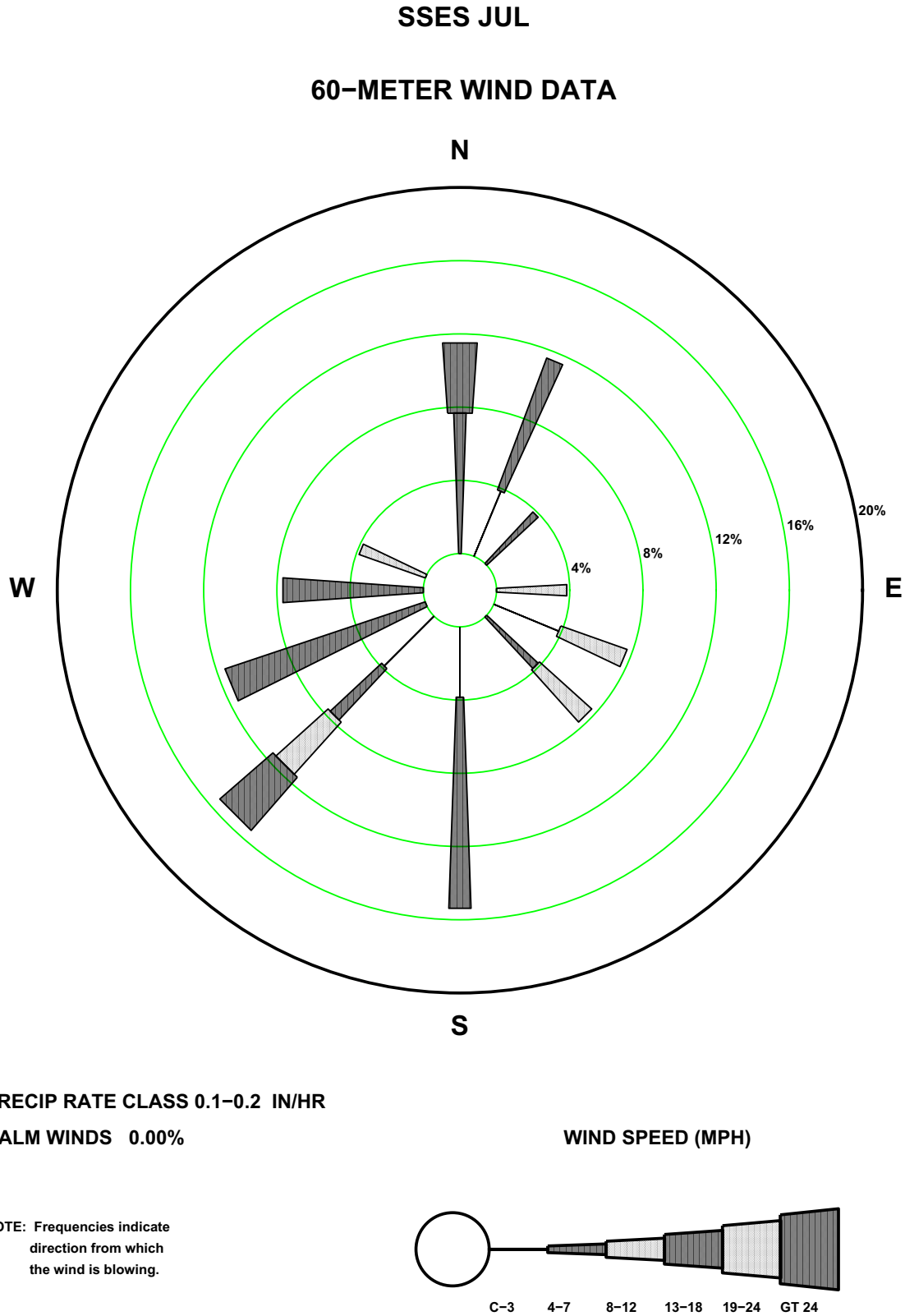
Figure 2.7-49—SSES 60 m July Precipitation Rate Wind Rose
