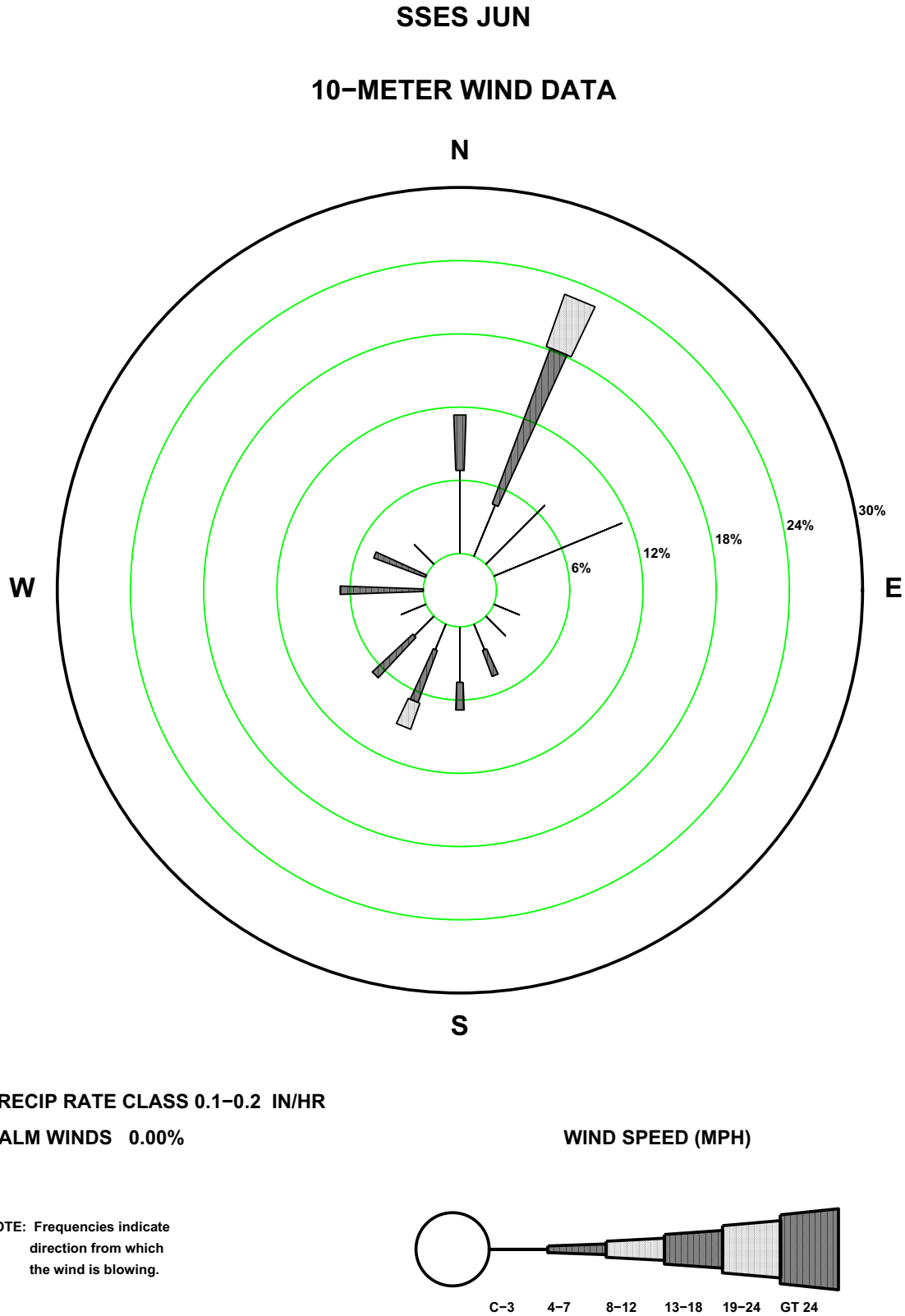
Figure 2.7-36—SSES 10 m June Precipitation Rate Wind Rose
