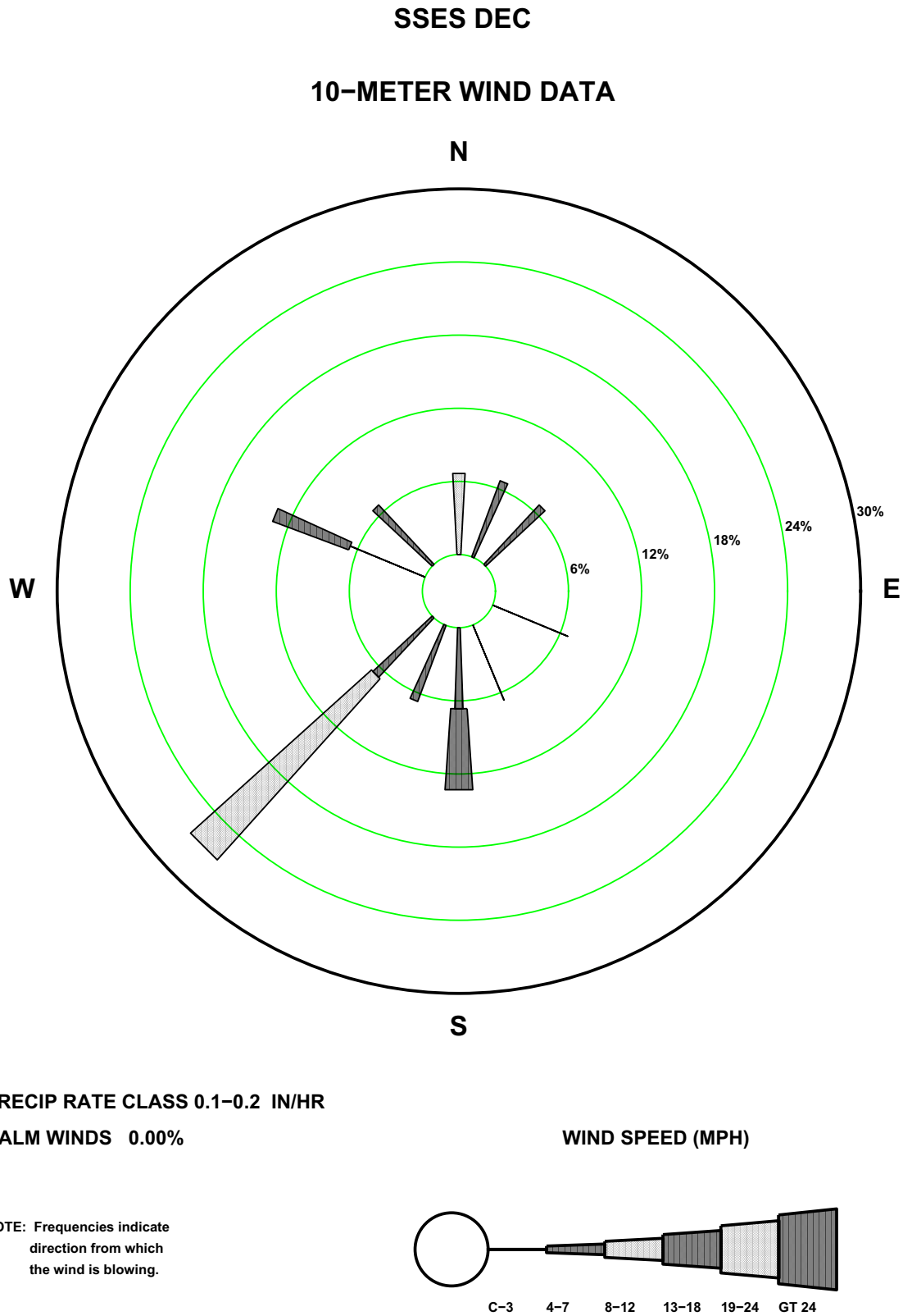
Figure 2.7-42—SSES 10 m December Precipitation Rate Wind Rose
