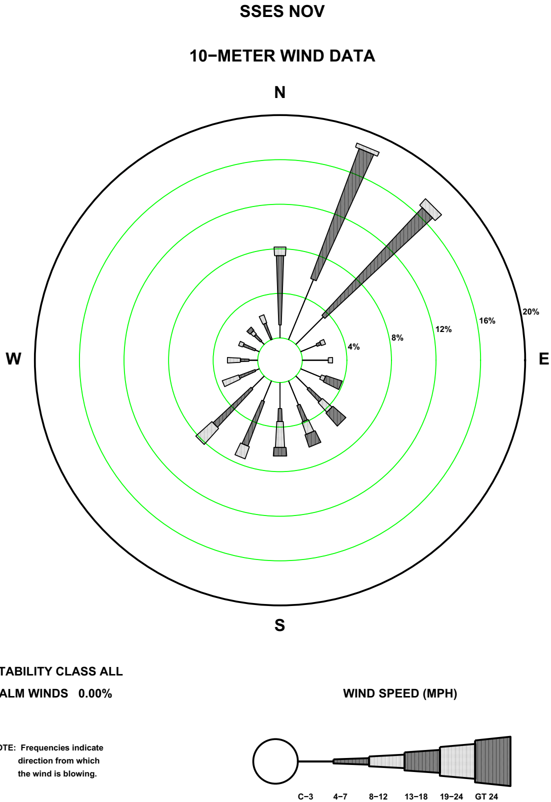
Figure 2.7-15—SSES 10 m November Precipitation Wind Rose
