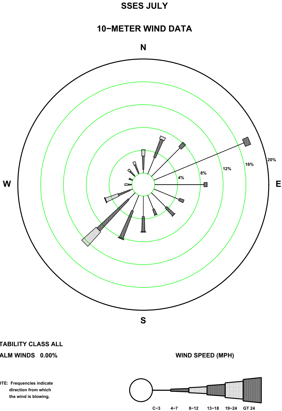
Figure 2.7-66—SSES 10m July Wind Rose
