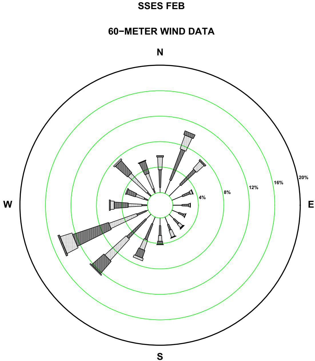
Figure 2.7-78—SSES 60m February Wind Rose
