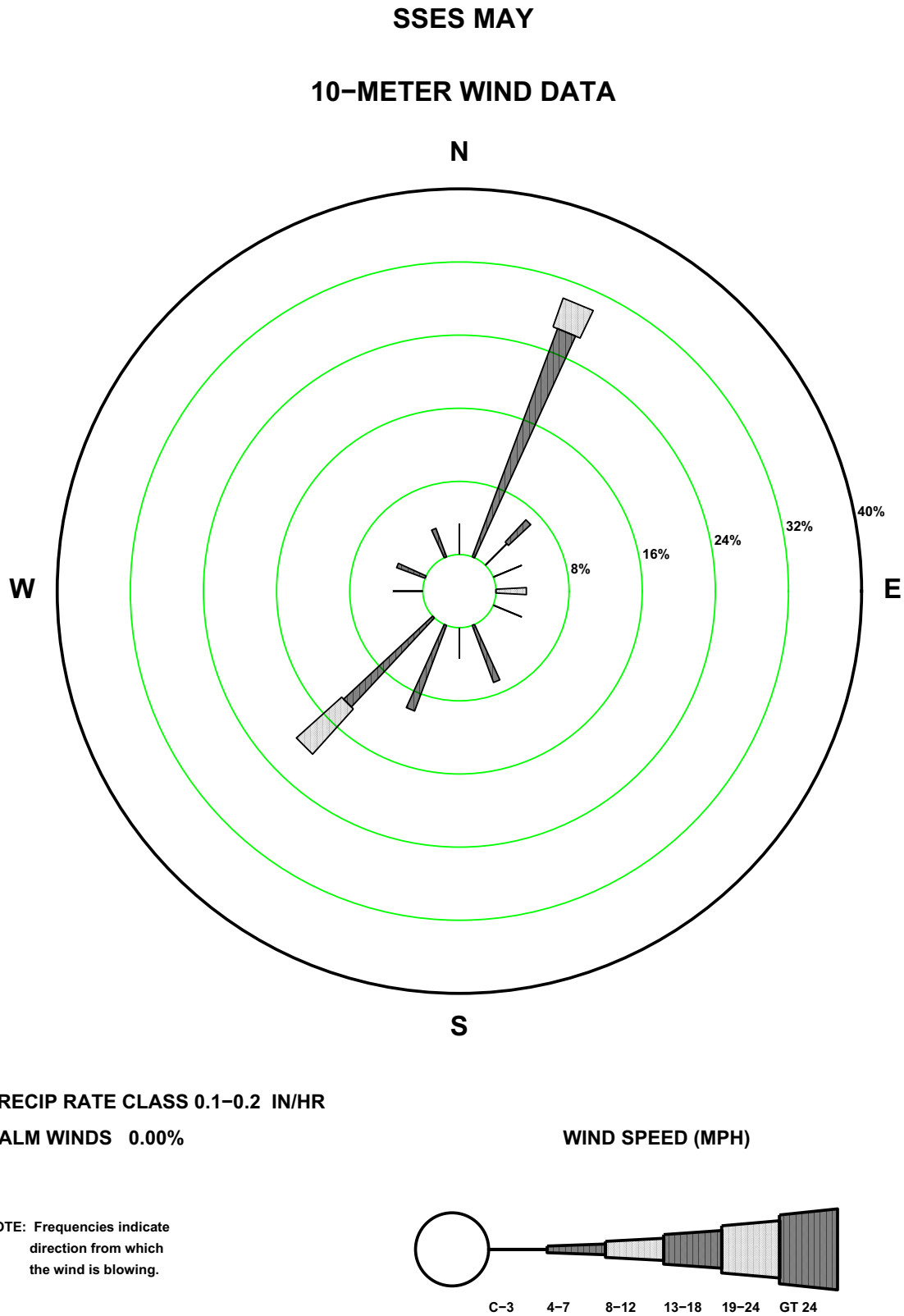
Figure 2.7-35—SSES 10 m May Precipitation Rate Wind Rose
