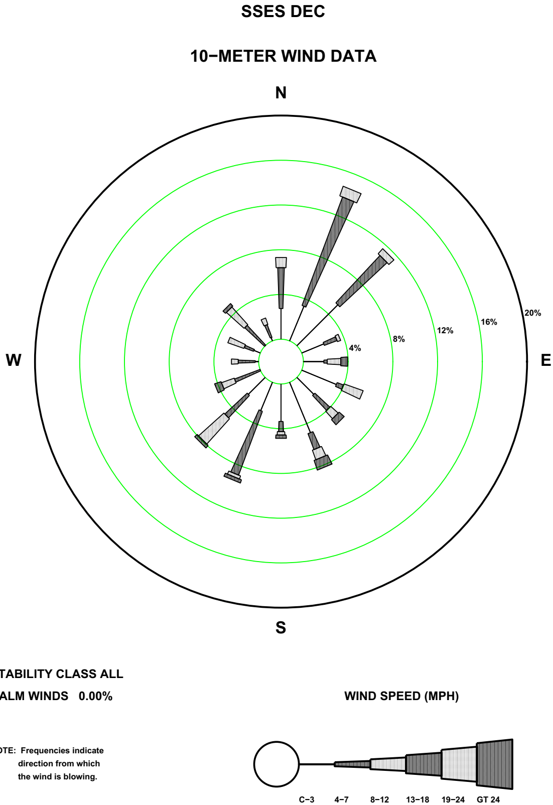
Figure 2.7-16—SSES 10 m December Precipitation Wind Rose
