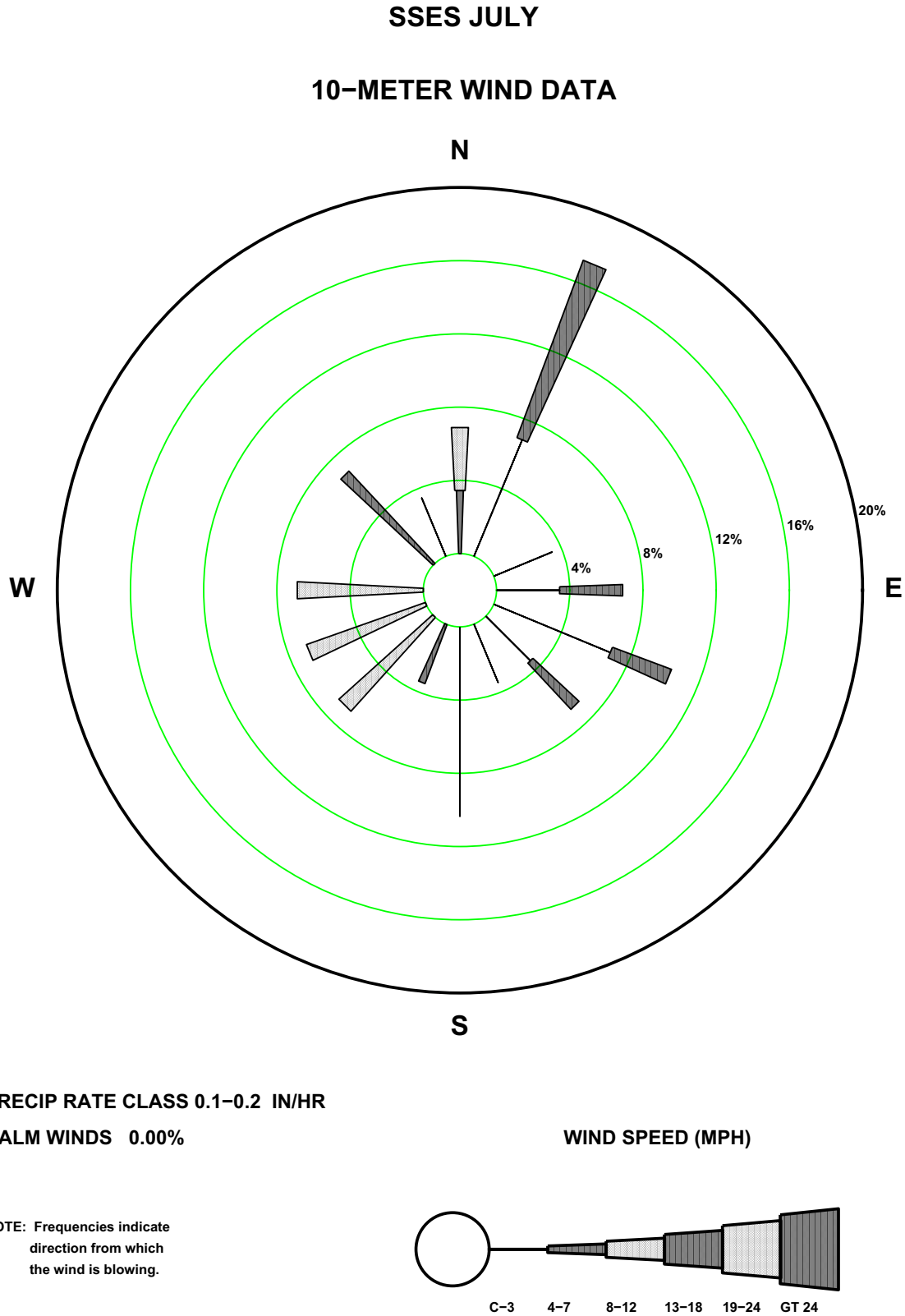
Figure 2.7-37—SSES 10 m July Precipitation Rate Wind Rose
