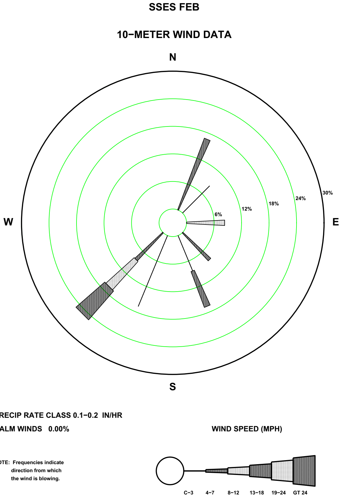
Figure 2.7-32—SSES 10 m February Precipitation Rate Wind Rose
