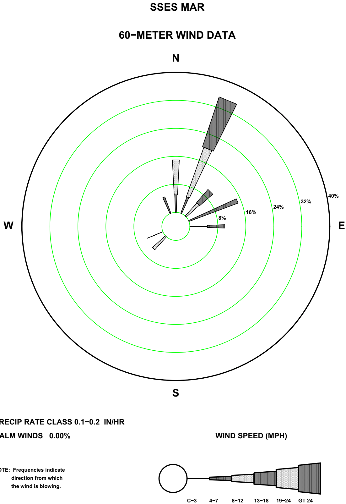
Figure 2.7-45—SSES 60 m March Precipitation Rate Wind Rose
