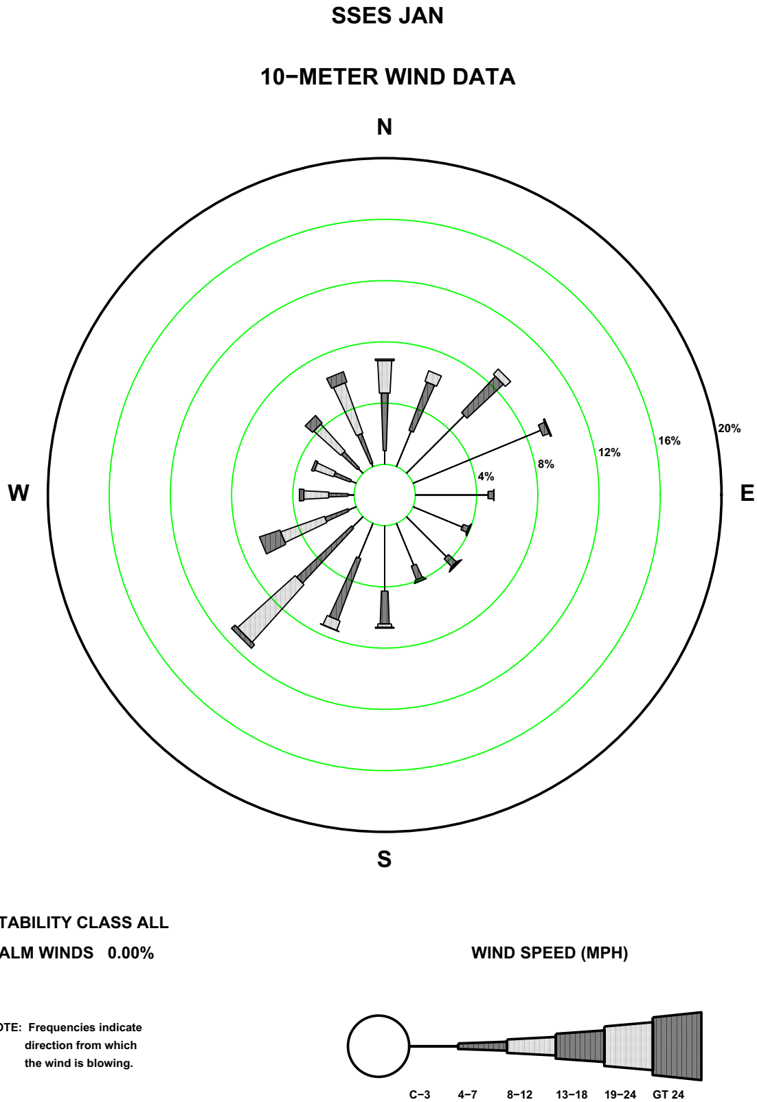
Figure 2.7-60—SSES 10m January Wind Rose
