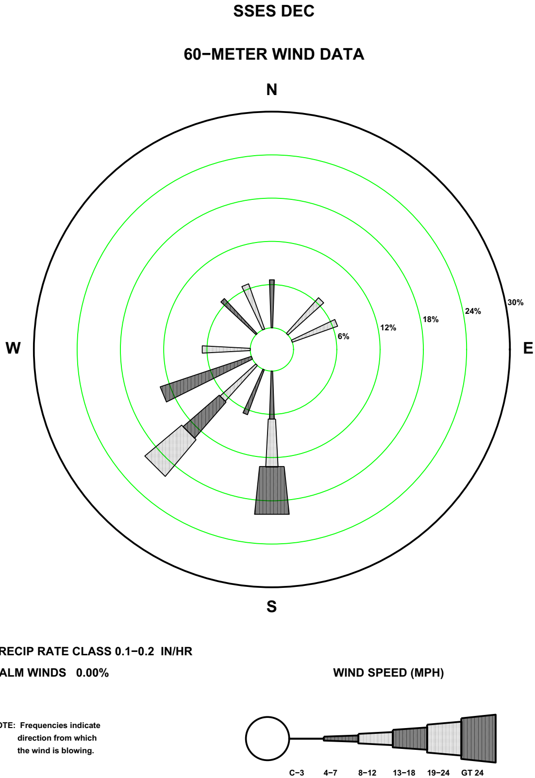
Figure 2.7-54—SSES 60 m December Precipitation Rate Wind Rose
