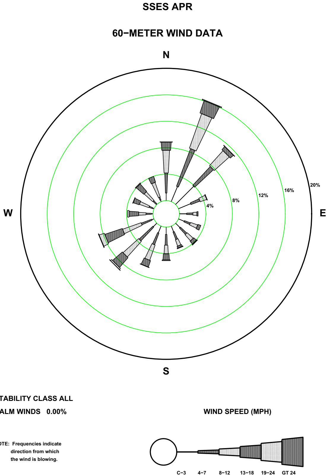
Figure 2.7-80—SSES 60m April Wind Rose
