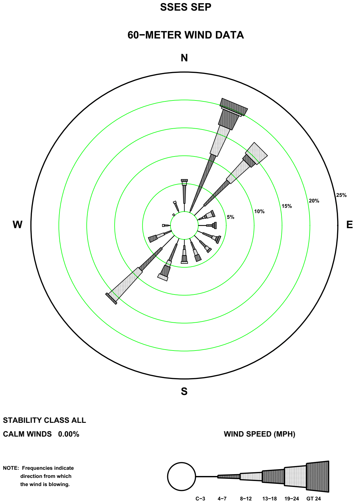
Figure 2.7-26—SSES 60 m September Precipitation Wind Rose
