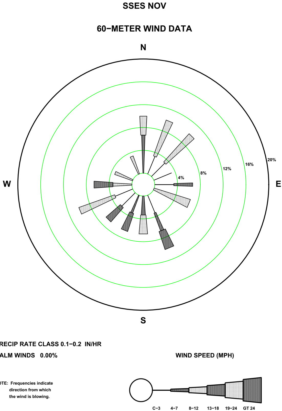
Figure 2.7-53—SSES 60 m November Precipitation Rate Wind Rose
