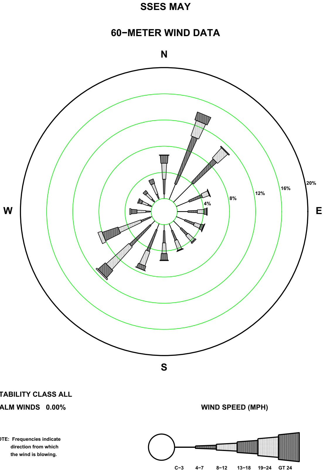
Figure 2.7-81—SSES 60m May Wind Rose
