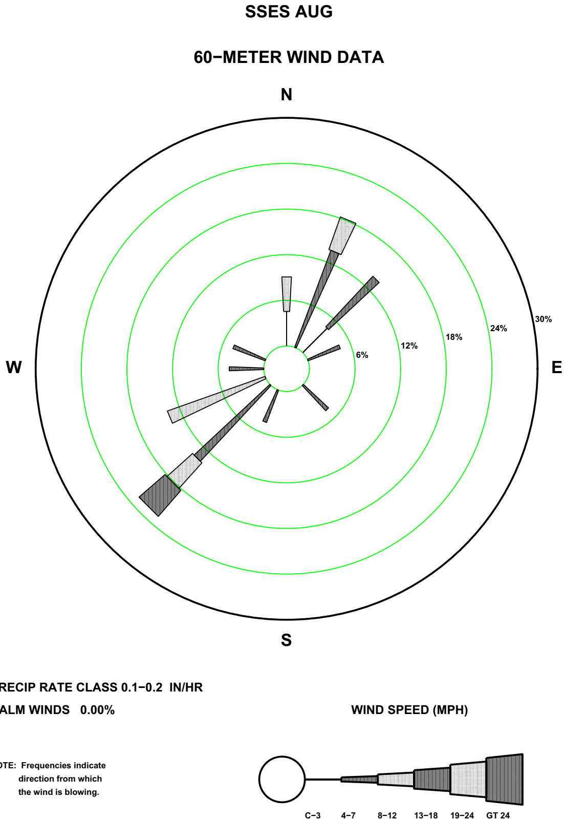
Figure 2.7-50—SSES 60 m August Precipitation Rate Wind Rose
