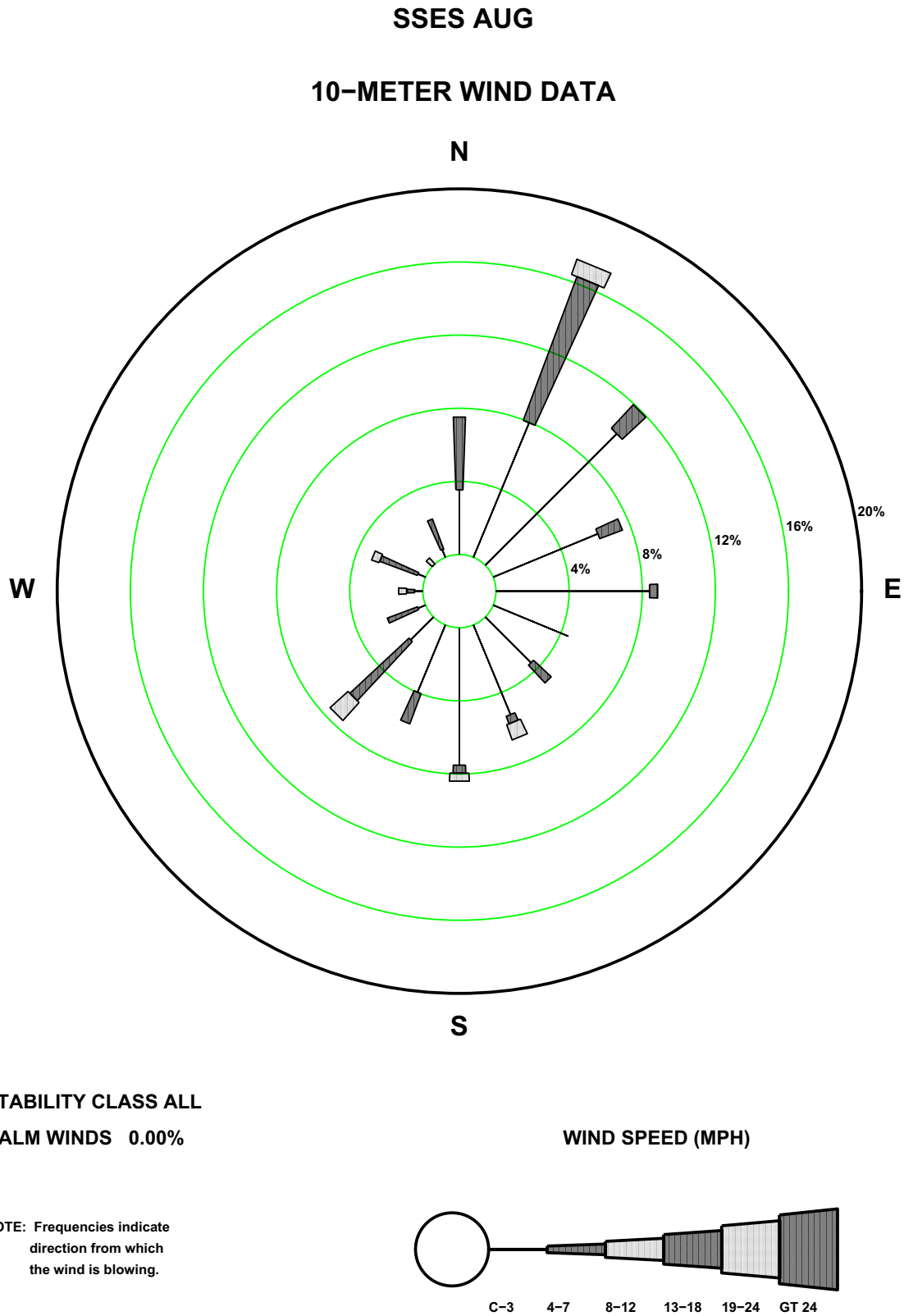
Figure 2.7-12—SSES 10 m August Precipitation Wind Rose
