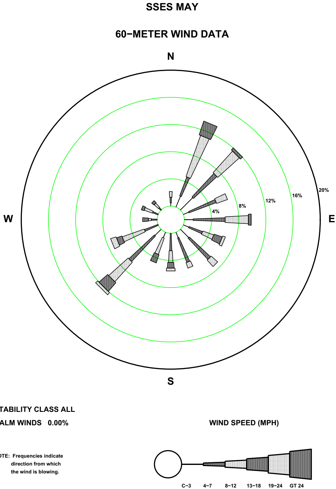
Figure 2.7-22—SSES 60 m May Precipitation Wind Rose
