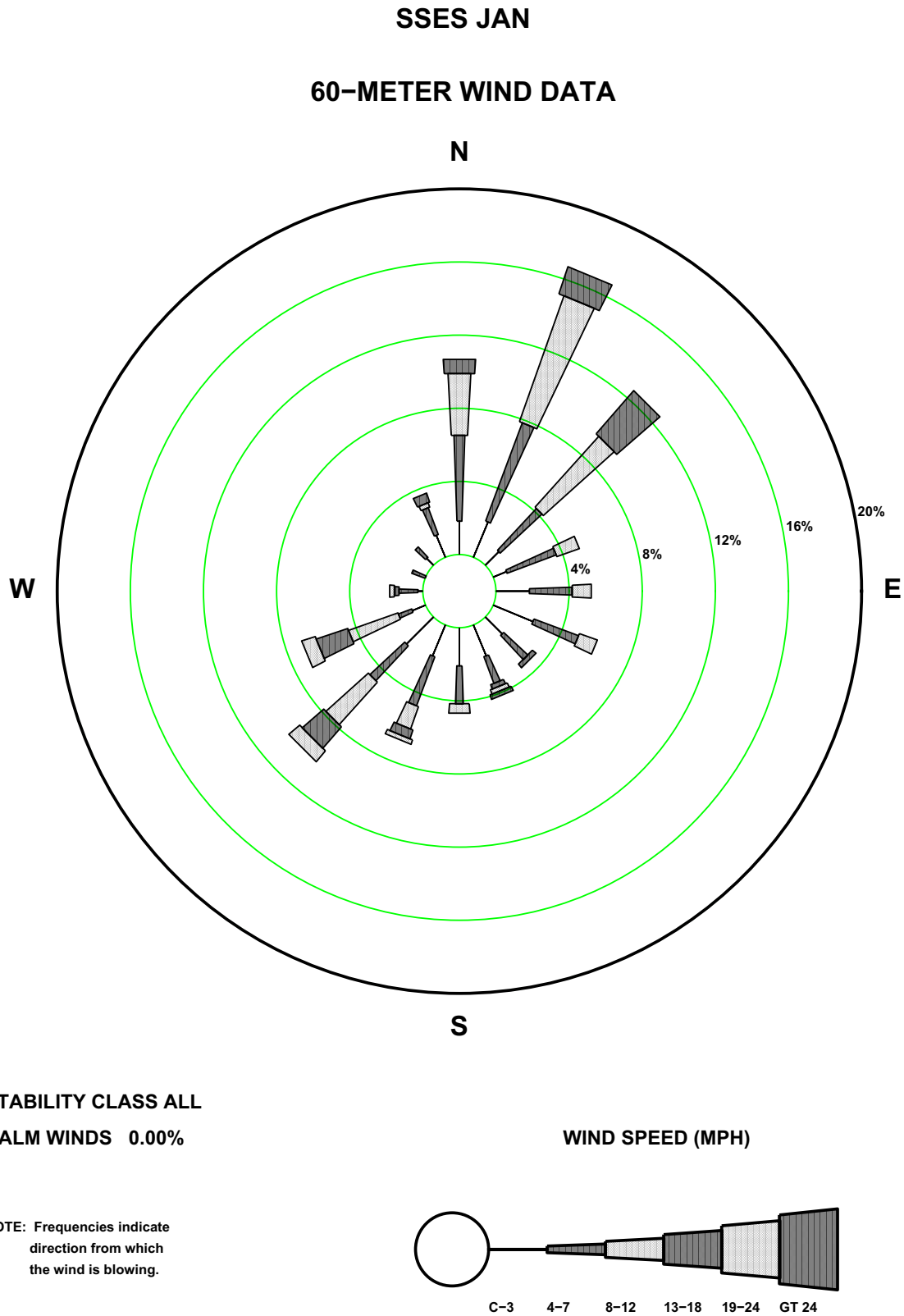
Figure 2.7-18—SSES 60 m January Precipitation Wind Rose
