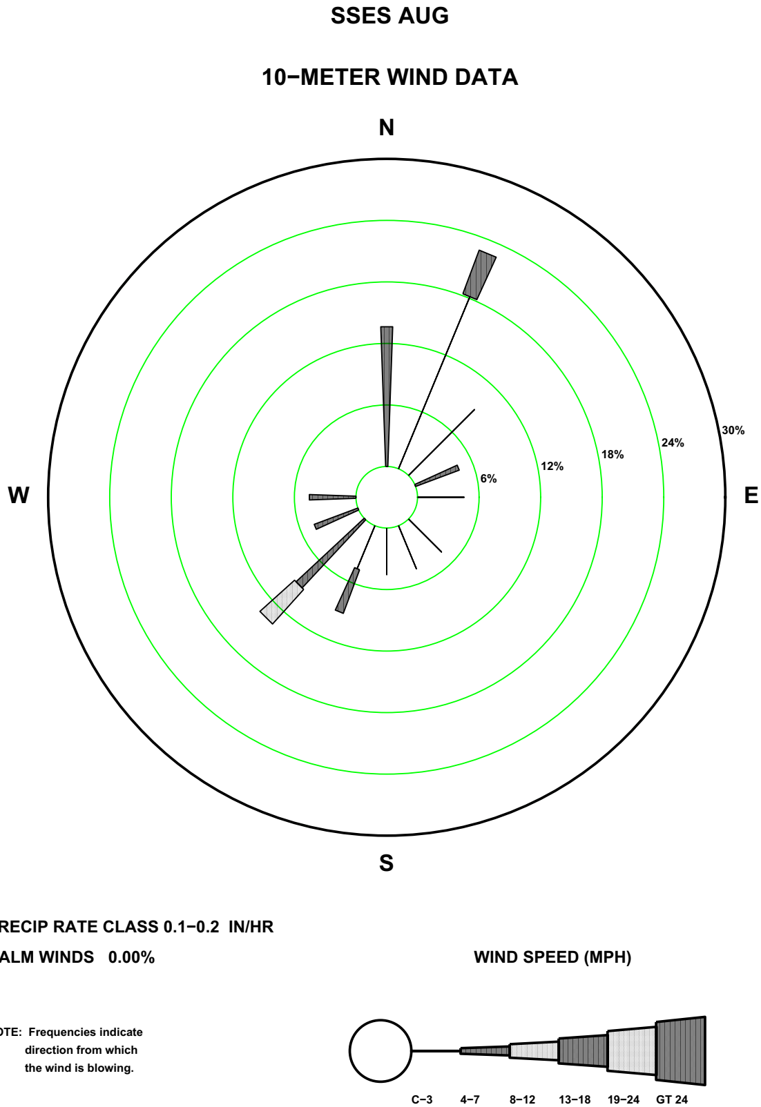
Figure 2.7-38—SSES 10 m August Precipitation Rate Wind Rose
