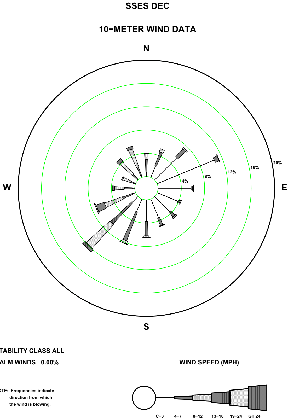
Figure 2.7-71—SSES 10m December Wind Rose
