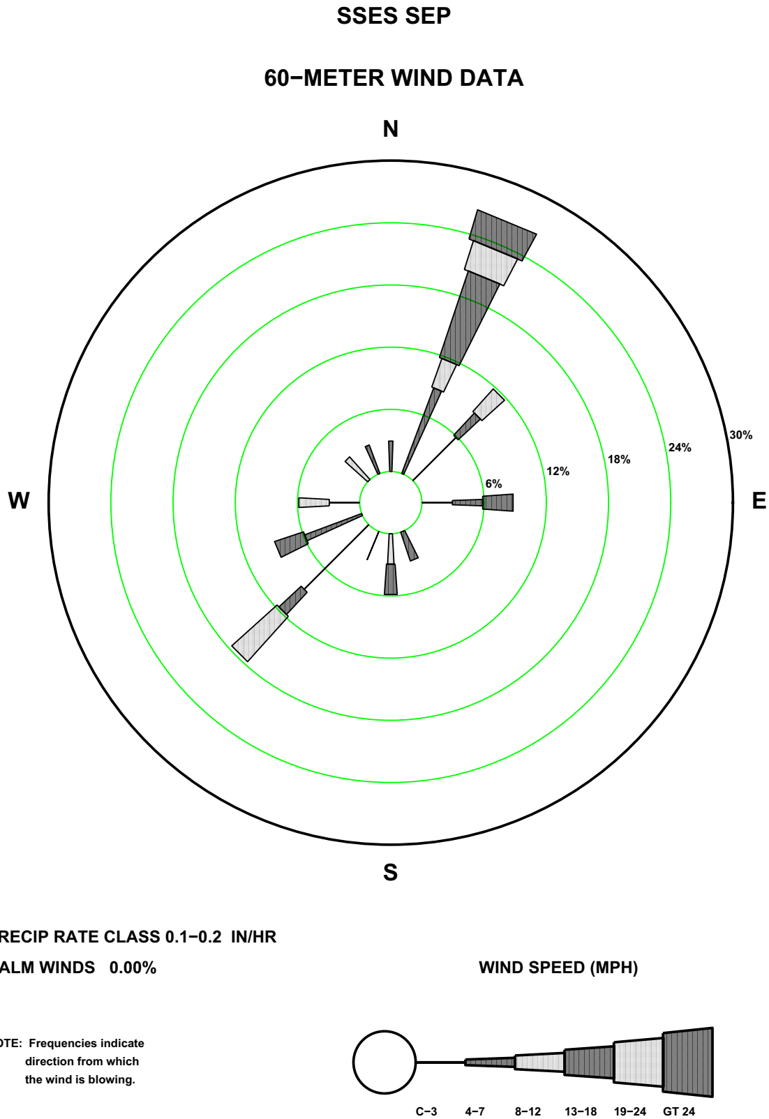
Figure 2.7-51—SSES 60 m September Precipitation Rate Wind Rose
