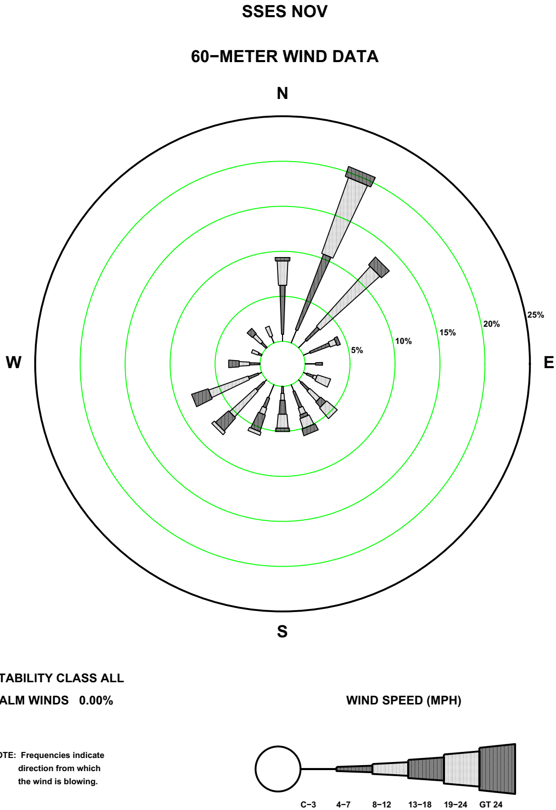
Figure 2.7-28—SSES 60 m November Precipitation Wind Rose
