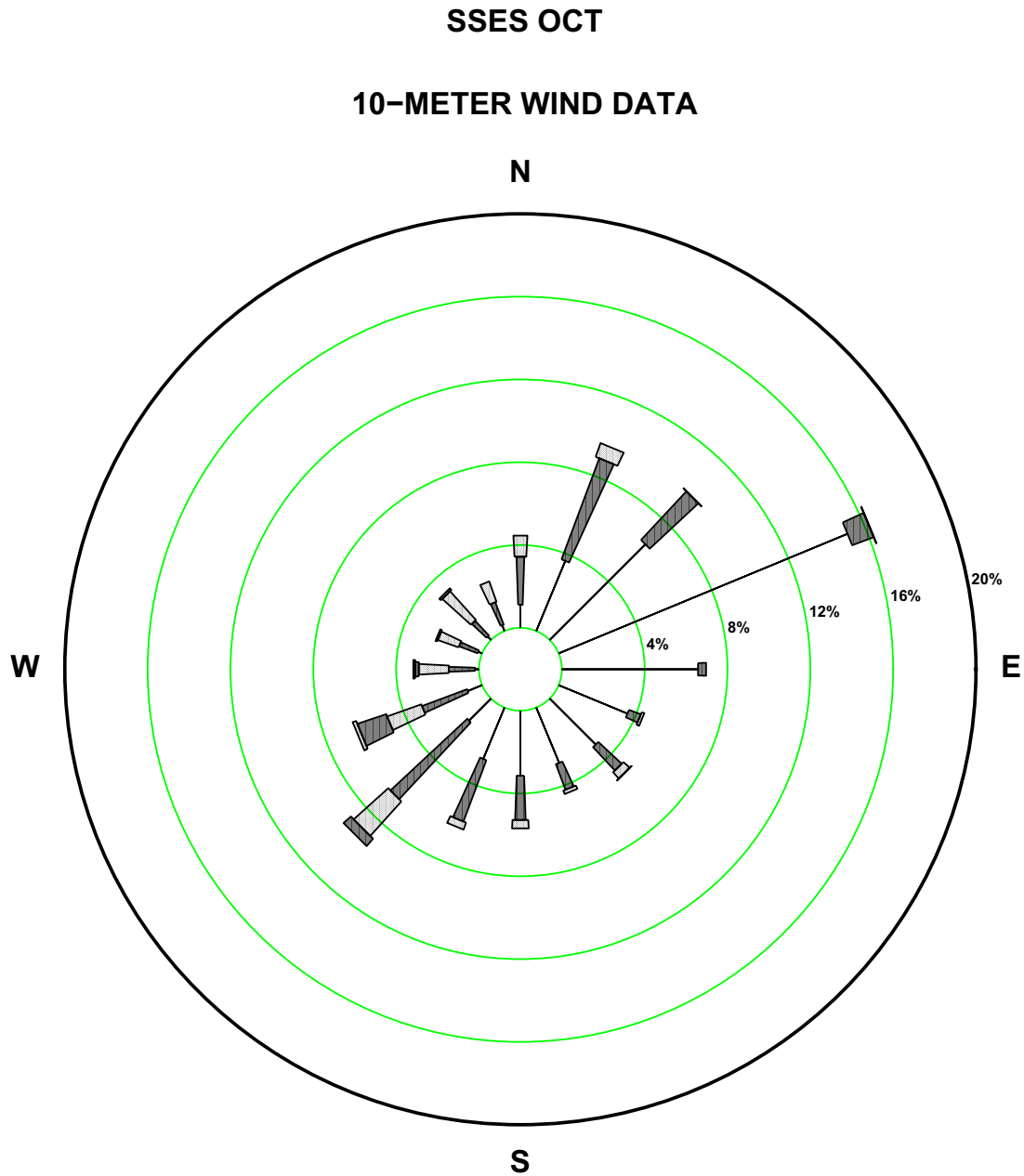
Figure 2.7-69—SSES 10m October Wind Rose
