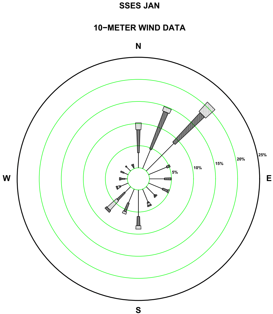
Figure 2.7-5—SSES 10 m January Precipitation Wind Rose
