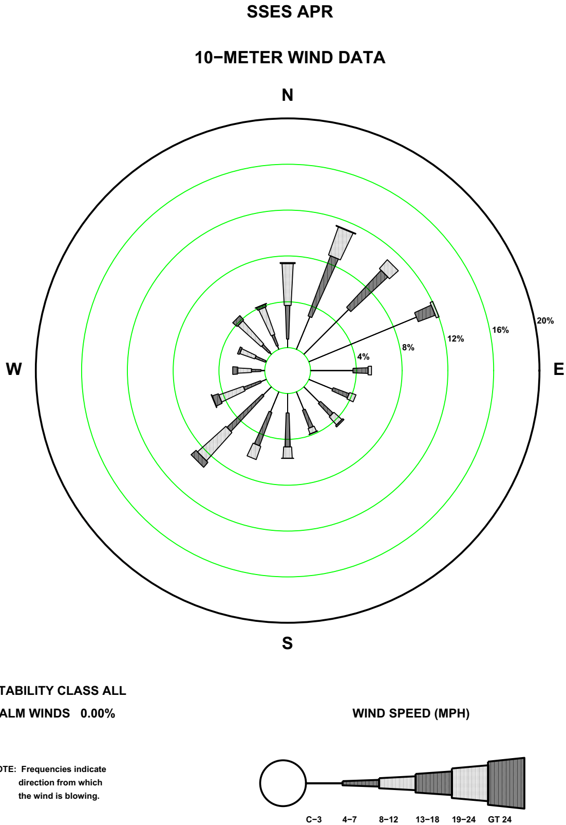
Figure 2.7-63—SSES 10m April Wind Rose
