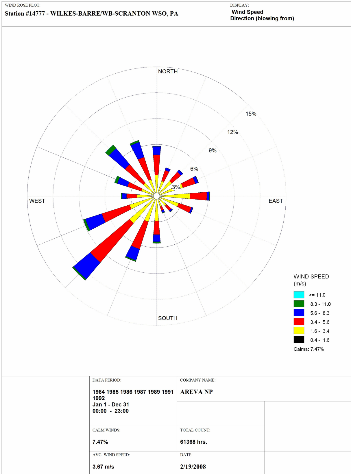
Figure 2.7-89—Wilkes-Barre/Scranton, PA, Wind Rose
