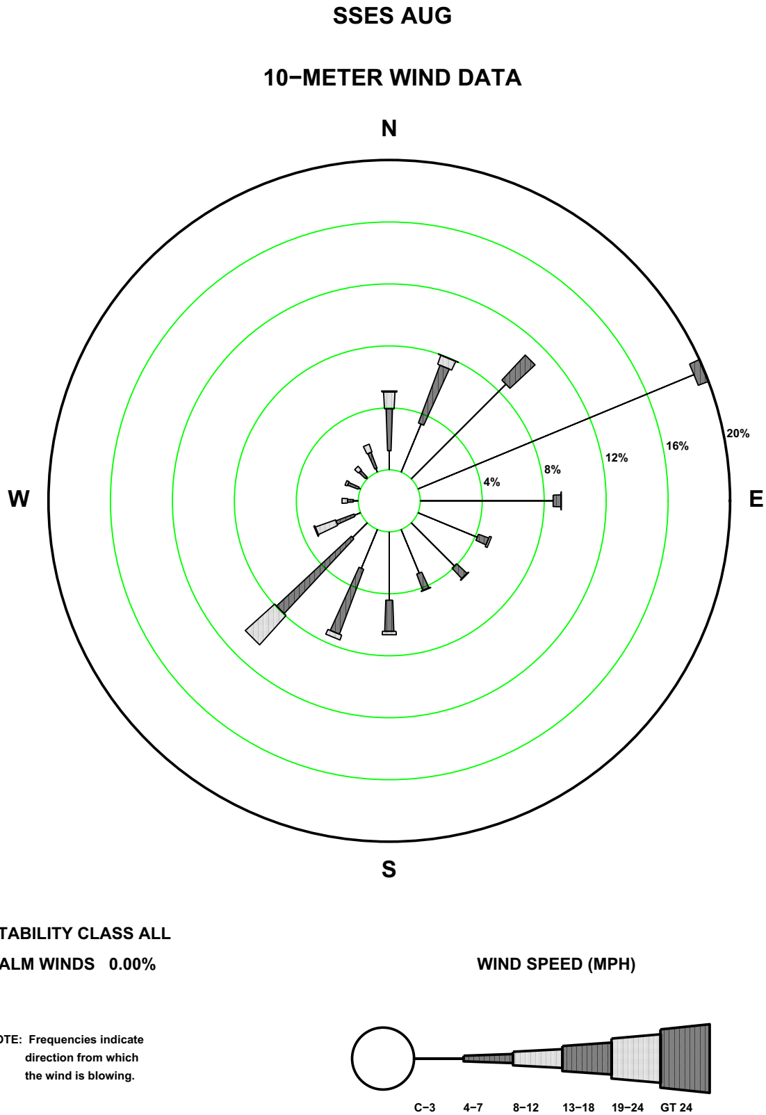
Figure 2.7-67—SSES 10m August Wind Rose
