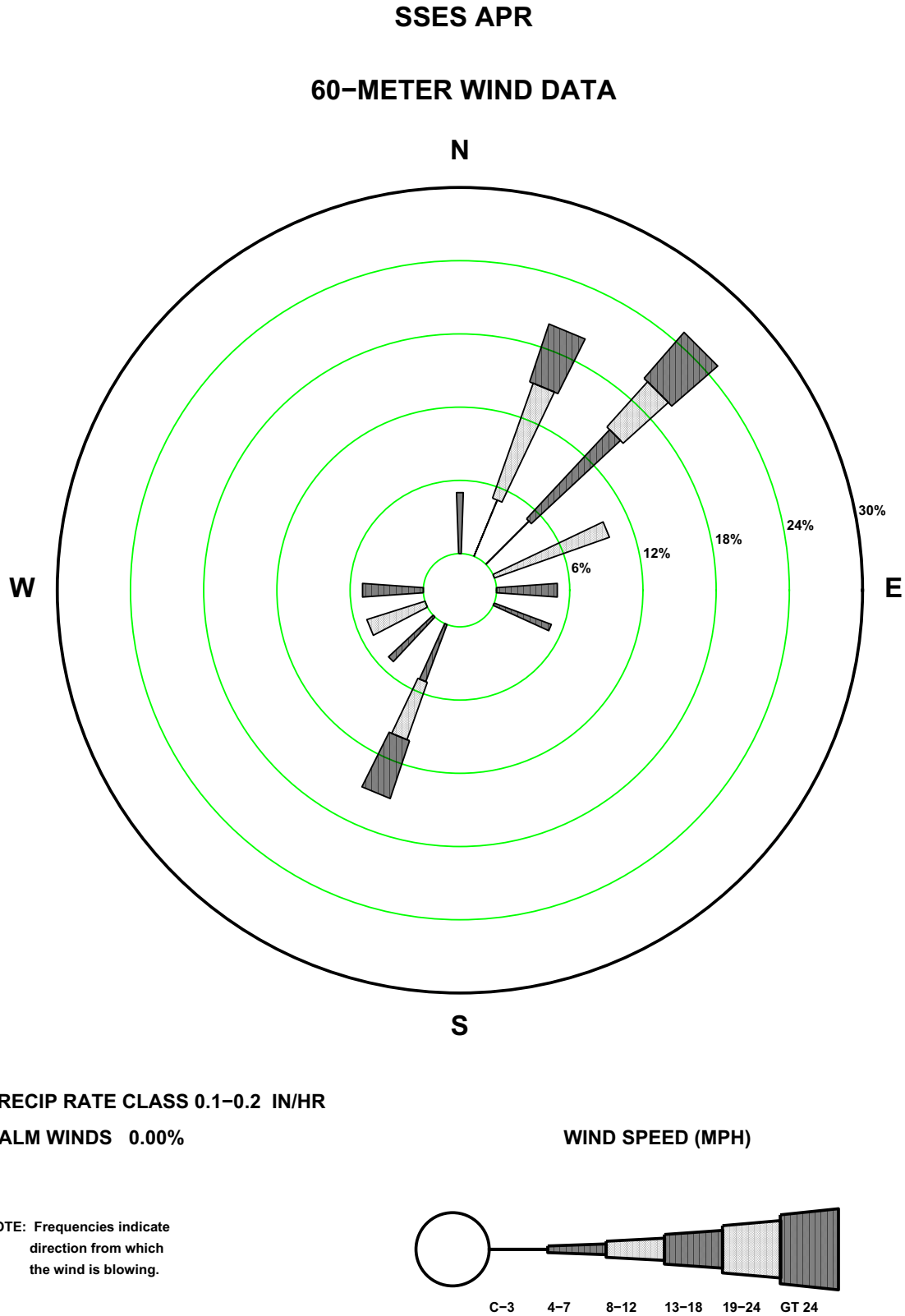
Figure 2.7-46—SSES 60 m April Precipitation Rate Wind Rose
