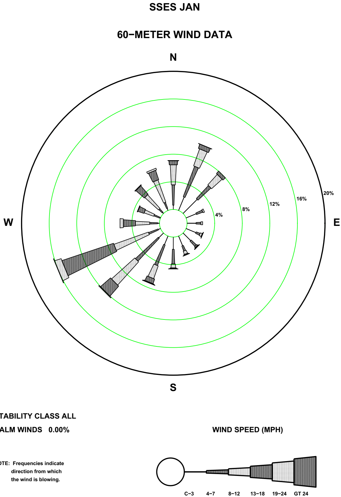
Figure 2.7-77—SSES 60m January Wind Rose
