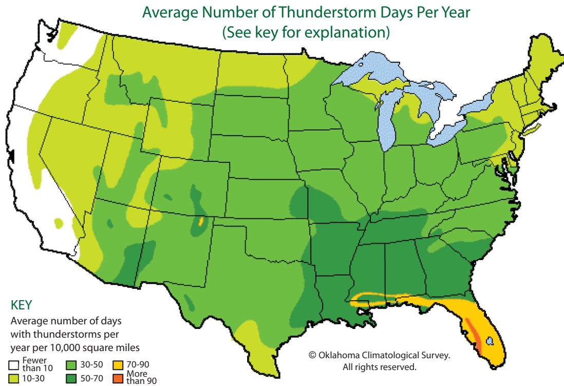
Figure 2.7-3—Annual Thunderstorm Frequency
