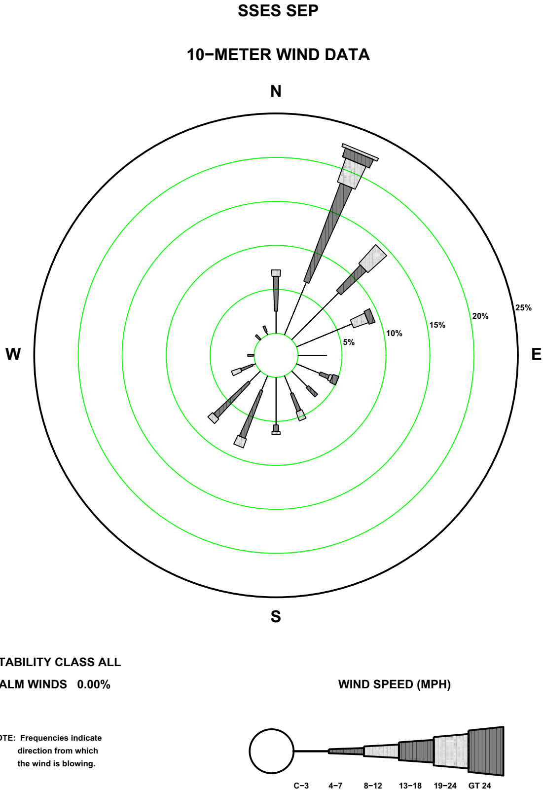
Figure 2.7-13—SSES 10 m September Precipitation Wind Rose
