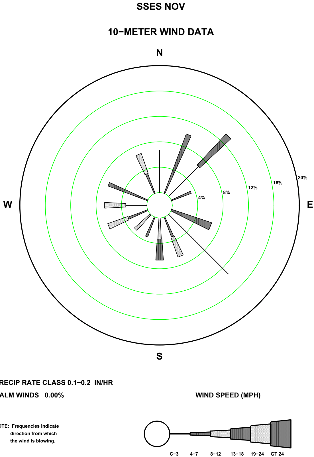
Figure 2.7-41—SSES 10 m November Precipitation Rate Wind Rose
