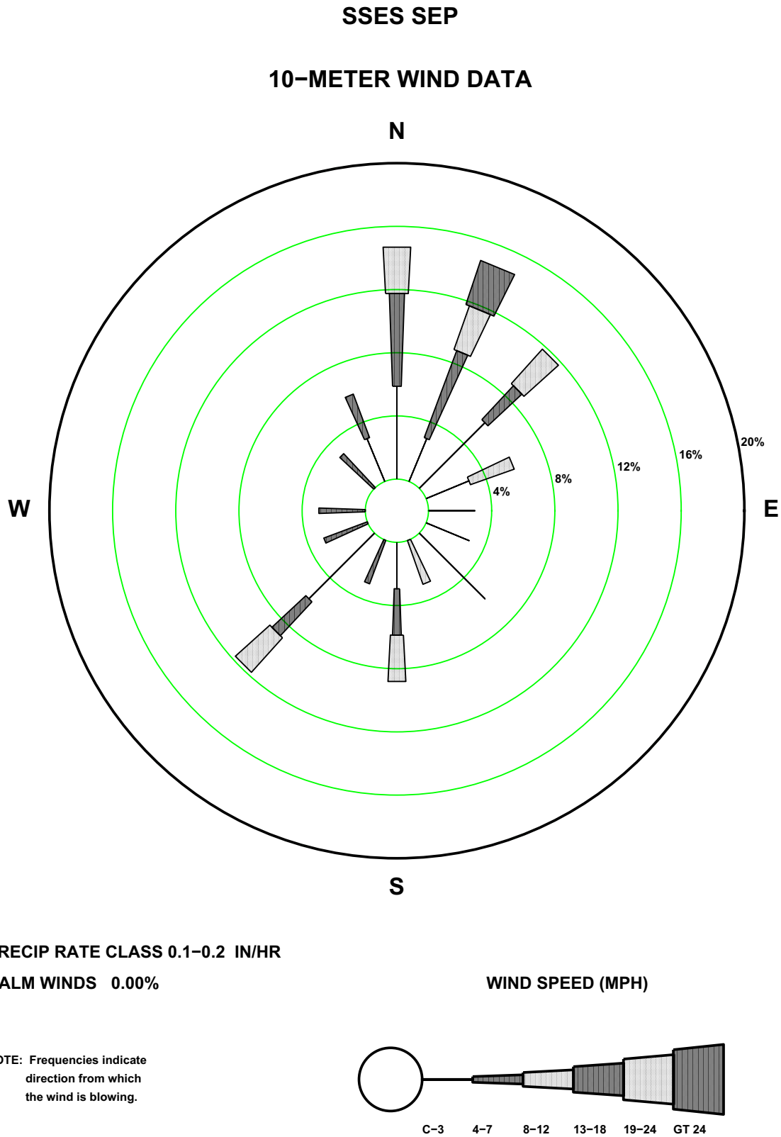
Figure 2.7-39—SSES 10 m September Precipitation Rate Wind Rose
