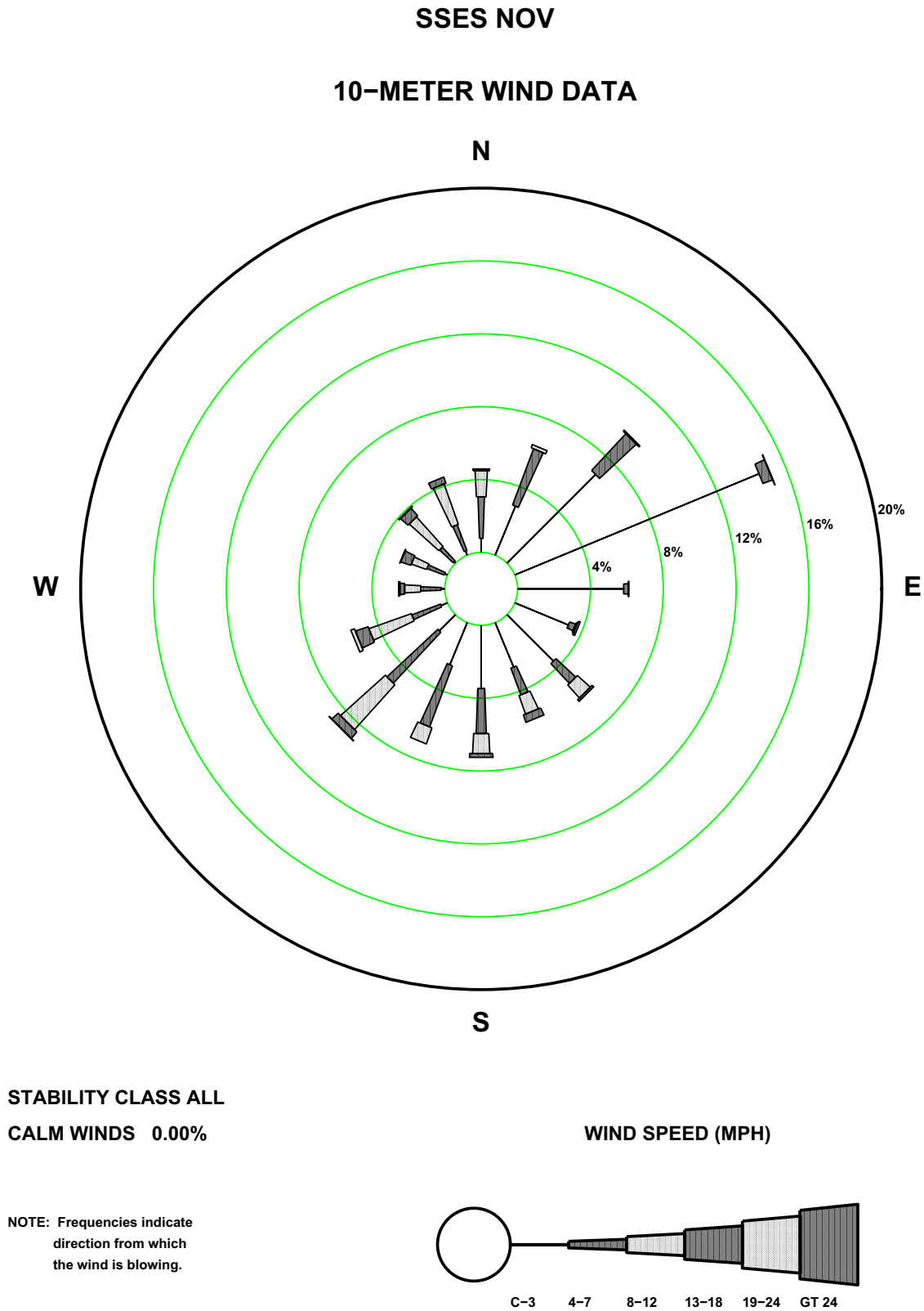
Figure 2.7-70—SSES 10m November Wind Rose
