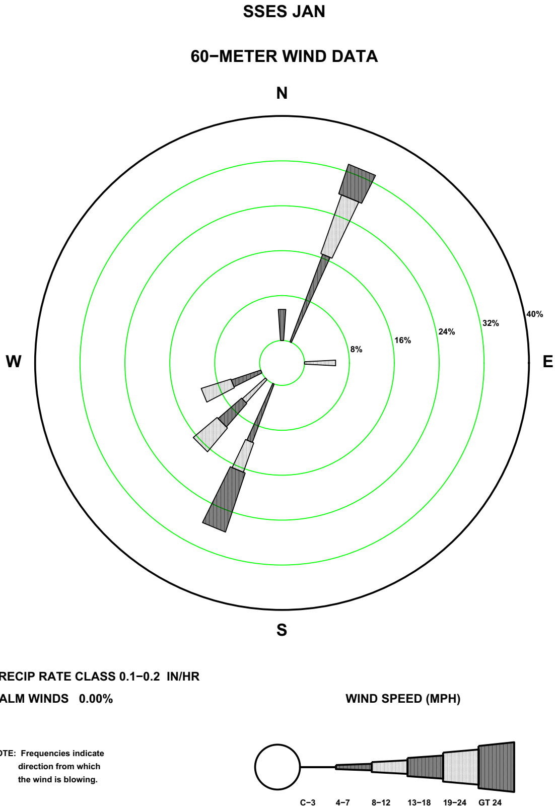
Figure 2.7-43—SSES 60 m January Precipitation Rate Wind Rose
