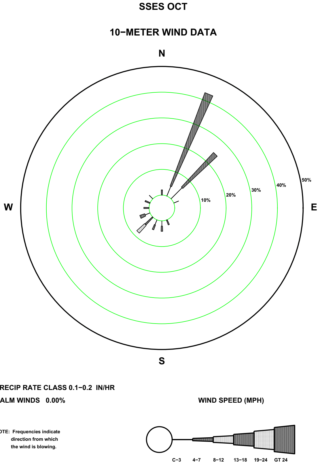
Figure 2.7-40—SSES 10 m October Precipitation Rate Wind Rose
