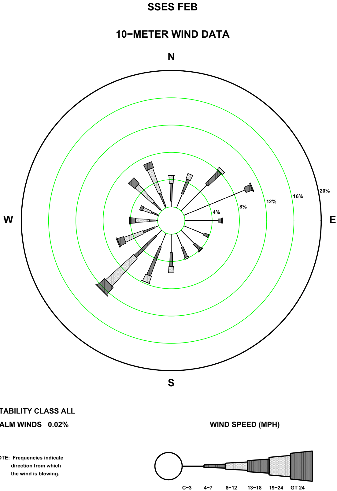
Figure 2.7-61—SSES 10m February Wind Rose
