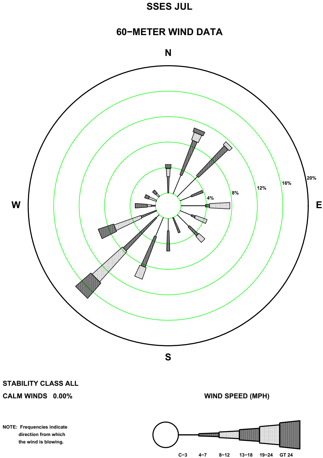
Figure 2.7-24—SSES 60 m July Precipitation Wind Rose
