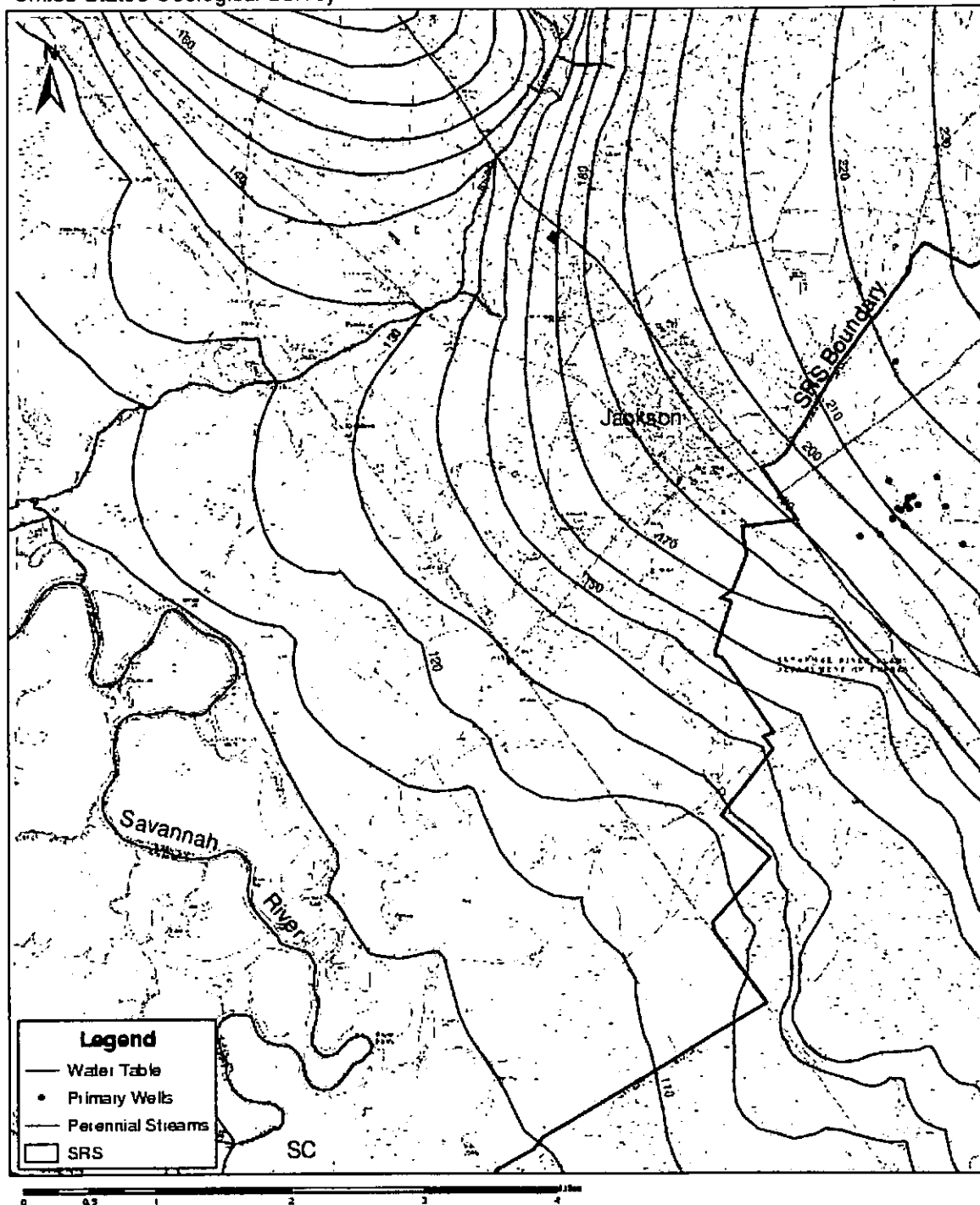
Figure 10. Water Table Configuration on the Jackson 7.5 Minute Quadrangle
