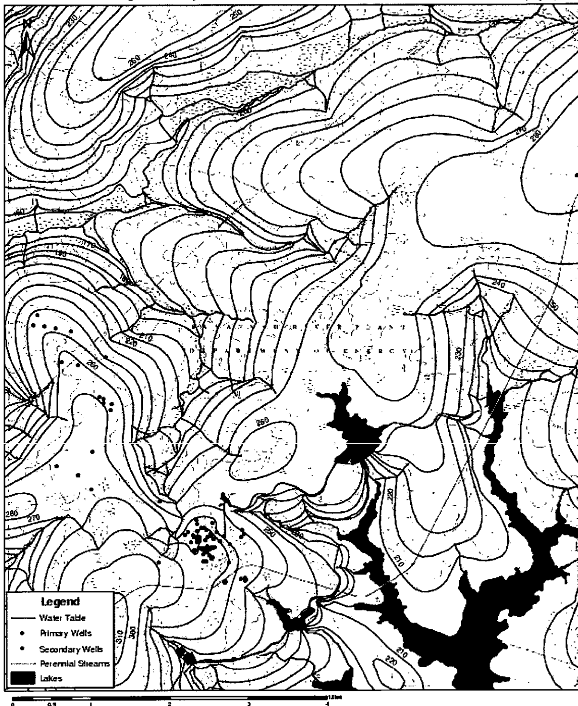
Figure 7. Water Table Configuration on the New Ellenton SE 7.5 Minute Quadrangle
