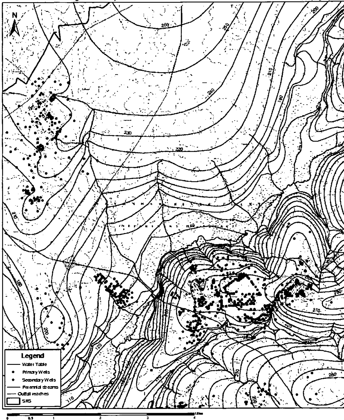
Figure 6. Water Table Configuration on the New Ellenton SW 7.5 Minute Quadrangle
