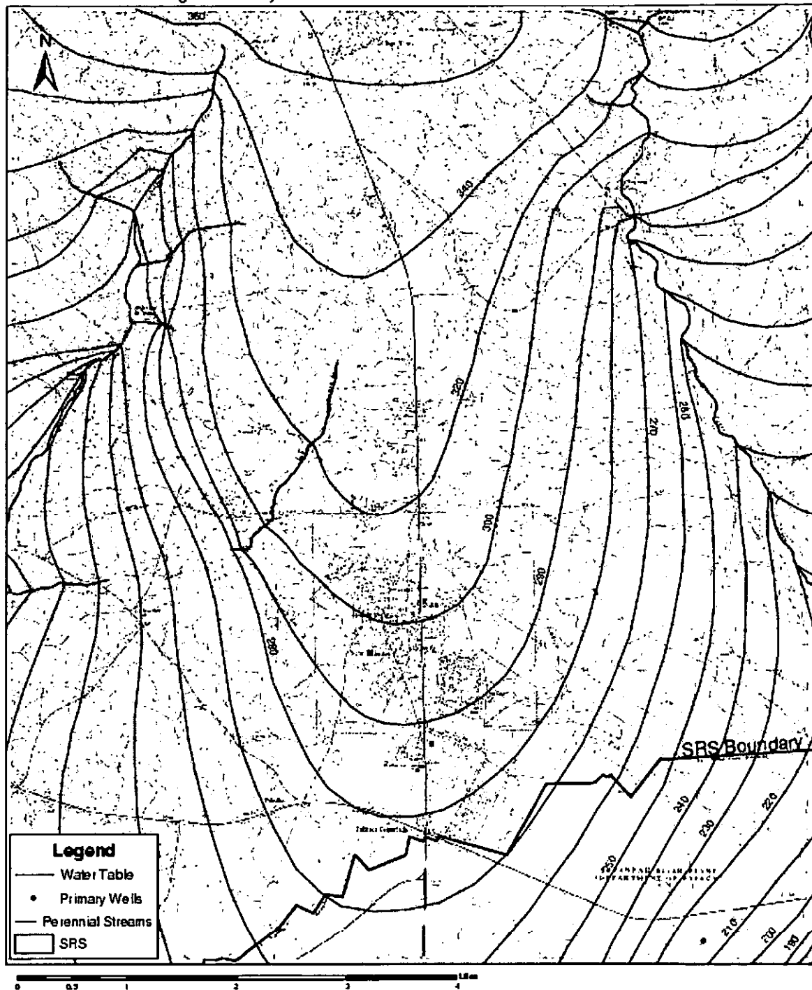
Figure 11. Water Table Configuration on the New Ellenton 7.5 Minute Quadrangle
