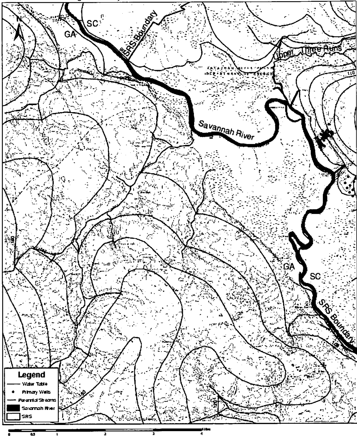
Figure 15. Water Table Configuration on the Shell Bluff Landing 7.5 Minute Quadrangle
