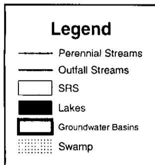
Figure 2. SRS Streams and Groundwater Basins
