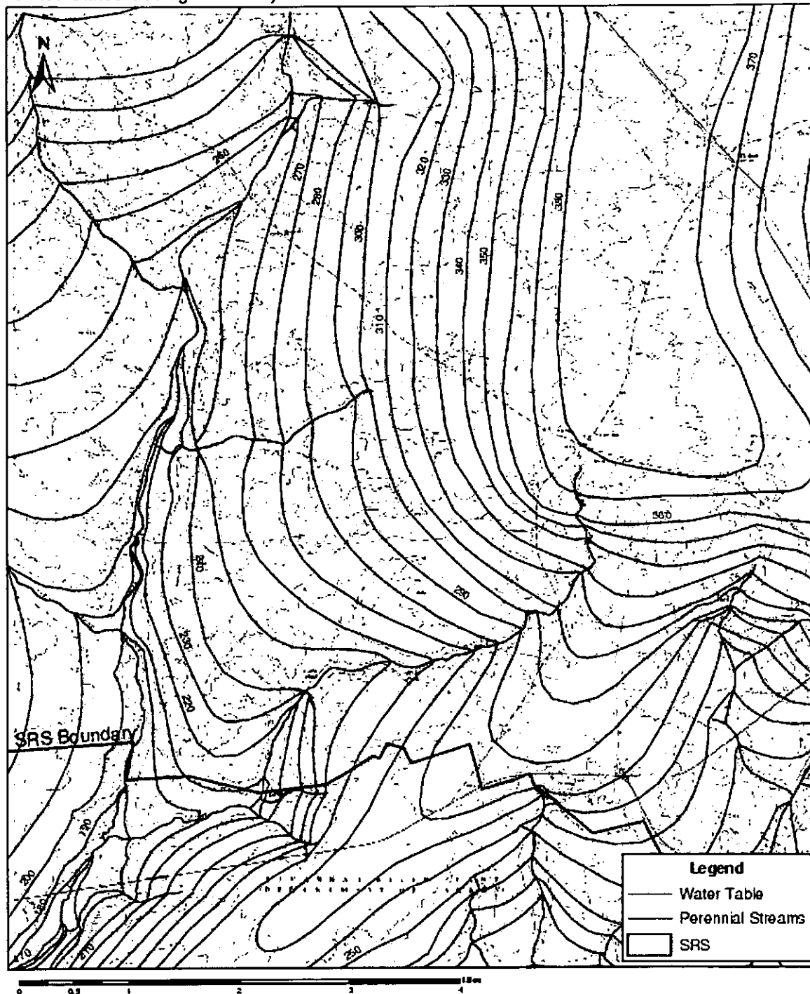
Figure 12. Water Table Configuration on the Windsor 7.5 Minute Quadrangle
