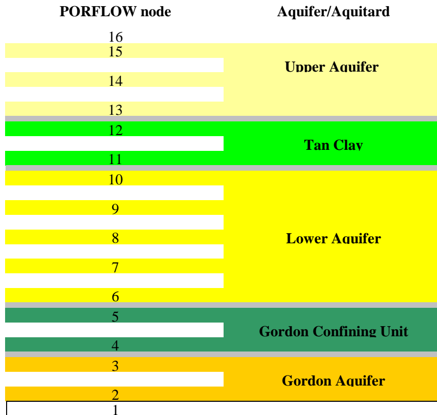
Figure 4-3. Schematic of the Aquifer/Aquitard System Model (Cook et al., 2005)
