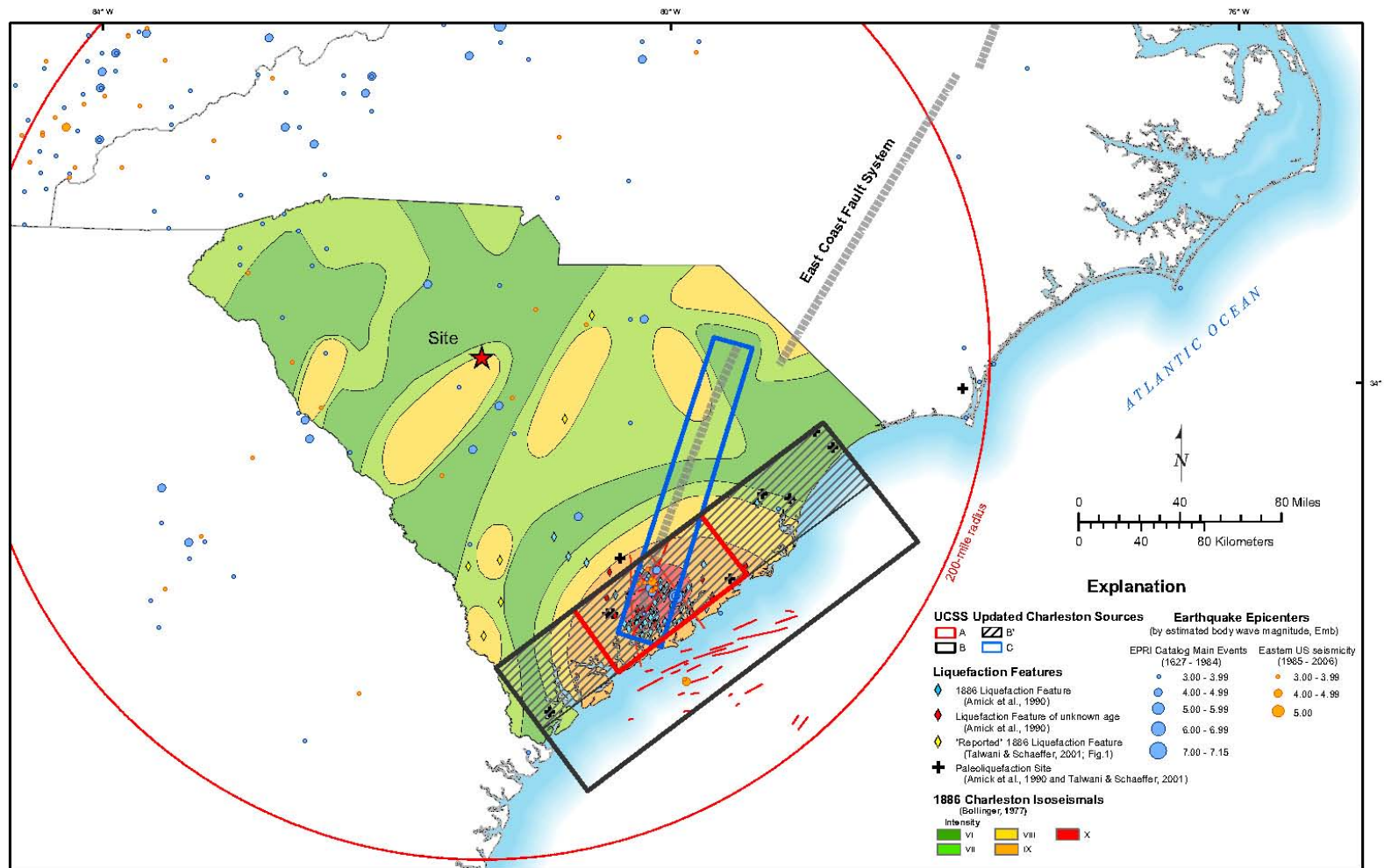
Figure 2.5.2-2. UCSS Model (Reproduced from VCSNS COL FSAR Figure 2.5.2-213)
