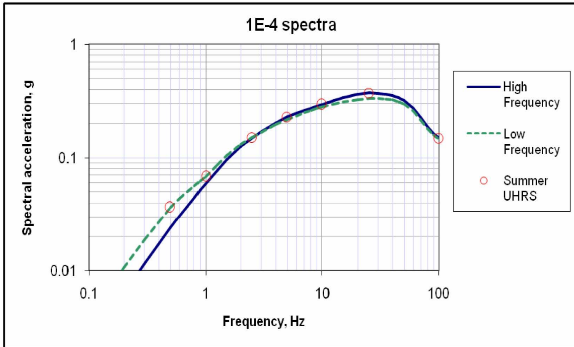
Figure 2.5.2-9. 10^{-4} Hard Rock UHRS (Depicted by Red Circles) and 10^{-4} High- and Low-Frequency Response Spectra (Depicted by Solid Blue and Dashed Green Curves, Respectively) (Reproduced from VCSNS COL FSAR Figure 2.5.2-242)
