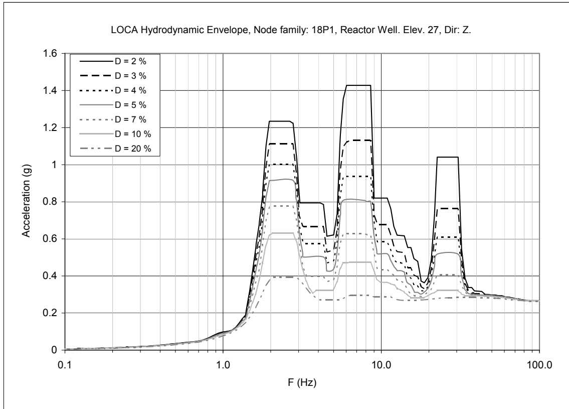
Figure 3F-26. Floor Response Spectra—Chugging & CO Envelope, Node Family: 18P1, Z-direction (Vertical)
