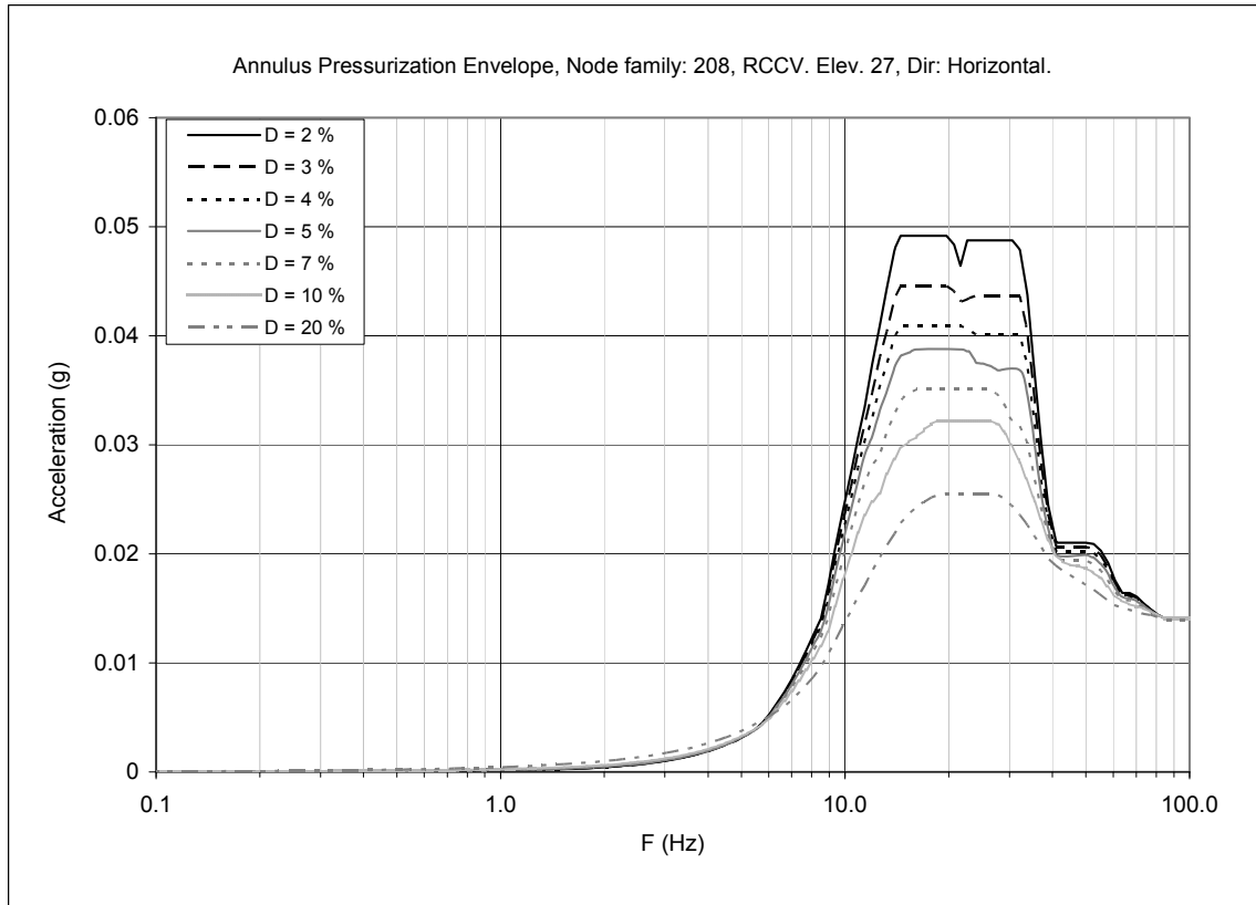
Figure 3F-10. Floor Response Spectra—Annulus Pressurization Envelope, Node Family: 208, Horizontal
