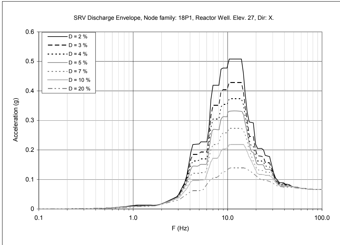
Figure 3F-18. Floor Response Spectra—SRV Discharge Envelope, Node Family: 18P1, X-direction (0°-180°)
