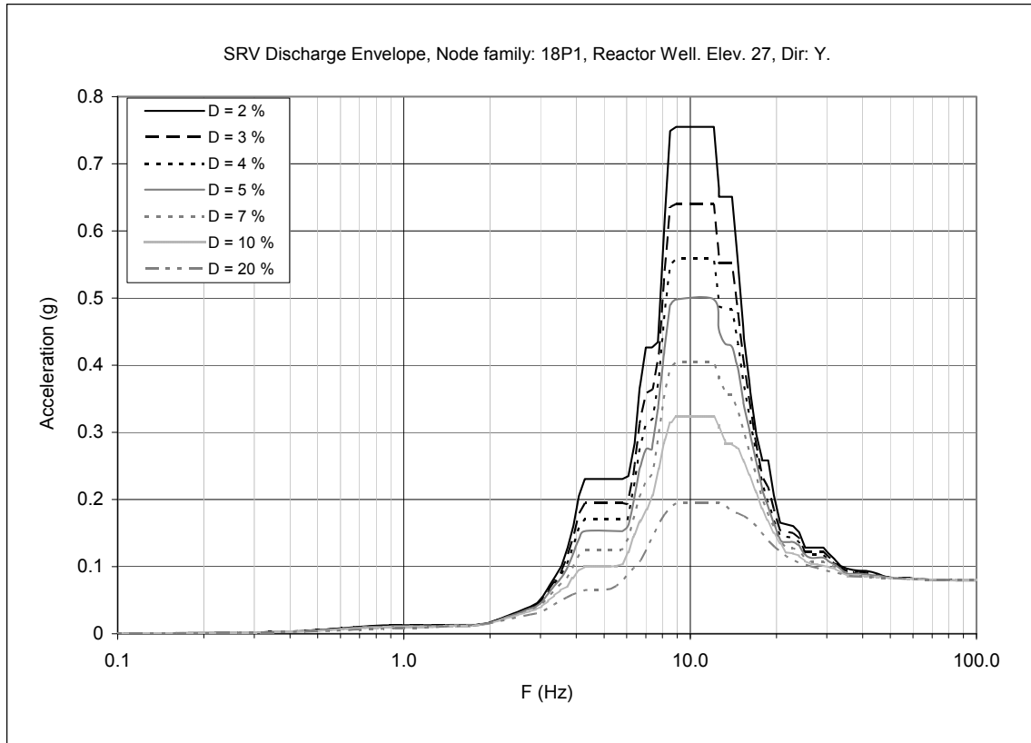
Figure 3F-22. Floor Response Spectra—SRV Discharge Envelope, Node Family: 18P1, Y-direction (90°-270°)
