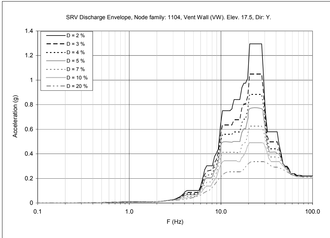
Figure 3F-19. Floor Response Spectra—SRV Discharge Envelope, Node Family: 1104, Y-direction (90°-270°)
