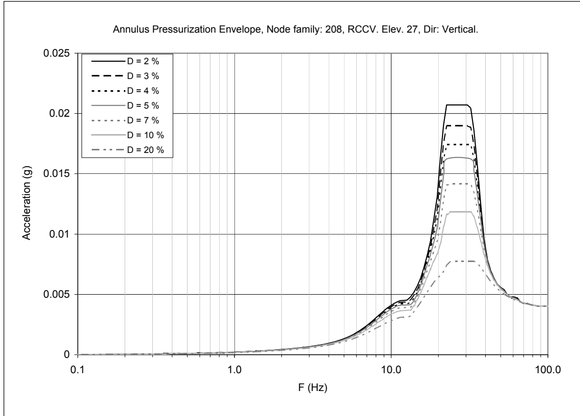
Figure 3F-7. Floor Response Spectra-Annulus Pressurization Envelope, Node Family: 208, Vertical
