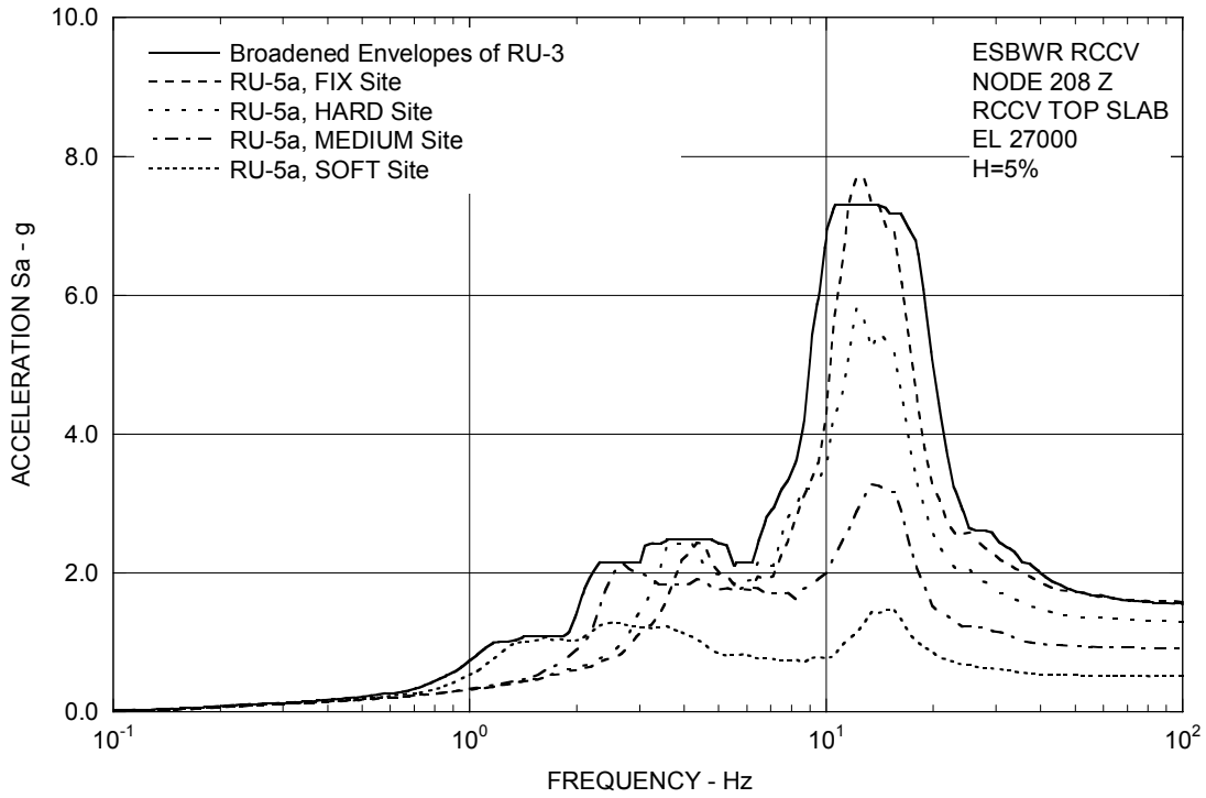
Figure 3A.8.4-6b. FRS (Effect of 100% Infill Concrete Stiffness of VW and D/F) – RCCV Top Slab Z
