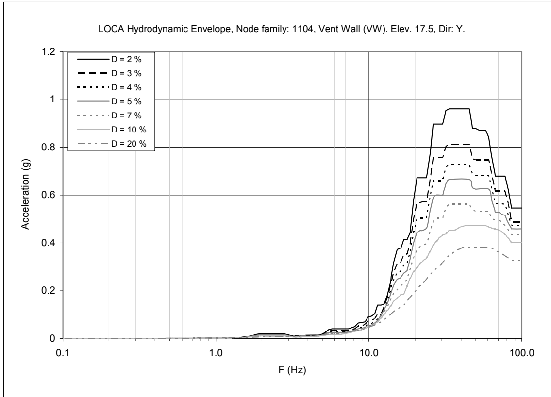
Figure 3F-31. Floor Response Spectra—Chugging & CO Envelope, Node Family: 1104, Y-direction (90°-270°)
