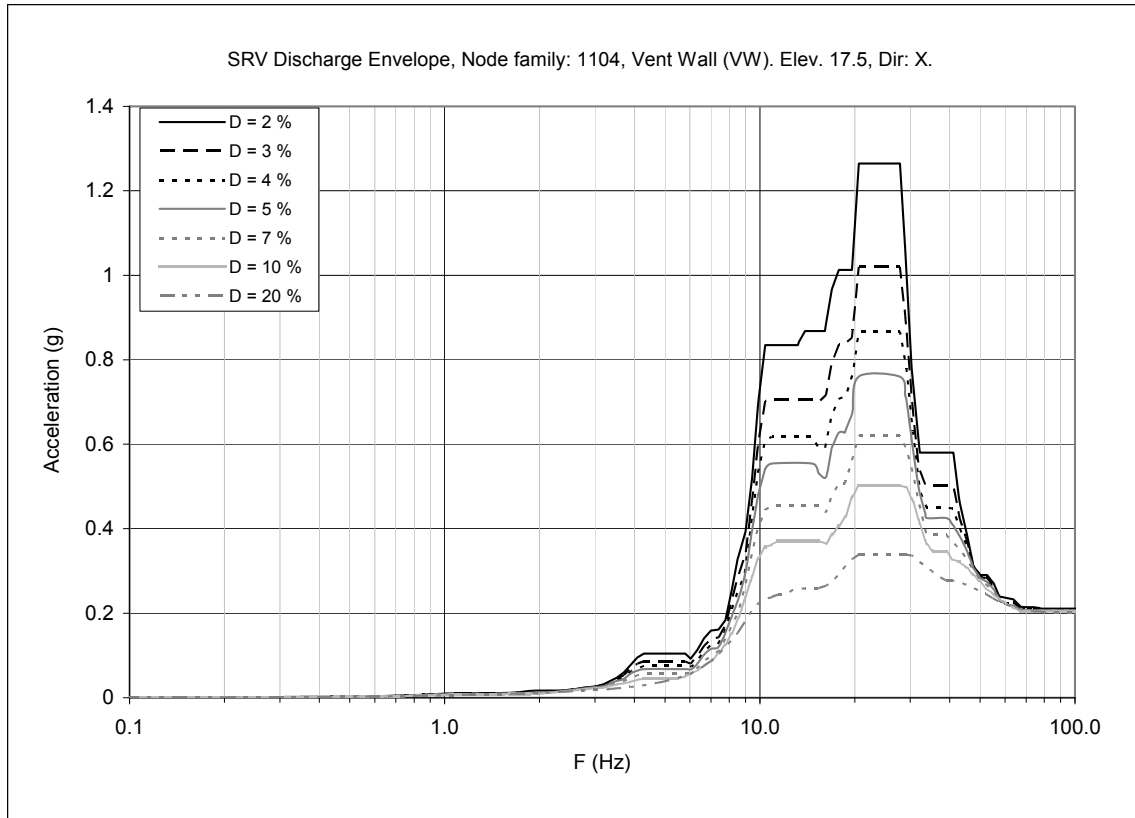
Figure 3F-15. Floor Response Spectra—SRV Discharge Envelope, Node Family: 1104, X-direction (0°-180°)
