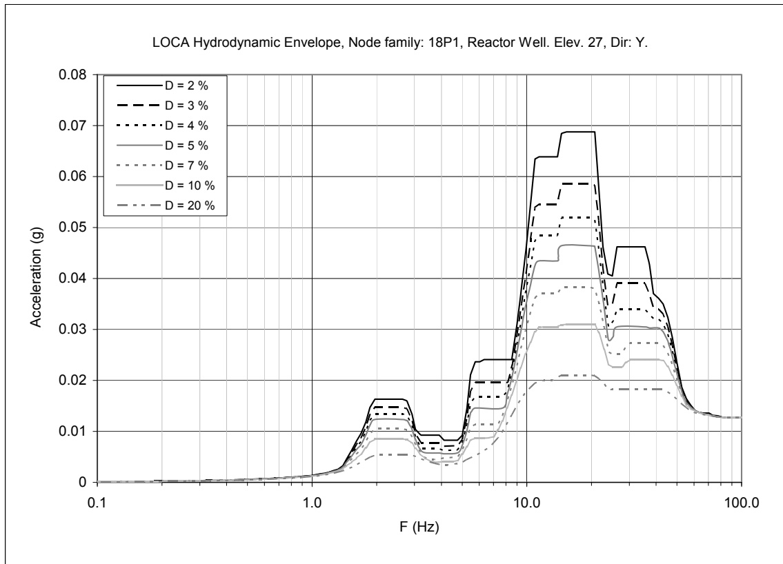
Figure 3F-34. Floor Response Spectra—Chugging & CO Envelope, Node Family: 18P1, Y-direction (90°-270°)]*
