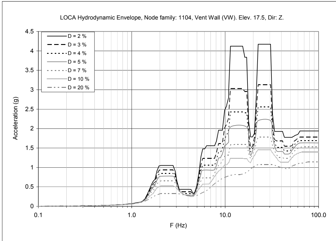
Figure 3F-23. Floor Response Spectra—Chugging & CO Envelope, Node Family: 1104, Z-direction (Vertical)
