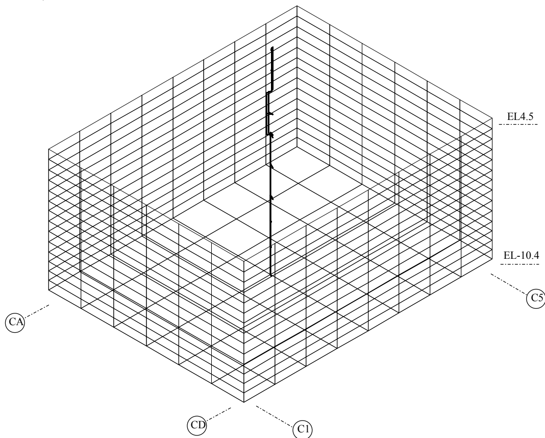
Figure 3A.7-13. Overview of CB SASSI2000 Model
