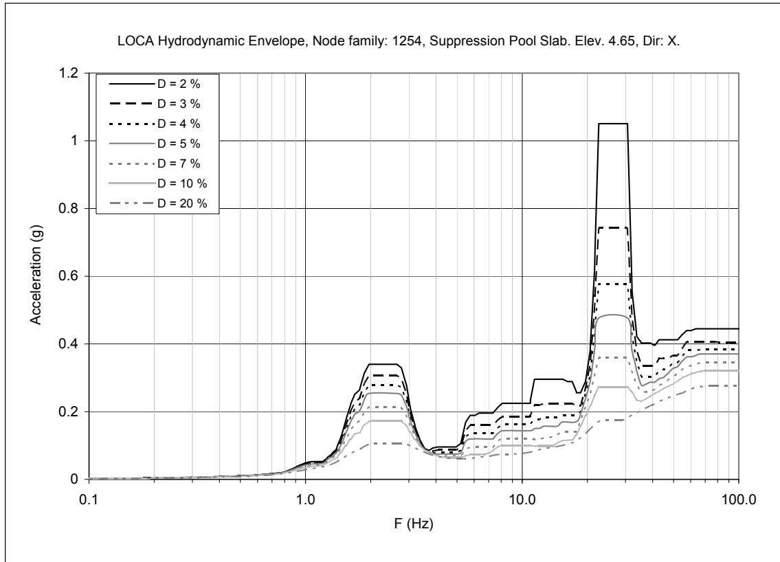
Figure 3F-28. Floor Response Spectra—Chugging & CO Envelope, Node Family: 1254, X-direction (0°-180°)
