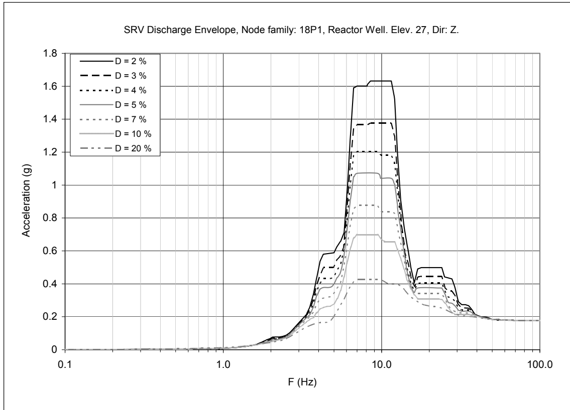
Figure 3F-14. Floor Response Spectra—SRV Discharge Envelope, Node Family: 18P1, Z-direction (Vertical)
