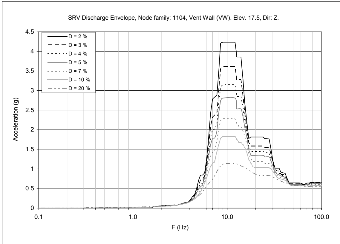
Figure 3F-11. Floor Response Spectra—SRV Discharge Envelope, Node Family: 1104, Z-direction (Vertical)
