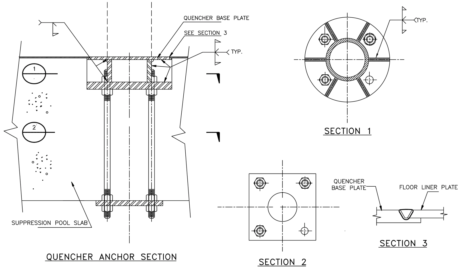
Figure 3.8-5. Quencher Anchorage
