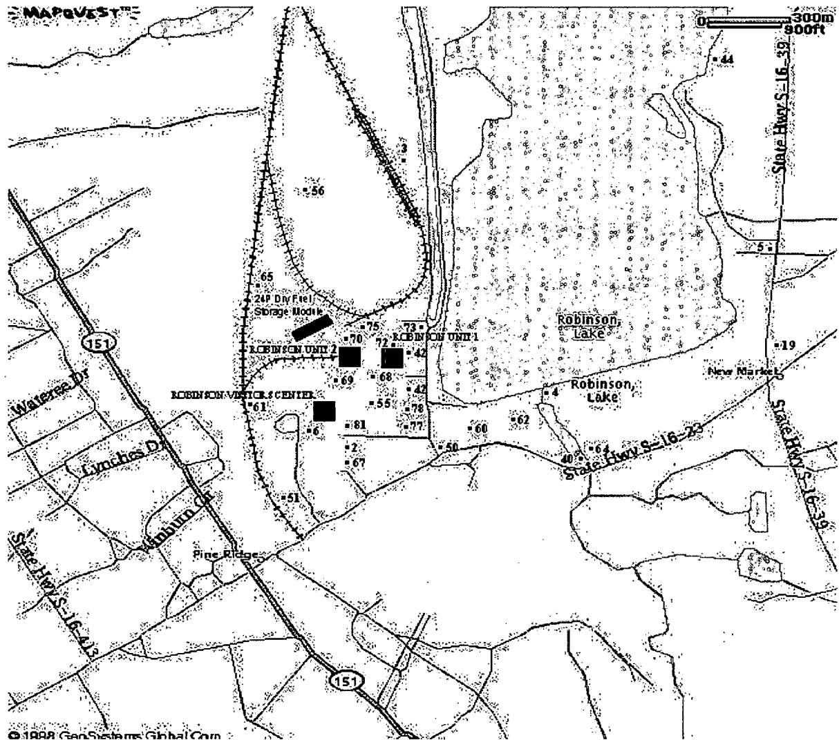
FIGURE 4-1 RADIOLOGICAL SAMPLE LOCATIONS NEAR SITE
