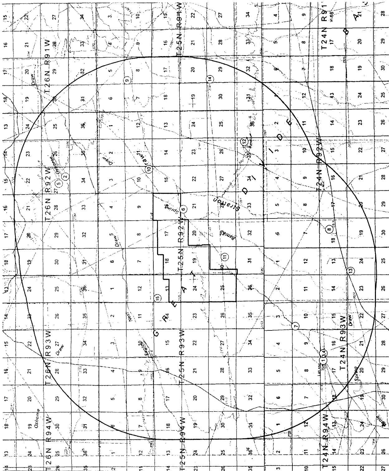
Figure 3.8: Domestic and Stock Wells within Five Miles of the Lost Creek Project Area (LCI, 2008c)
