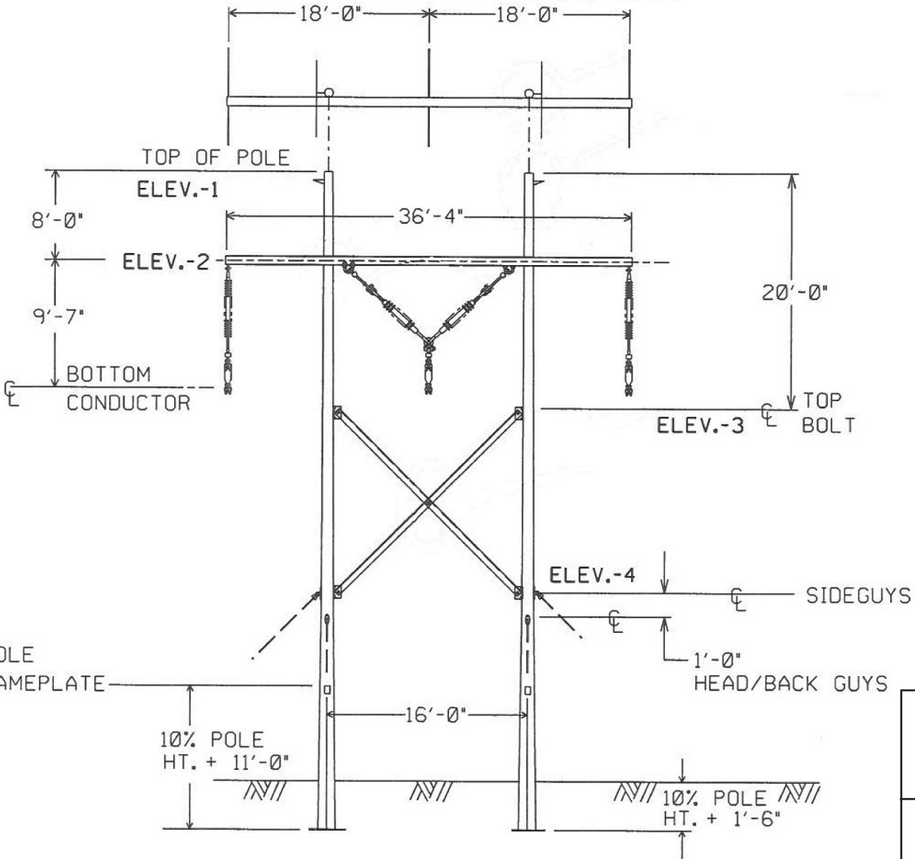
Typical Design of a Pole H-Frame Support Structure for Transmission Lines FIGURE 3.7-4
