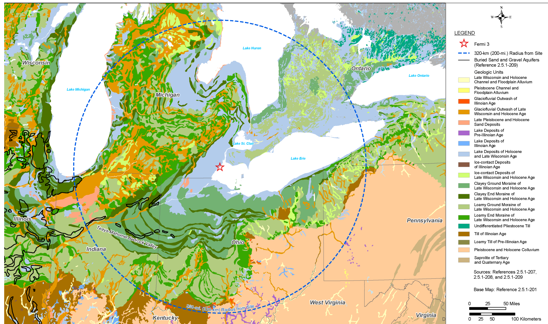
Figure 2.5.1-205 Quaternary Geology Map of the Fermi 3 Site Region
