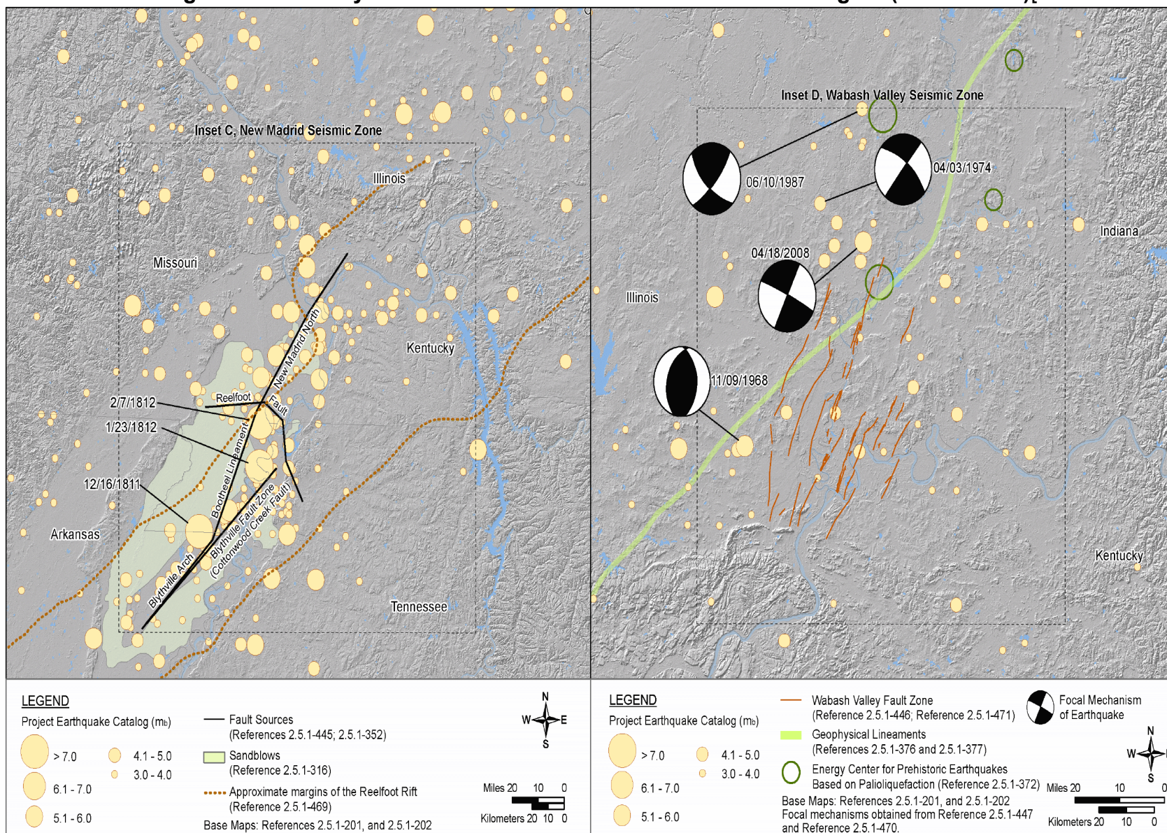
Figure 2.5.1-207 Regional Seismicity and tectonic Features in the Fermi 3 Site Region (Sheet 3 of 3)[EF3 COL 2.0-26-A]
