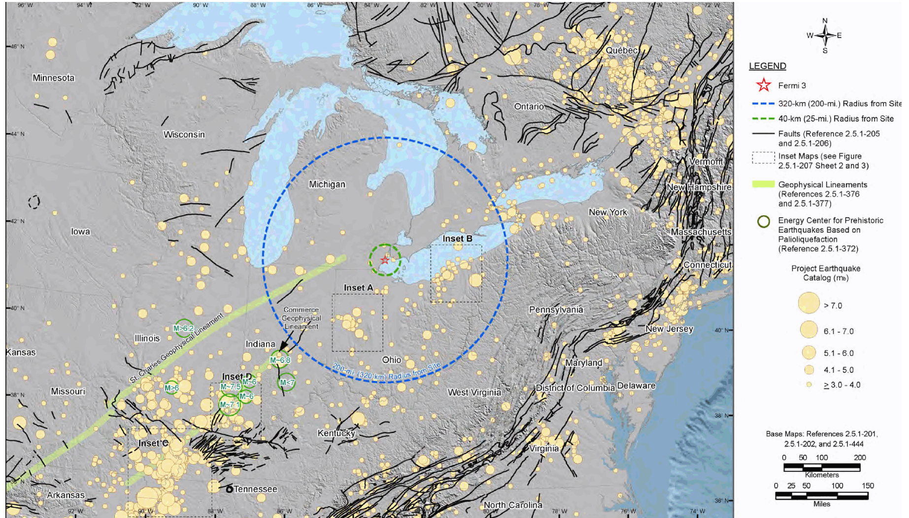
Figure 2.5.1-207 Regional Seismicity and Tectonic Features in the Fermi 3 Site Region (Sheet 1 of 3)
