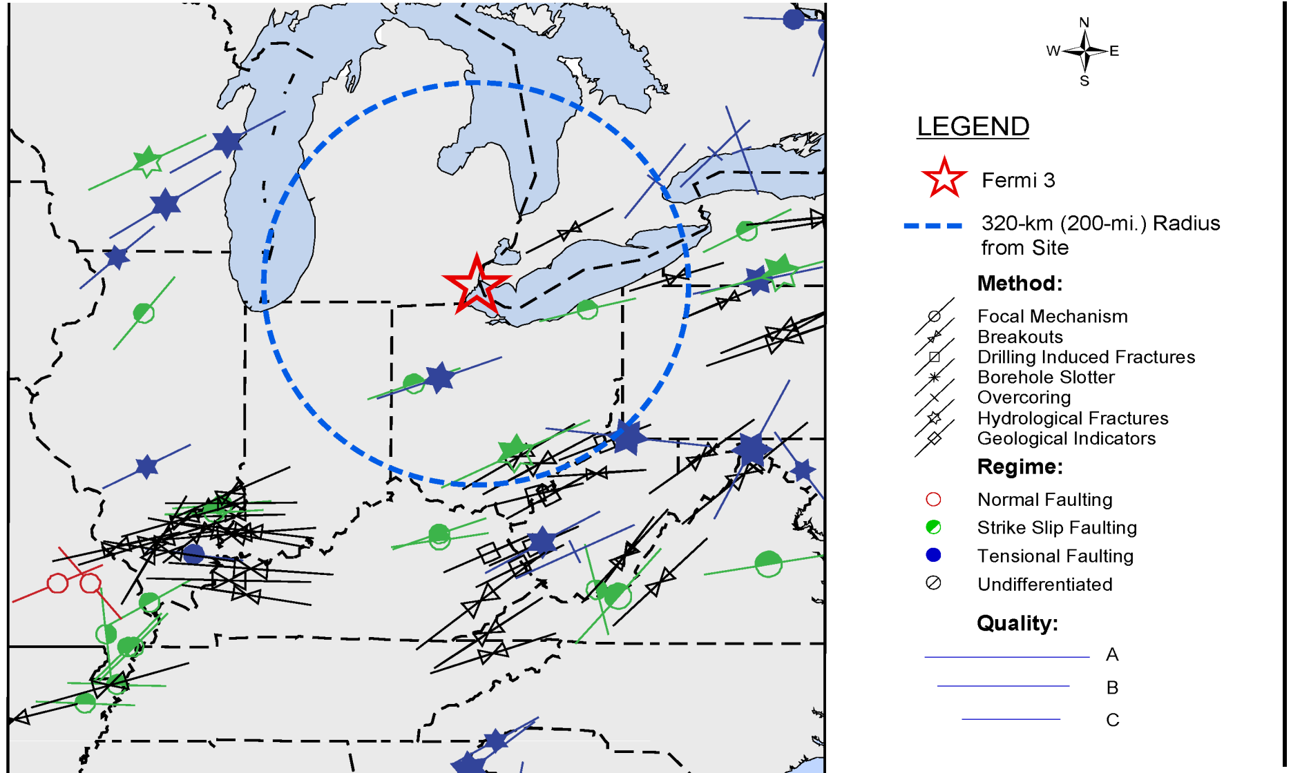
Figure 2.5.1-219 World Stress Map Showing Maximum Horizontal Stress Trajectory in the Fermi 3 Site Region [EF3 COL 2.0-26-A]
