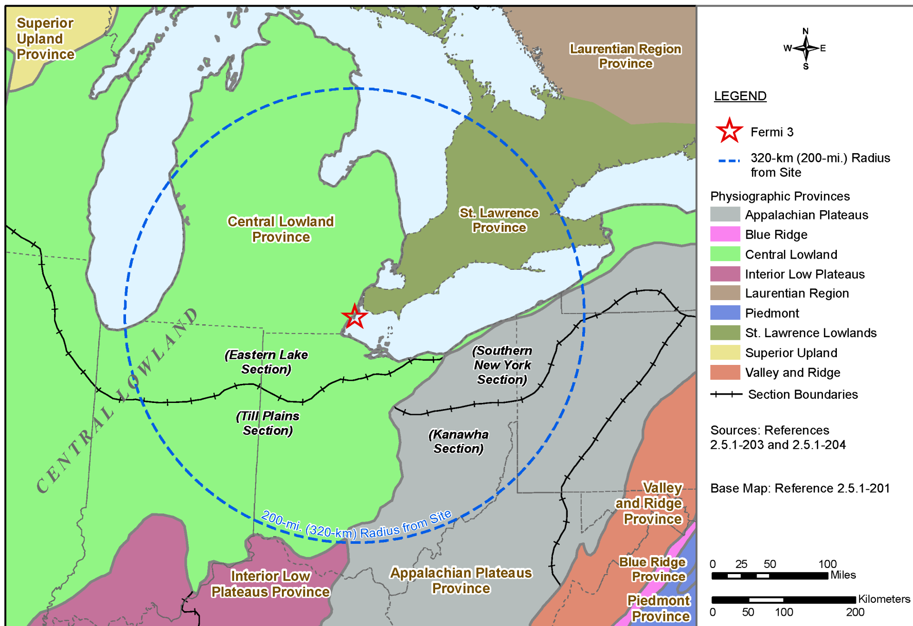
Figure 2.5.1-202 Fermi 3 Site Regional Physiographic Map
