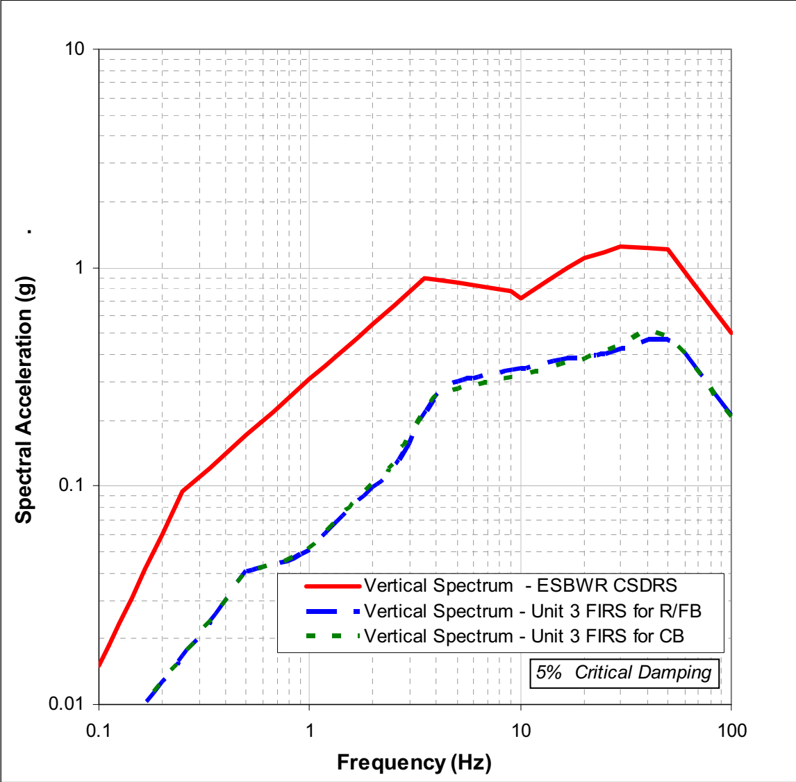
Figure 2.0-202 Comparison of Vertical CSDRS with the Unit 3 FIRS for the R/FB and CB [EF3 COL 2.0-1-A]
