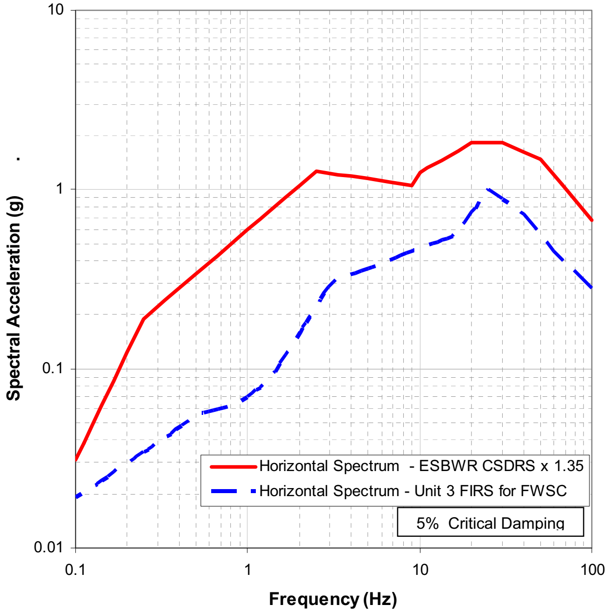
Figure 2.0-203 Comparison of Horizontal CSDRS with the Unit 3 FIRS for the FWSC [EF3 COL 2.0-1-A]
