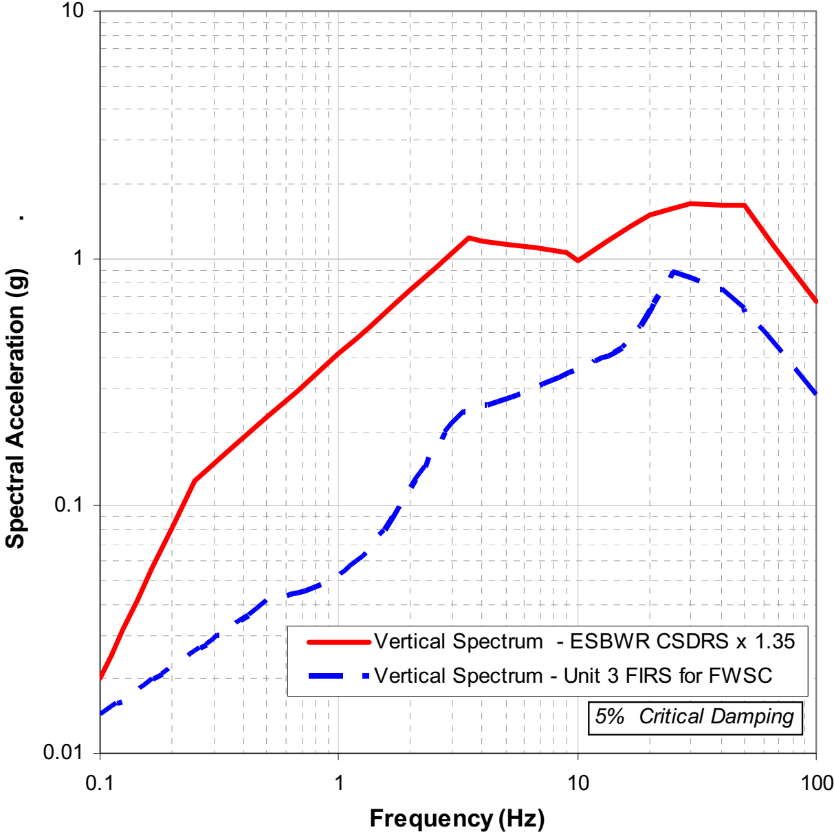
Figure 2.0-204 Comparison of Vertical CSDRS with the Unit 3 FIRS for the FWSC [EF3 COL 2.0-1-A]
