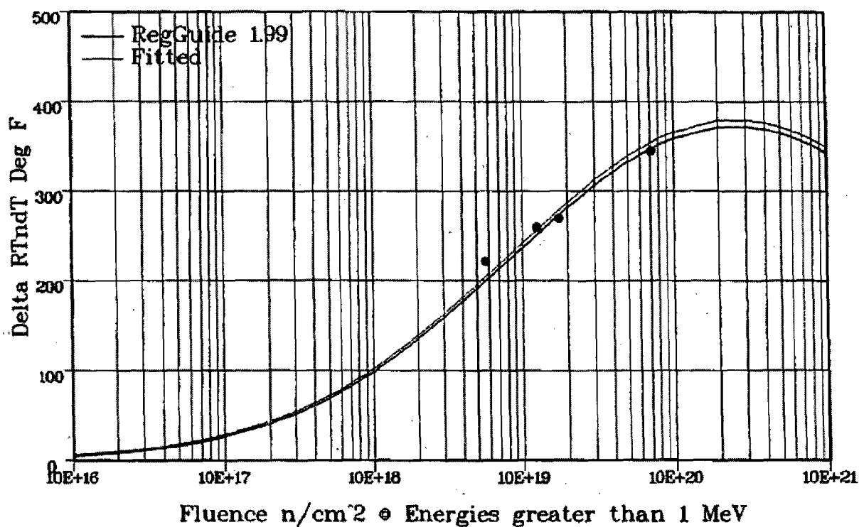
Figure 2-5 Maine Yankee Surveillance Weld Data
