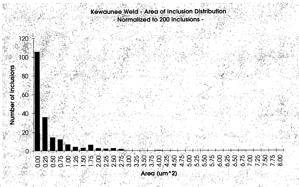
Figure 1 Normalized area distribution for (a) the Maine Yankee surveillance weld and (b) the Kewaunee surveillance weld materials, respectively.
