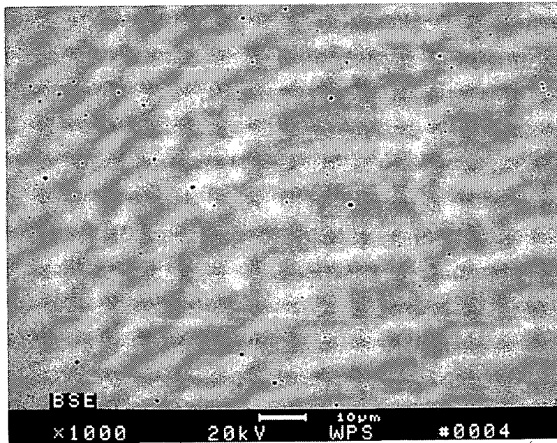
Figure 4b SEM Backscatter Micrograph of Kewaunee Surveillance Weld
