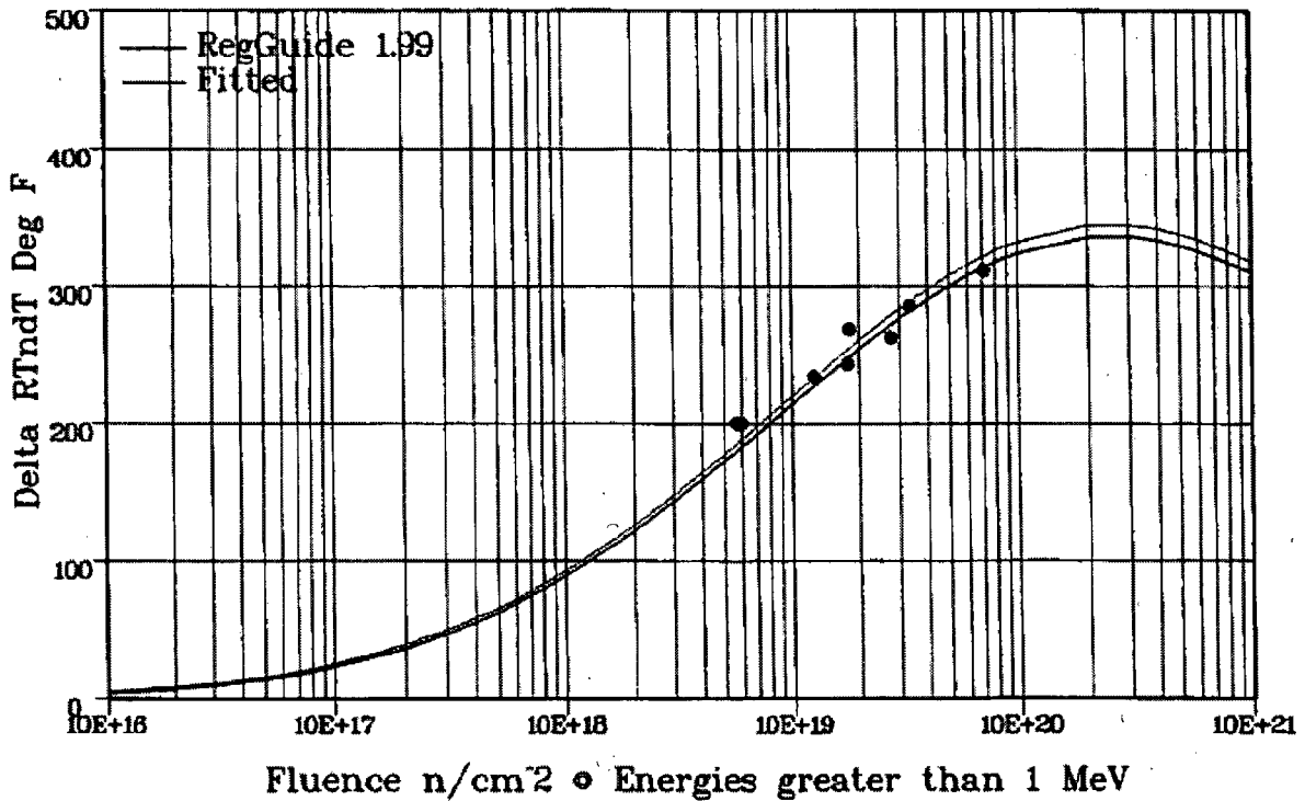
Figure 2-8 Kewaunee and Maine Yankee Surveillance Welds Using Ratioing
