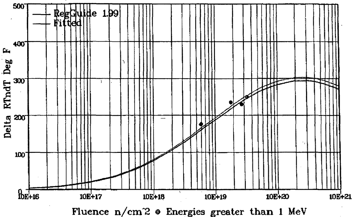
Figure 2-4 Kewaunee Surveillance Weld Data
