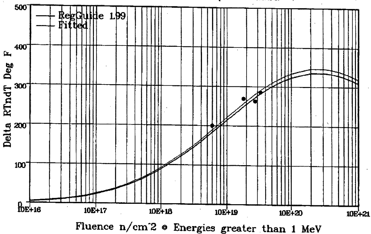
Figure 2-9 Kewaunee Surveillance Weld Data Using Ratioing
