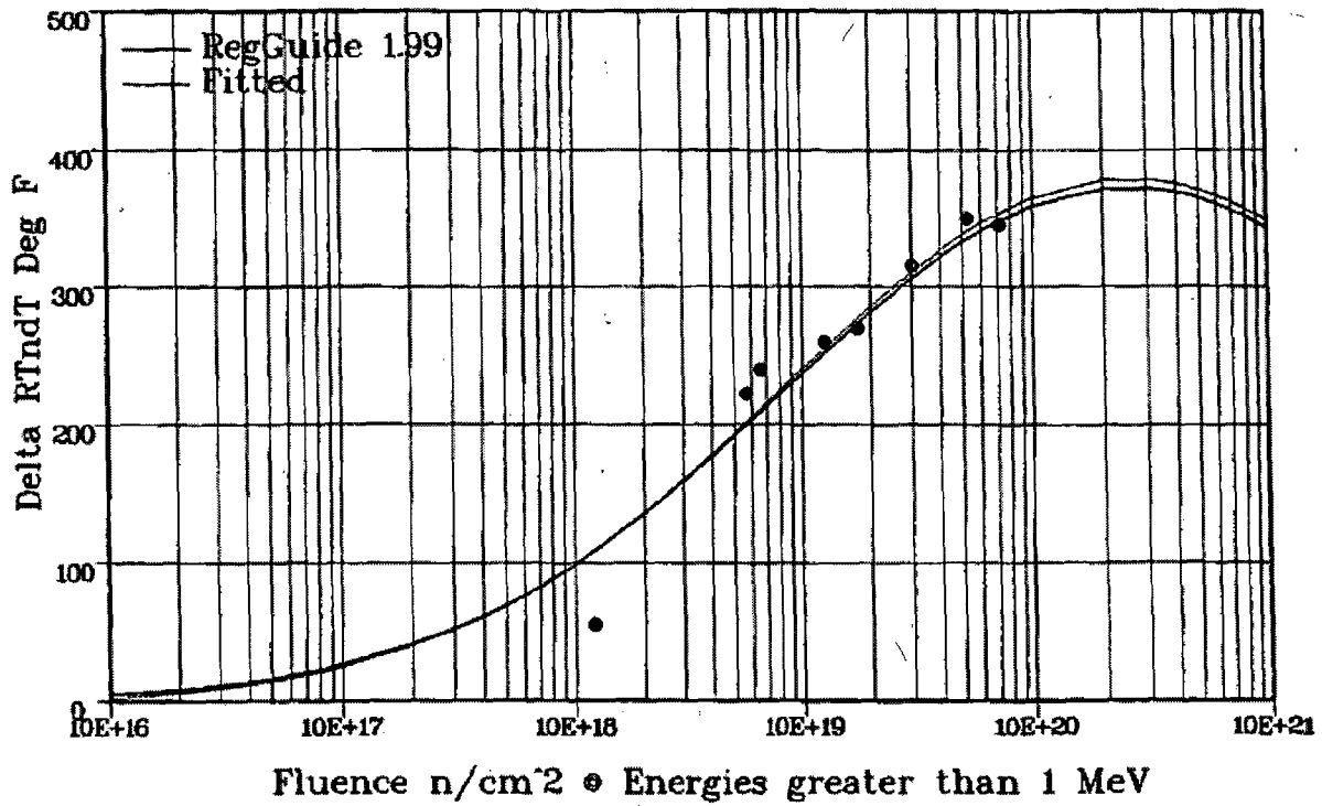
Figure 2-6 Maine Yankee Surveillance Plus MTR Weld Data
