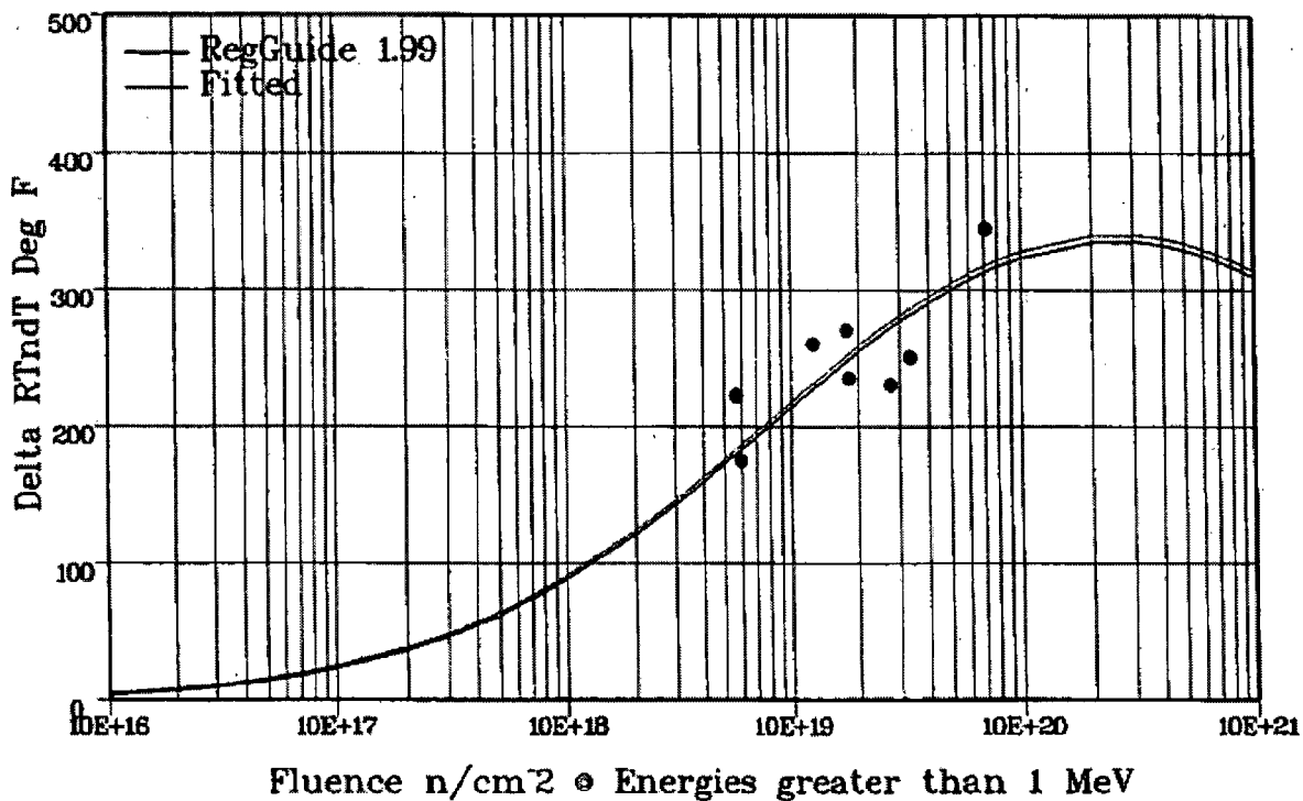
Figure 2-7 Kewaunee and Maine Yankee Surveillance Welds (No Ratioing)
