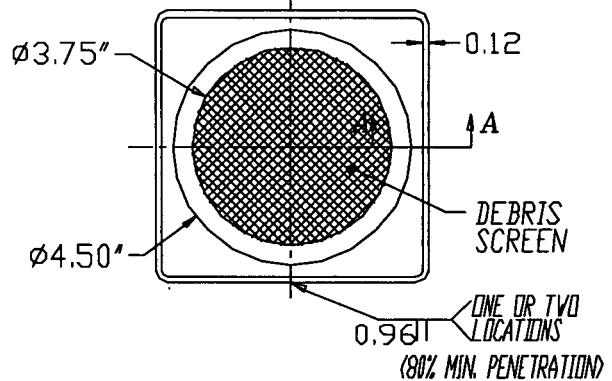
FIGURE 2.1.1; DAMAGED FUEL CONTAINER FOR DRESDEN UNIT-1/ HUMBOLDT BAY SNF
