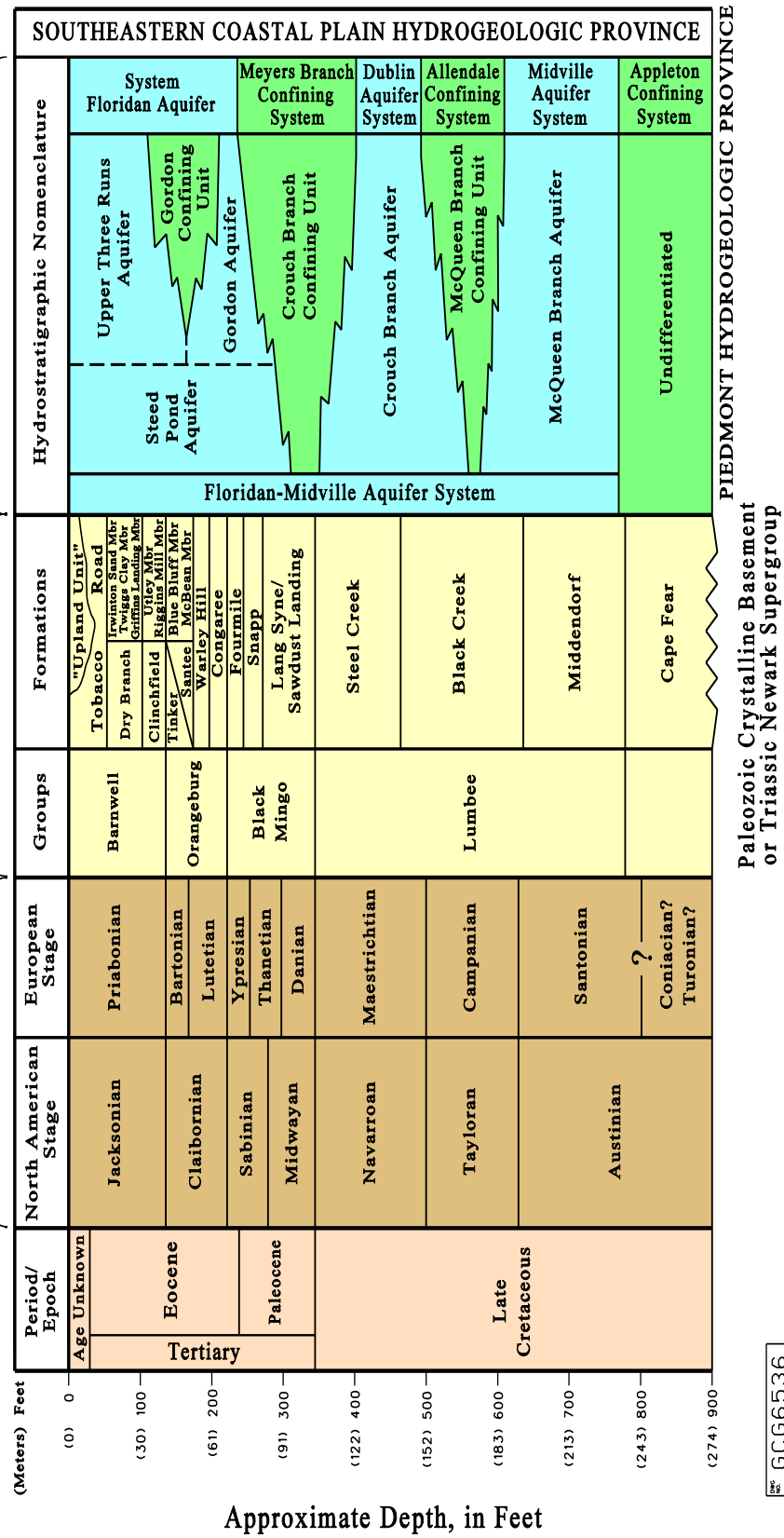
Figure 1.3.4-8. Comparison of Chronostratigraphic, Lithostratigraphic, and Hydrostratigraphic Units in the SRS Region
