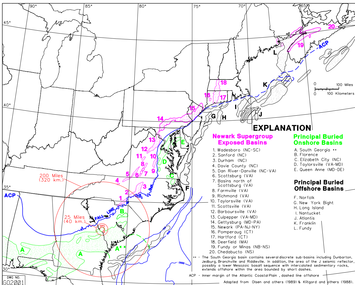
Figure 1.3.5-4. Location of Mesozoic Rift Basins Along the Entire Eastern Continental Margin of North America from the Gulf Coast Through Nova Scotia
