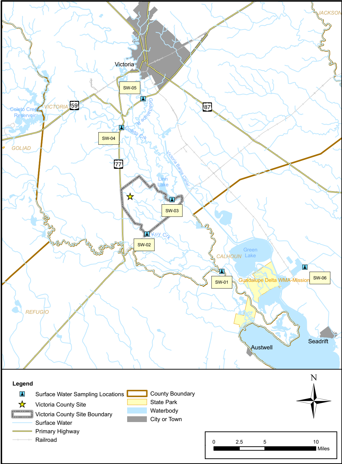
Figure 2.3.3-4 VCS Site Surface Water Sample Locations
