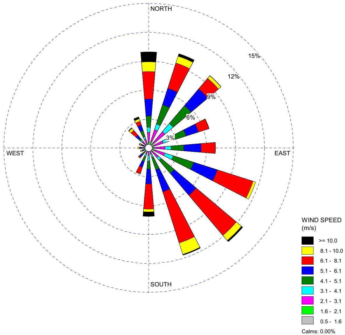
Figure 2.3.2-11 60-Meter Level Wind Rose — Autumn VCS Pre-Application Monitoring Program (July 1, 2007–June 30, 2009)
