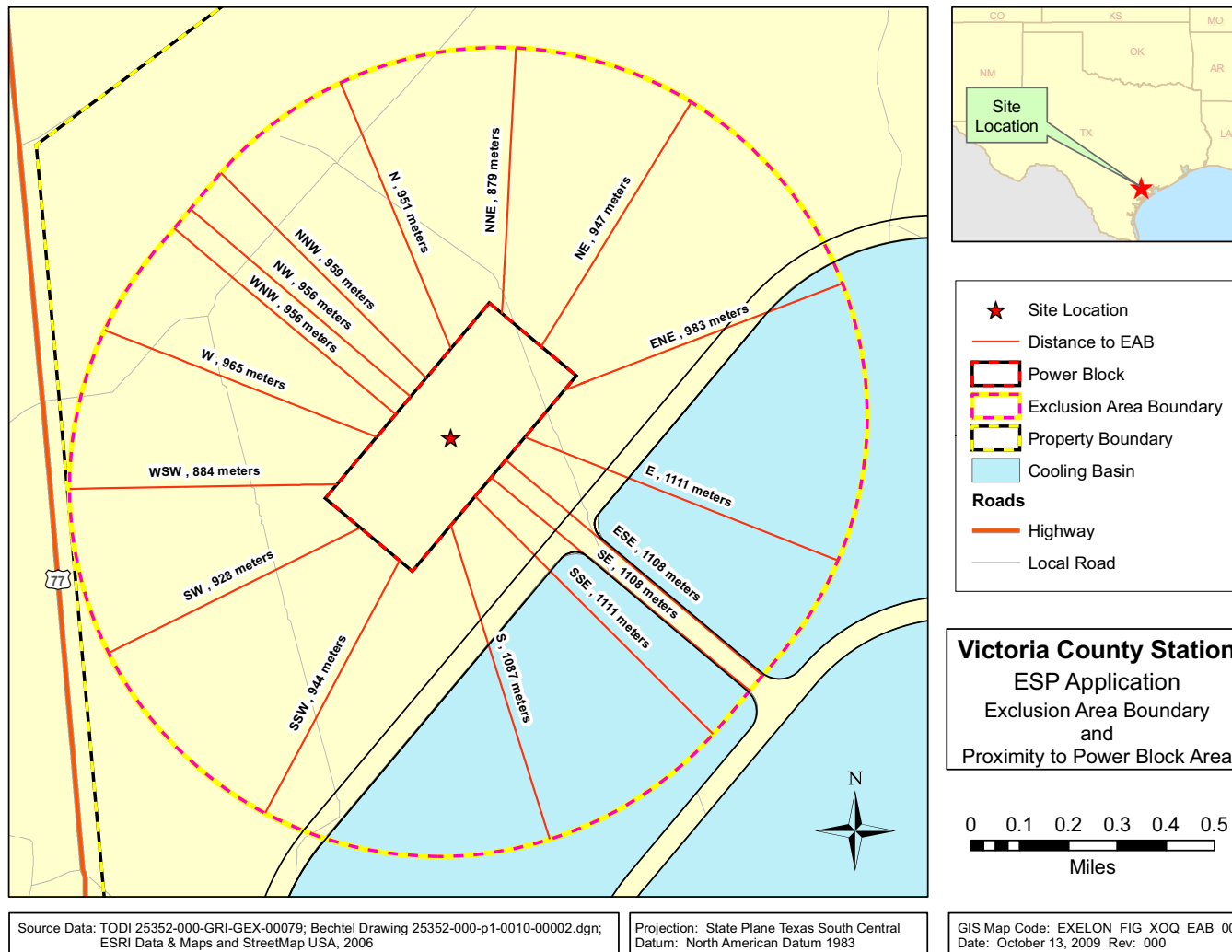
Figure 2.3.4-1 Distance to EAB from the Source Boundary
