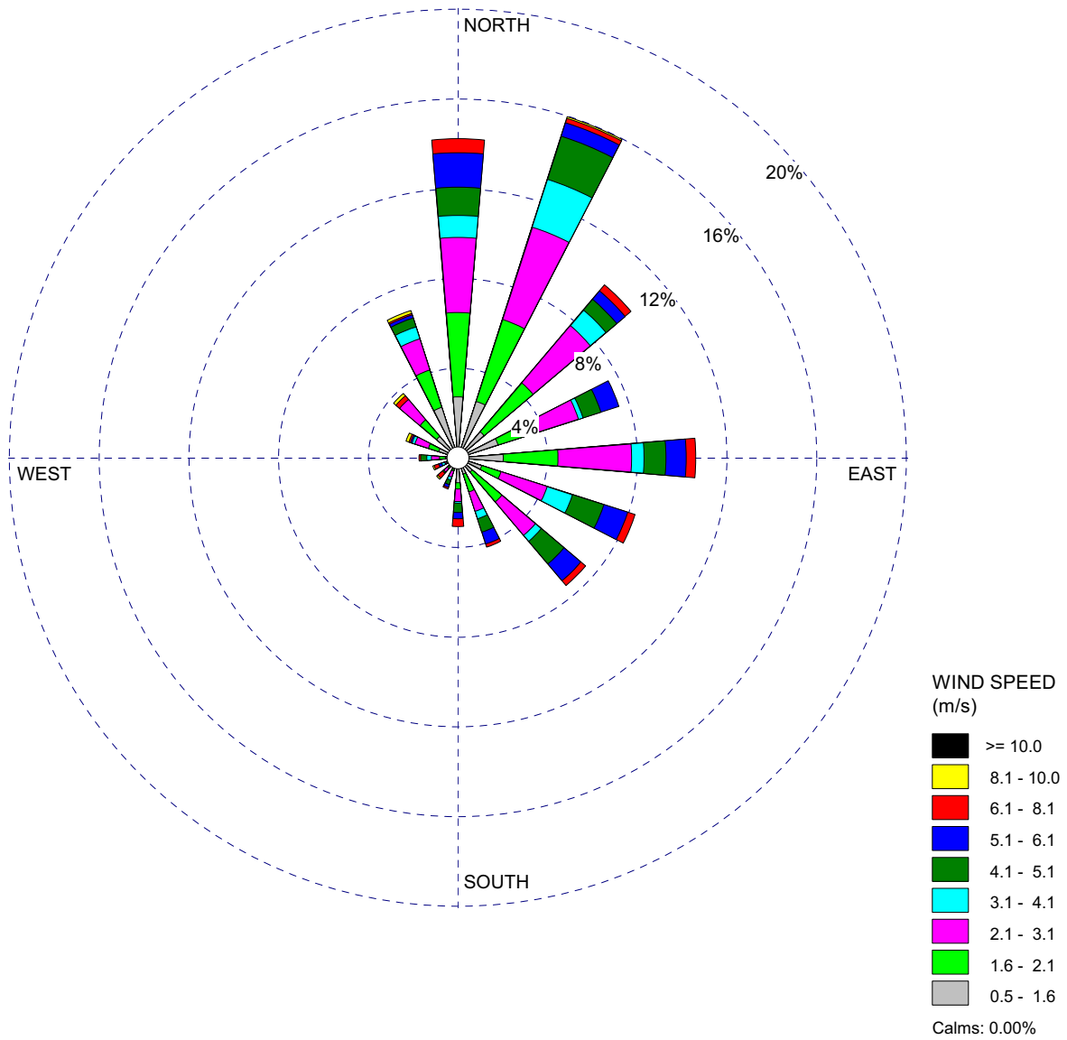
Figure 2.3.2-6 10-Meter Level Wind Rose — September (Sheet 9 of 12) VCS Pre-Application Monitoring Program (July 1, 2007–June 30, 2009)
