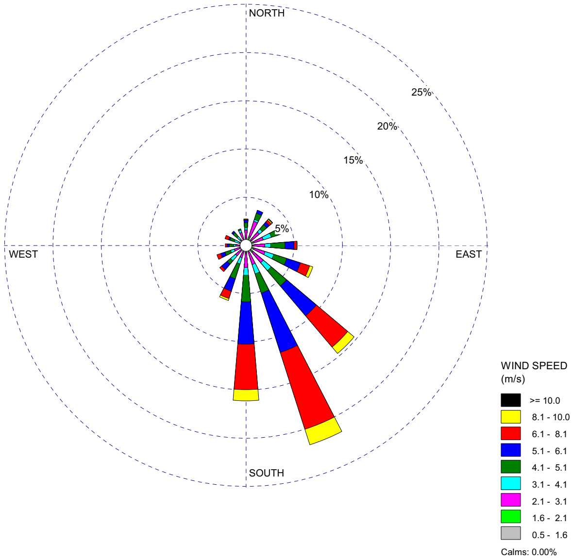
Figure 2.3.2-12 60-Meter Level Wind Rose — August (Sheet 8 of 12) VCS Pre-Application Monitoring Program (July 1, 2007–June 30, 2009)
