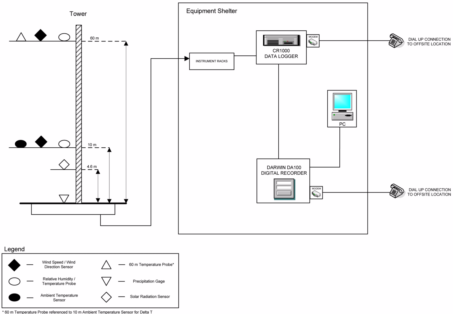
Figure 2.3.3-5 Onsite Meteorological Monitoring System Block Diagram
