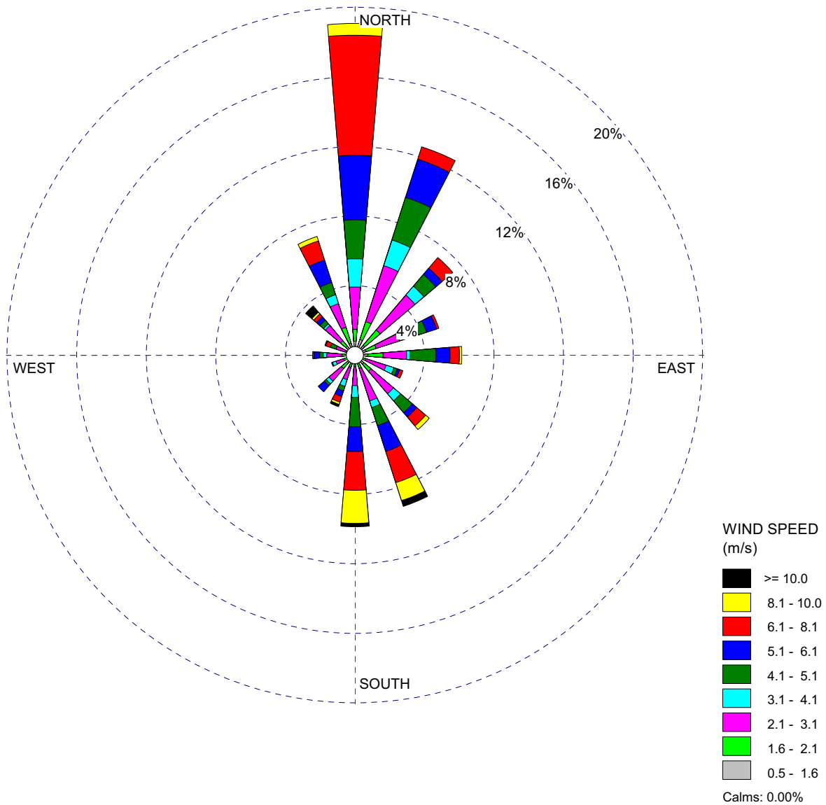
Figure 2.3.2-6 10-Meter Level Wind Rose — January (Sheet 1 of 12) VCS Pre-Application Monitoring Program (July 1, 2007–June 30, 2009)
