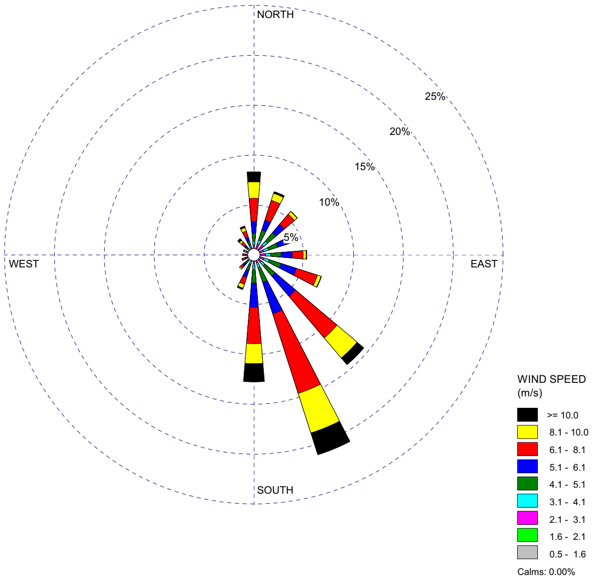
Figure 2.3.2-7 60-Meter Level Wind Rose — Annual VCS Pre-Application Monitoring Program (July 1, 2007–June 30, 2009)
