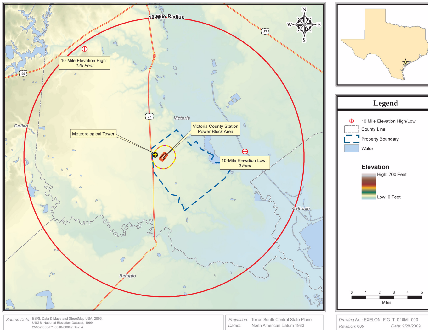
Figure 2.3.3-2 Site and Vicinity Map (10-Mile Radius)
