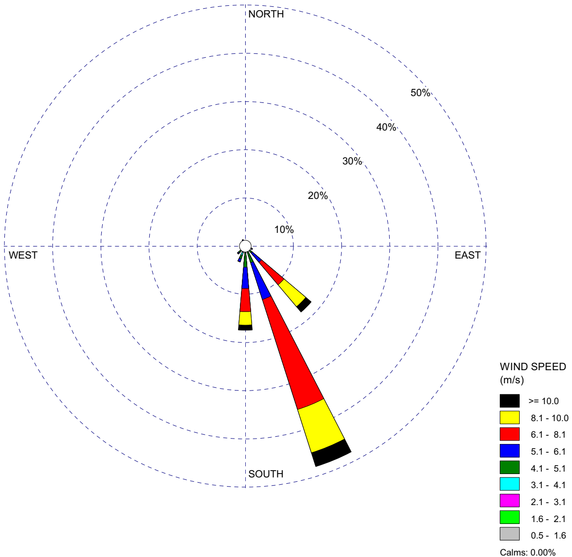
Figure 2.3.2-12 60-Meter Level Wind Rose — June (Sheet 6 of 12) VCS Pre-Application Monitoring Program (July 1, 2007–June 30, 2009)
