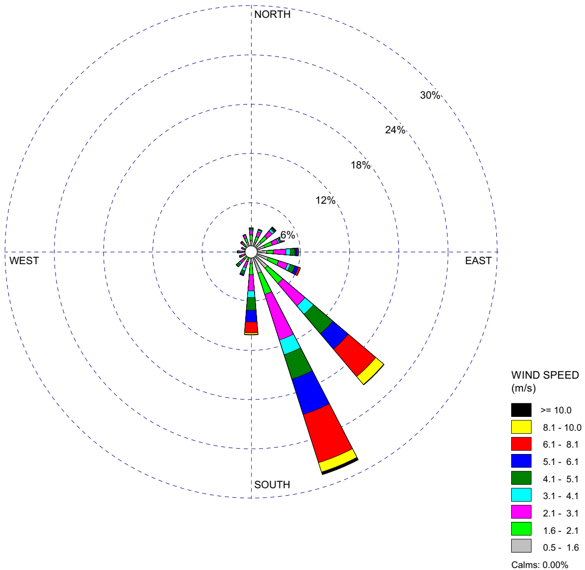
Figure 2.3.2-4 10-Meter Level Wind Rose — Summer VCS Pre-Application Monitoring Program (July 1, 2007–June 30, 2009)
