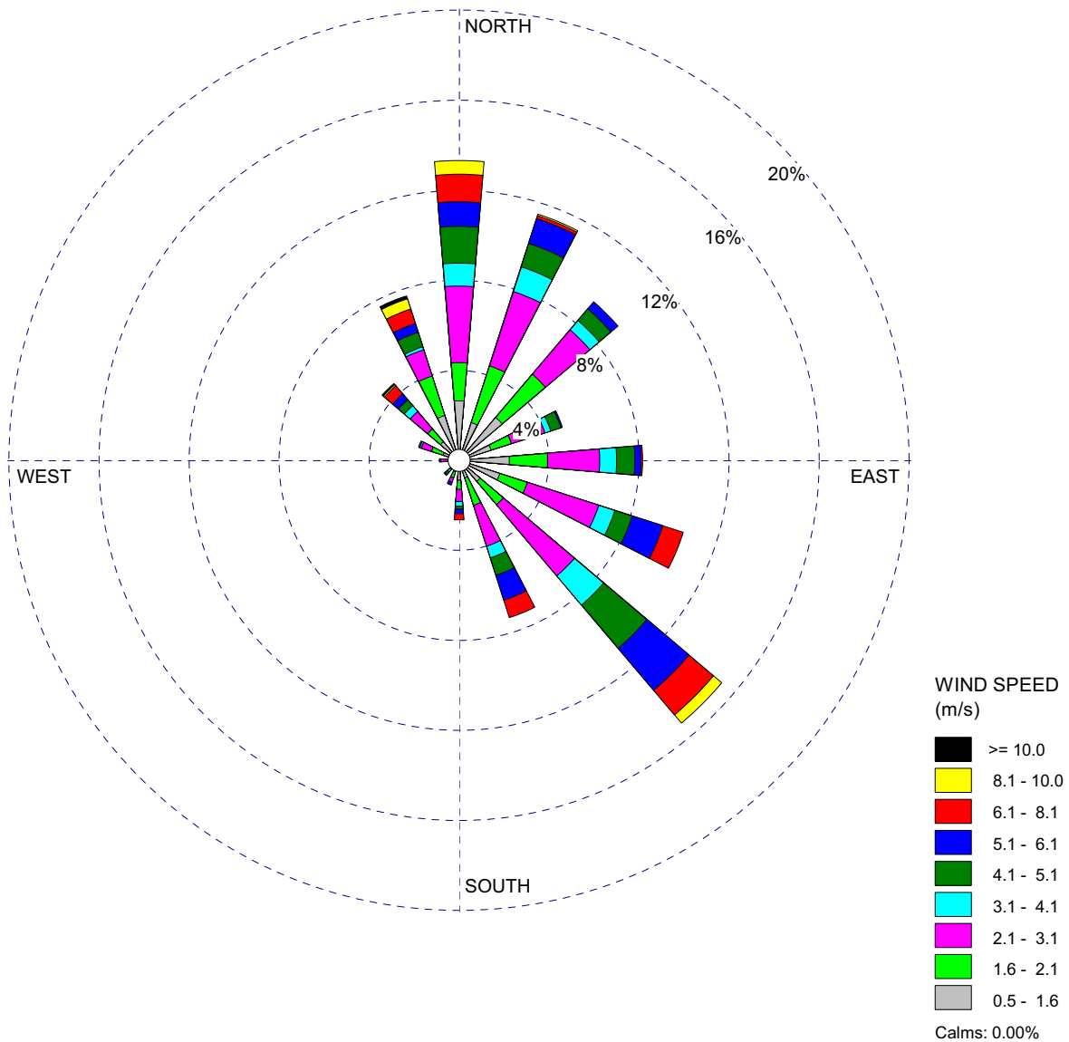
Figure 2.3.2-6 10-Meter Level Wind Rose — October (Sheet 10 of 12) VCS Pre-Application Monitoring Program (July 1, 2007–June 30, 2009)
