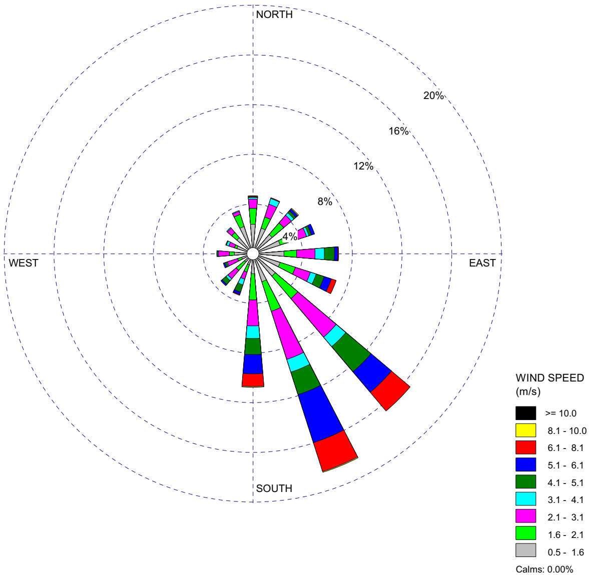
Figure 2.3.2-6 10-Meter Level Wind Rose — August (Sheet 8 of 12) VCS Pre-Application Monitoring Program (July 1, 2007–June 30, 2009)
