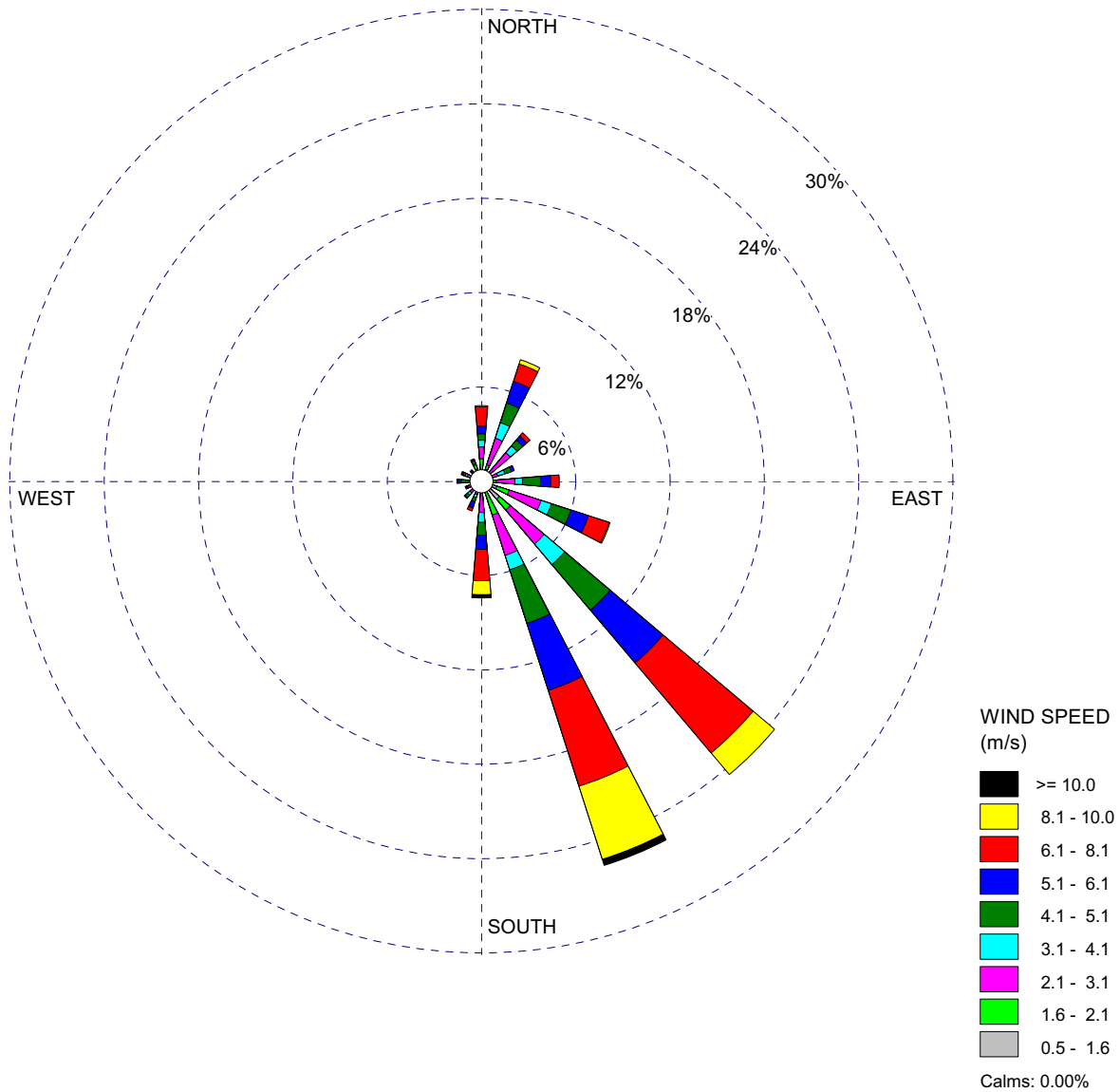
Figure 2.3.2-6 10-Meter Level Wind Rose — May (Sheet 5 of 12) VCS Pre-Application Monitoring Program (July 1, 2007–June 30, 2009)
