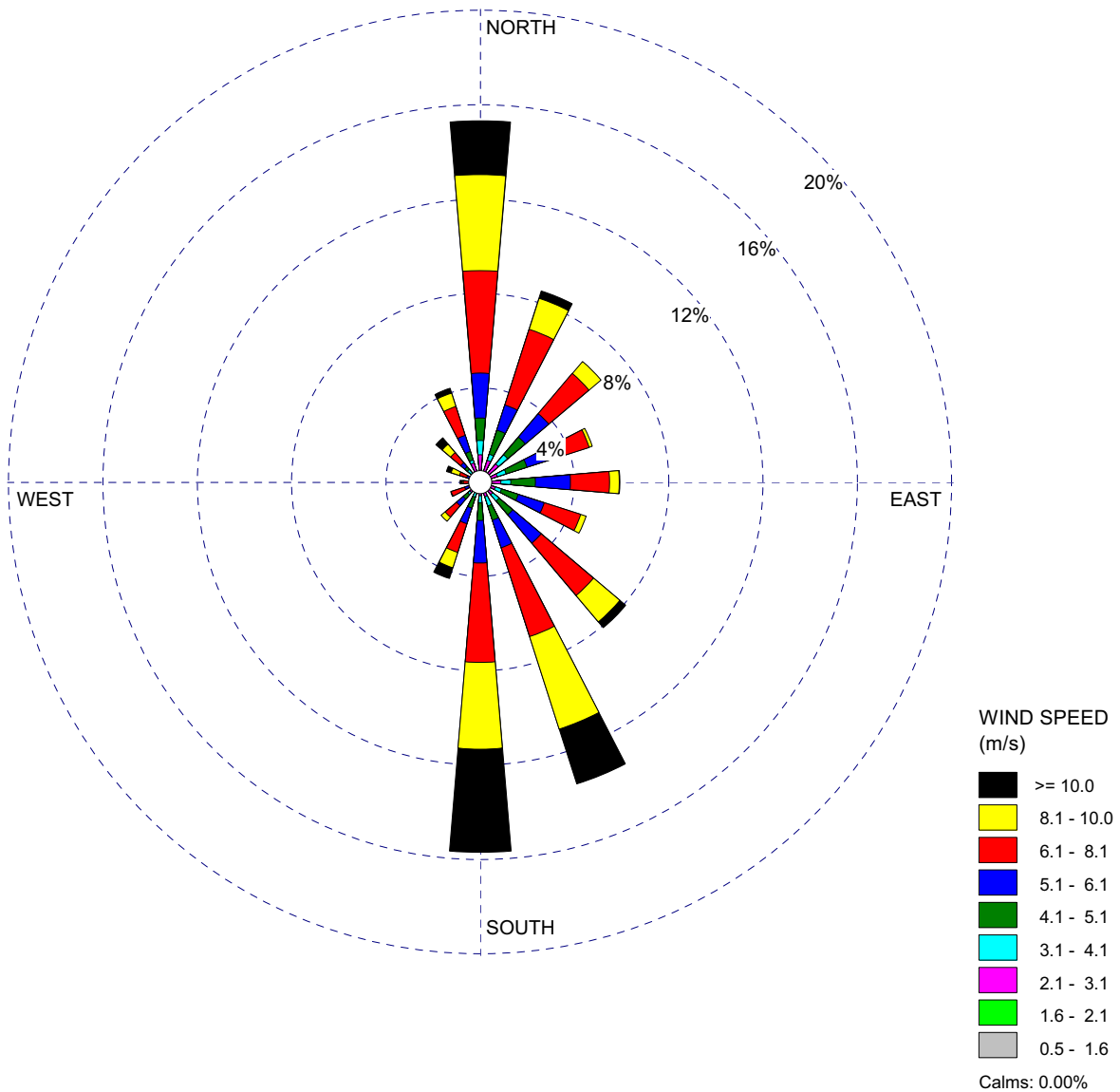
Figure 2.3.2-8 60-Meter Level Wind Rose — Winter VCS Pre-Application Monitoring Program (July 1, 2007–June 30, 2009)
