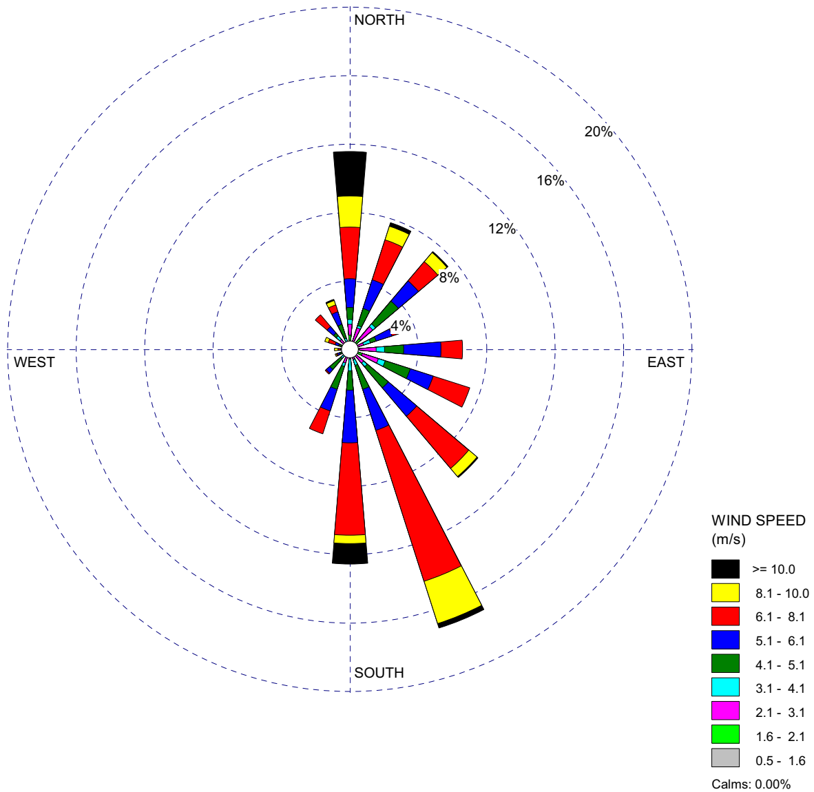
Figure 2.3.2-12 60-Meter Level Wind Rose — November (Sheet 11 of 12) VCS Pre-Application Monitoring Program (July 1, 2007–June 30, 2009)
