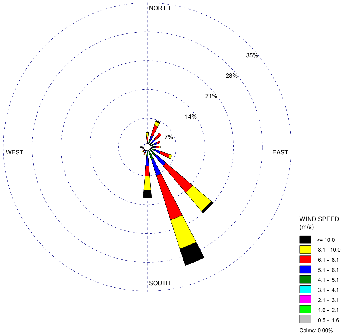
Figure 2.3.2-12 60-Meter Level Wind Rose — May (Sheet 5 of 12) VCS Pre-Application Monitoring Program (July 1, 2007–June 30, 2009)
