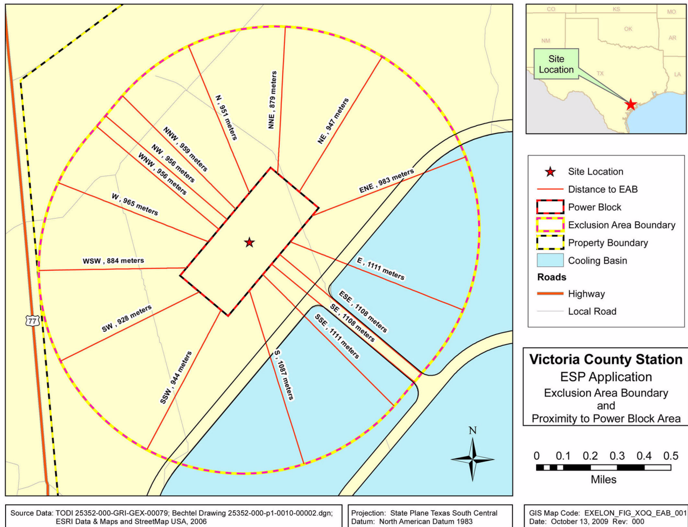
Figure 2.1-3 VCS Site Plan with Exclusion Area Boundary Map
