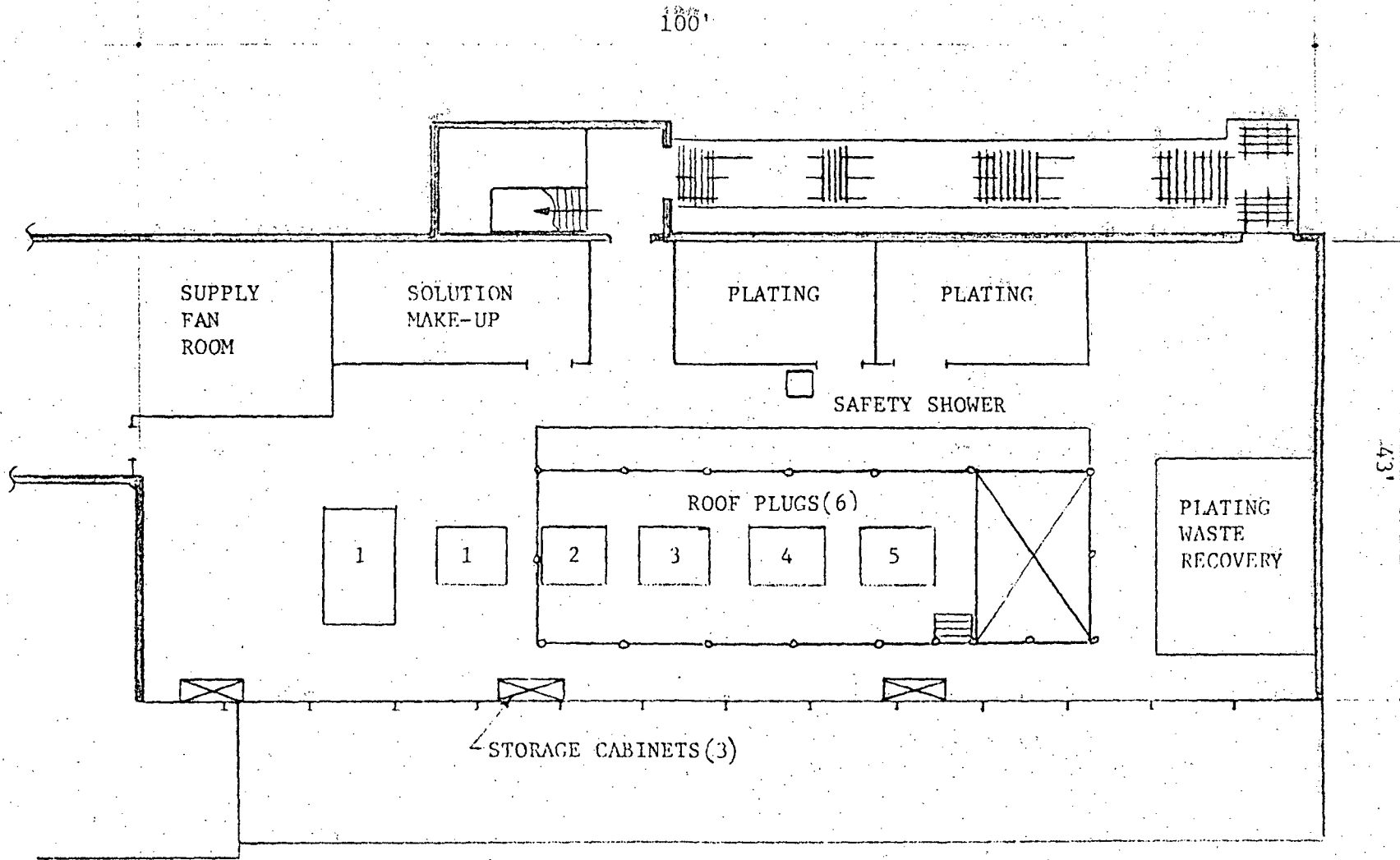
HOT LABORATORY - FLOOR PLAN - UPPER LEVEL
