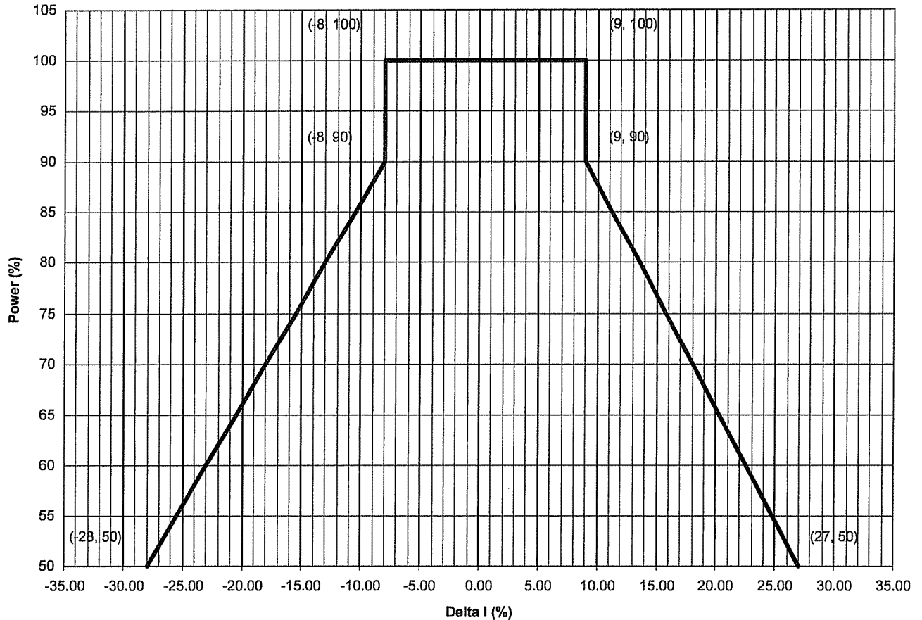
FIGURE 6 FLUX DIFFERENCE OPERATING ENVELOPE
