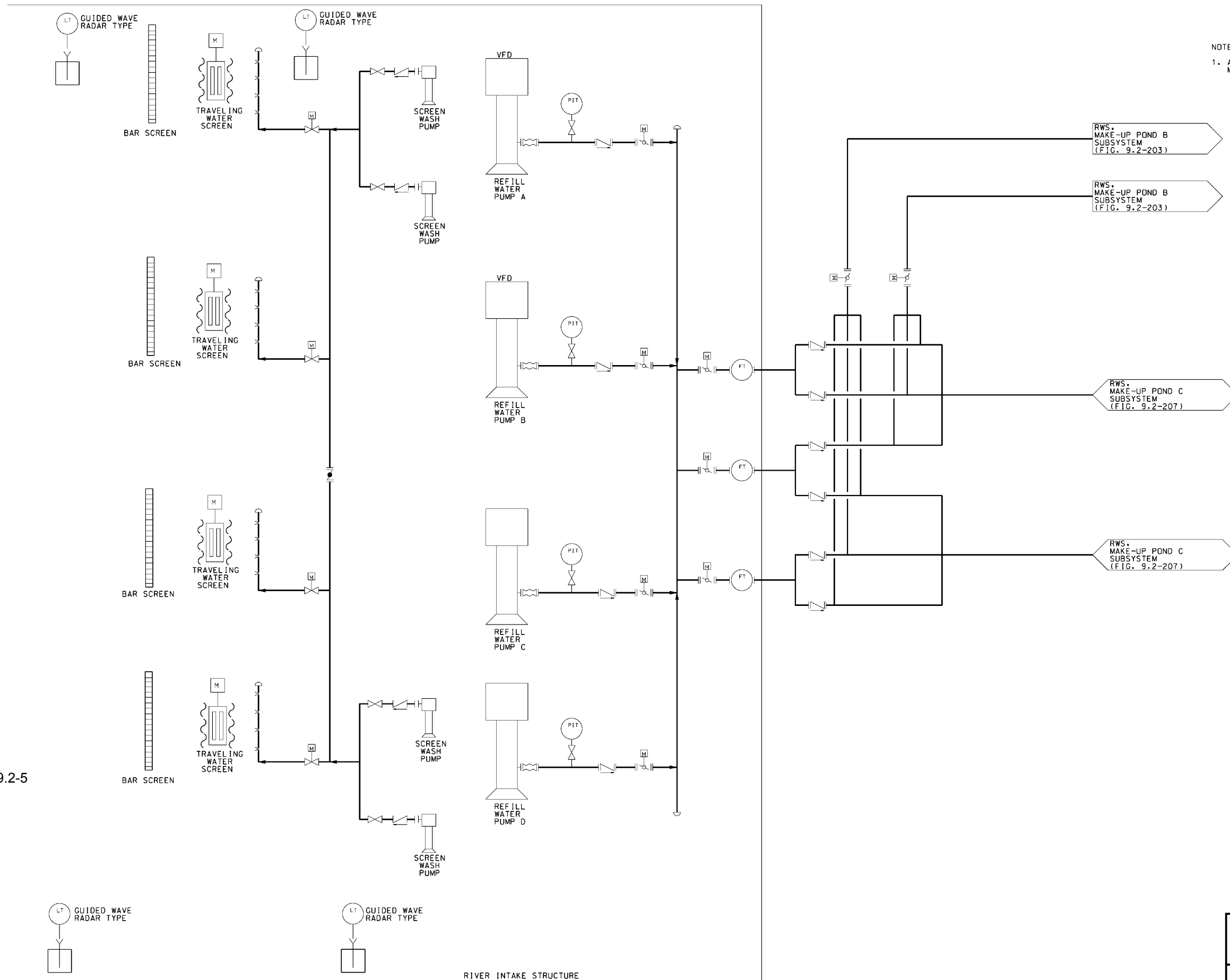
WILLIAM STATES LEE III NUCLEAR STATION UNITS 1 & 2 Raw Water System, Refill Subsystem FIGURE 9.2-206 Rev 2
