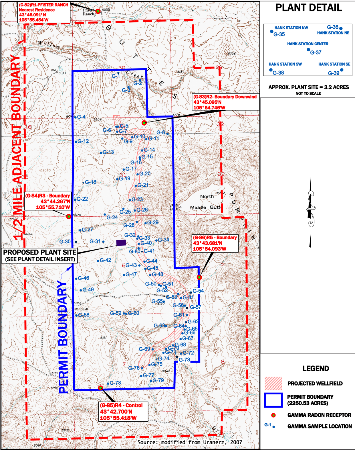
Figure 6-4. Hank Unit Radon, Gamma, and Air Particulate Monitoring Locations
