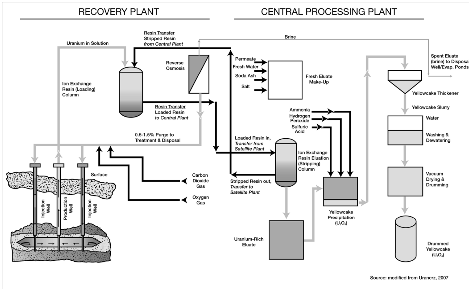
Figure 2-11. General Flow Schematic for the ISR Process
