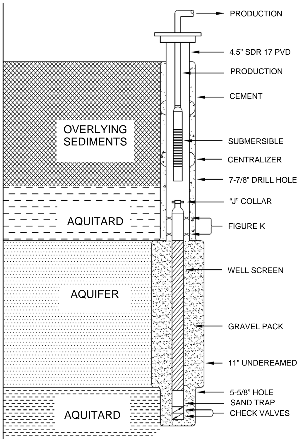
Figure 2-9. Production Well Construction
