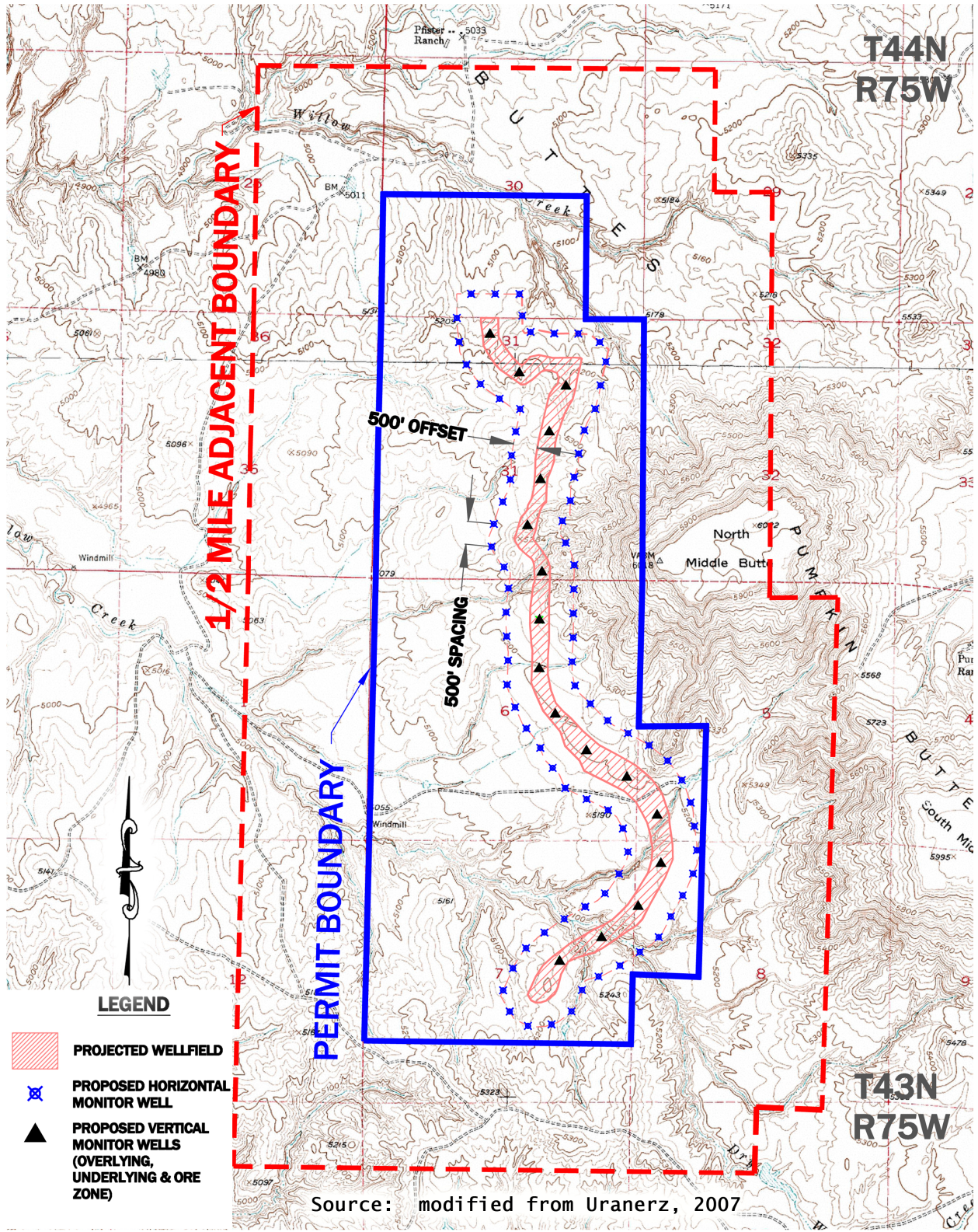
Figure 6-9. Hank Unit Monitoring Well Locations
