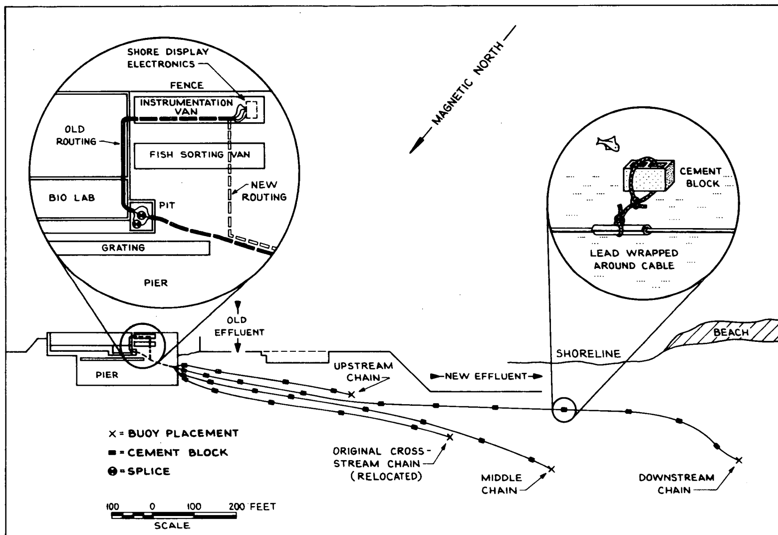
Figure 5-15. Cable Routing Diagram for Thermal Chains
