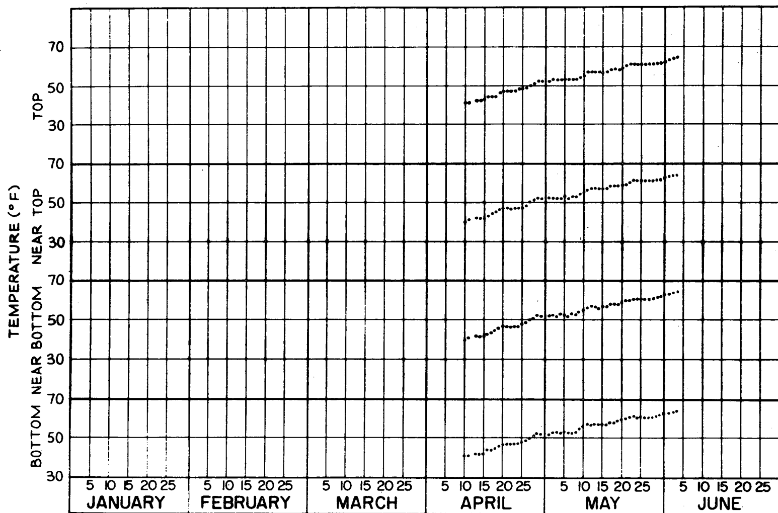
Figure 6-6. Thermal Chain 0800 Data—Middle Buoy—1970
