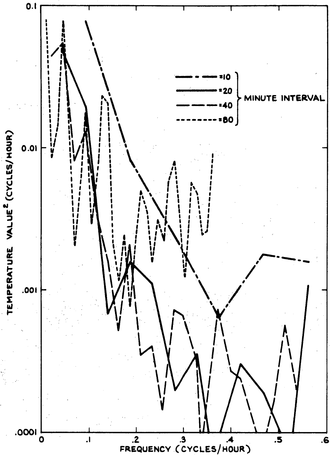
Figure 6-14. Spectral Analysis of Thermal Chain Data from Downstream Buoy Surface Sensor—27 May—2 June 1970, Data Points Constant
