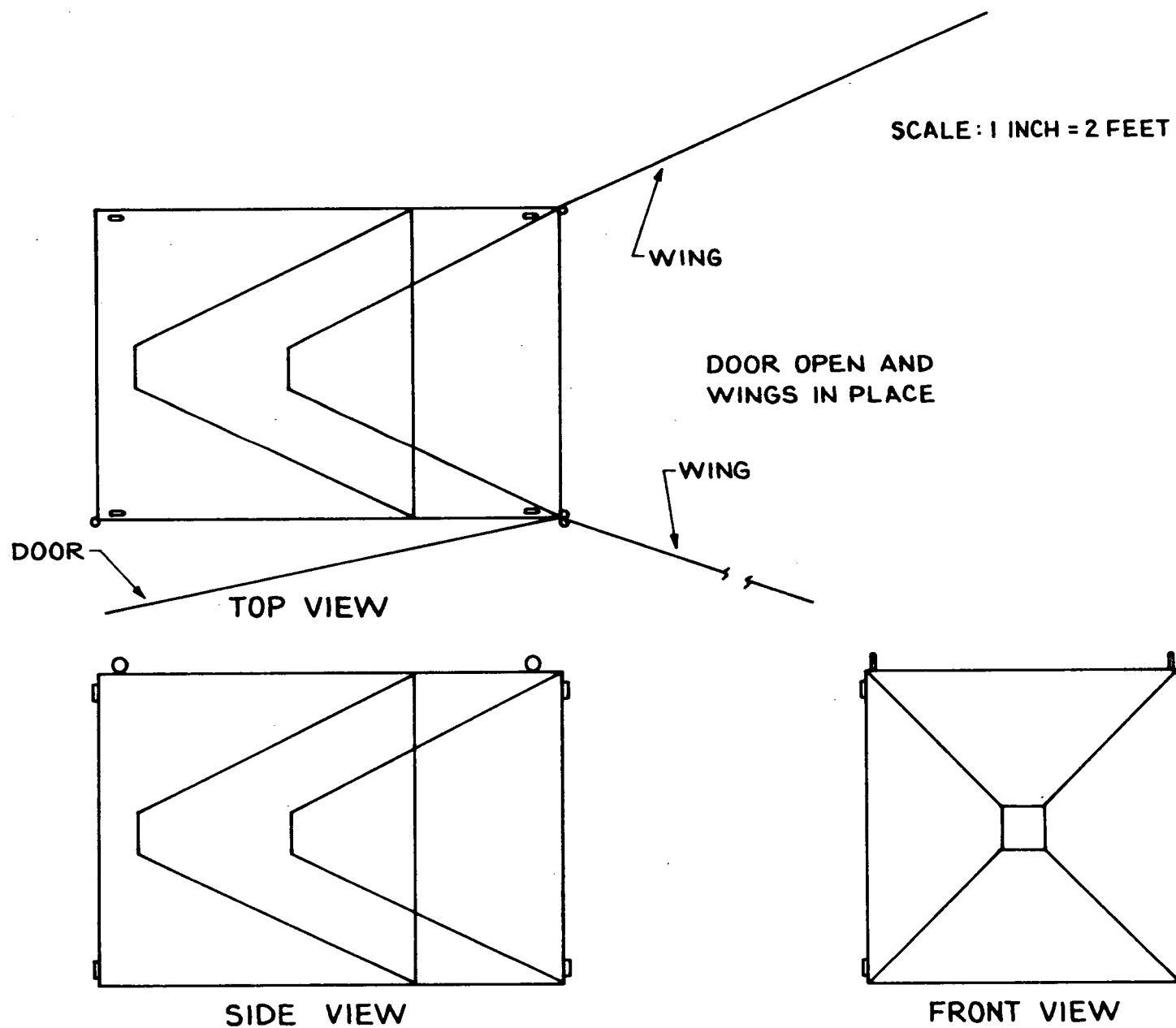
Figure 10-2. Indian Point Fish Trap
