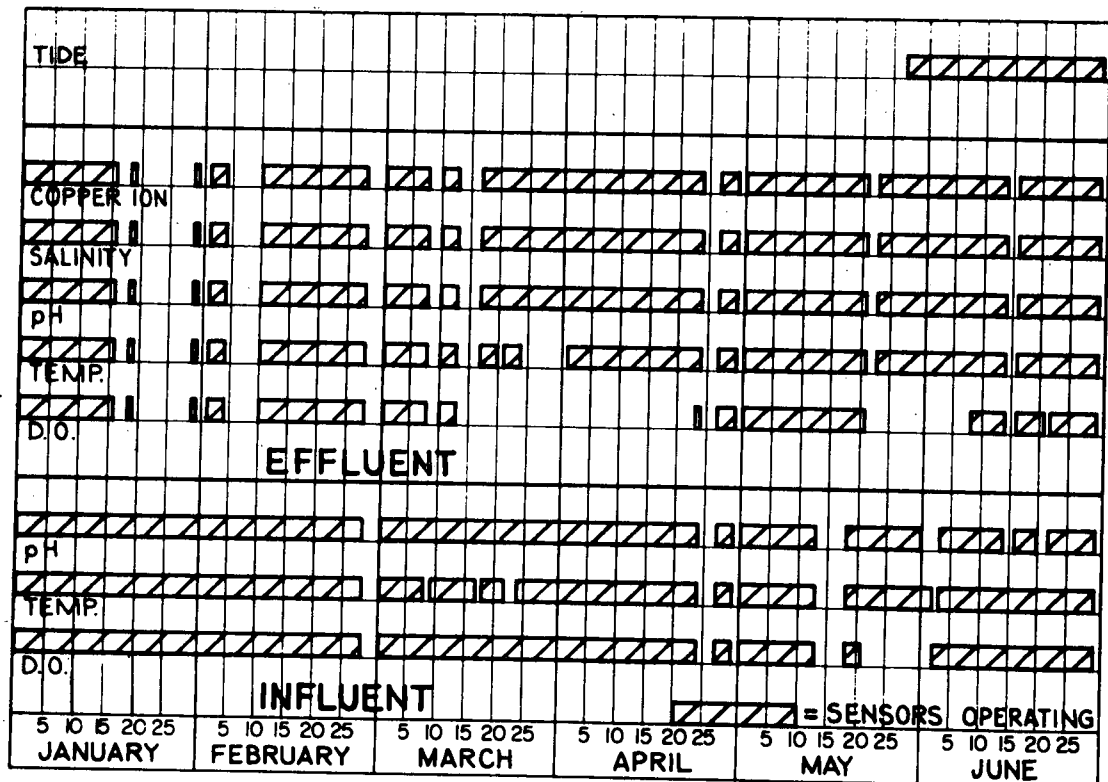
Figure 5-2. Automated Environmental System (AES) Operational History - 1970
