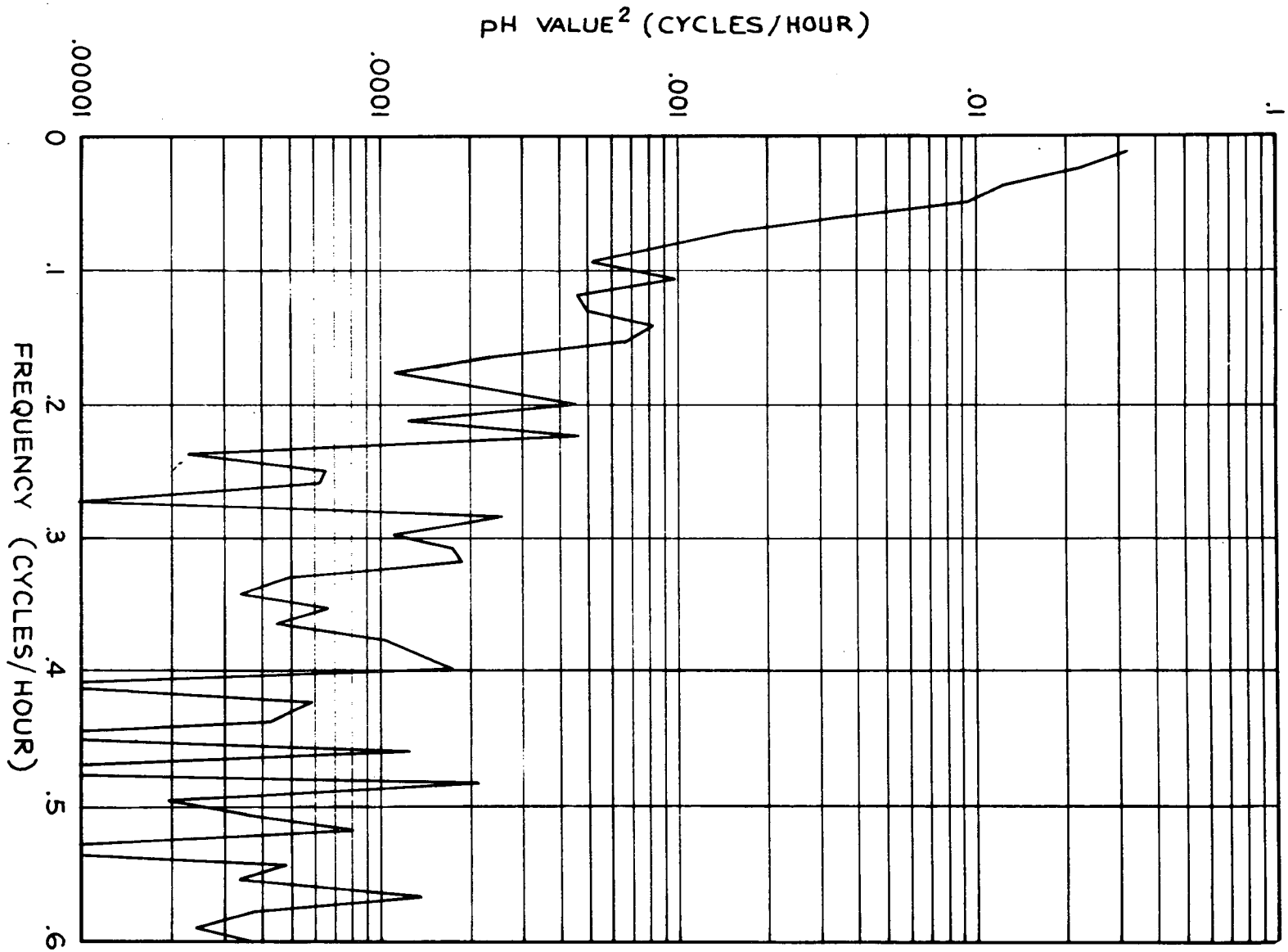
Figure 7-6. Spectral Analysis of Intake pH—June 19-22, 1970
