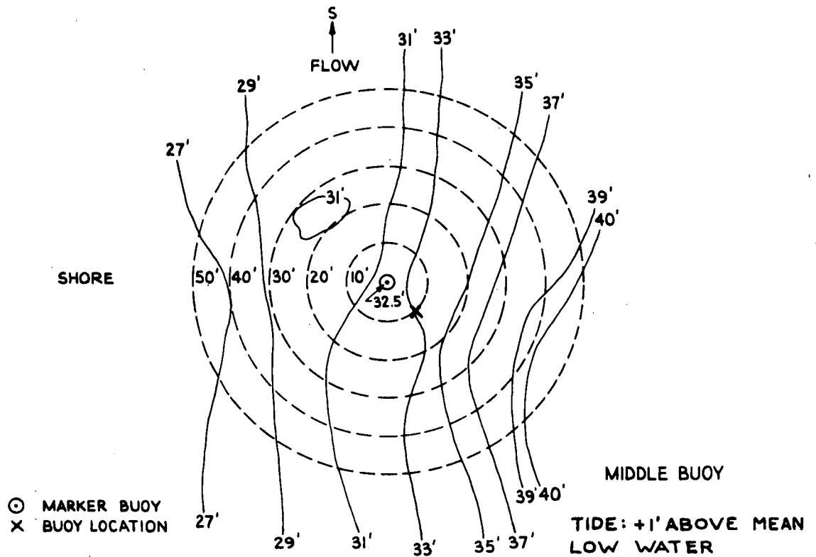
Figure 5-11. Middle Buoy — Bottom Profile
