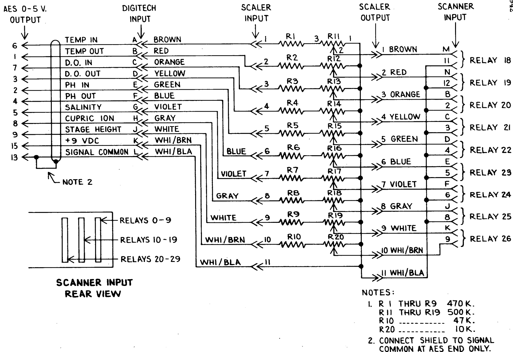
Figure 5-5. AES/Digitech Interface
