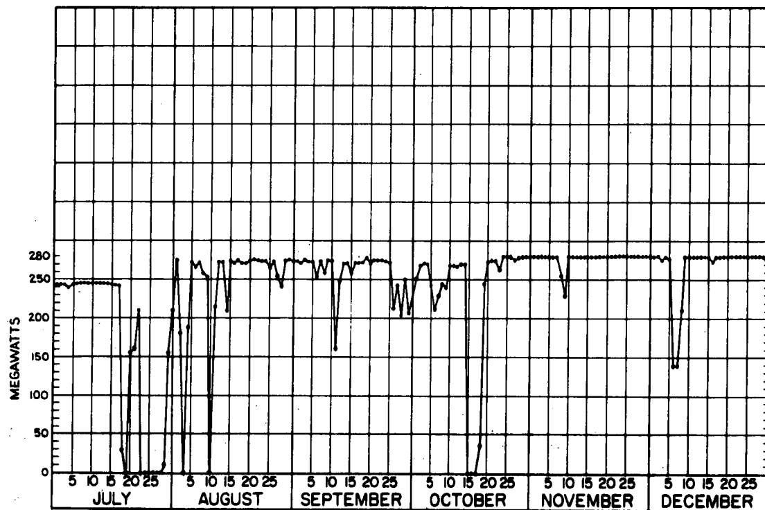
Figure 5-7. Average Daily Output, Indian Point - Unit One
