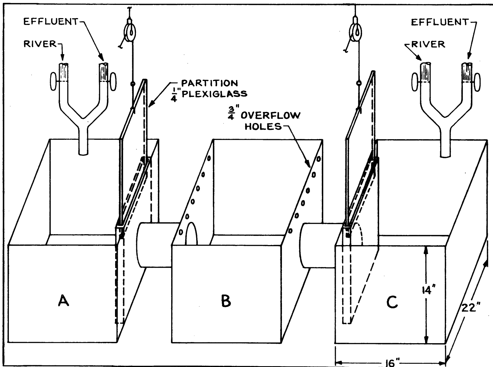
Figure 11-2. Large Thermal Effluent Choice Apparatus
