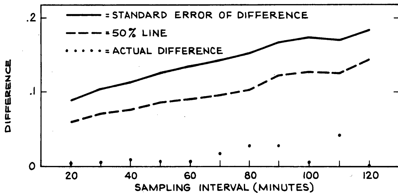
Figure 6-12. Standard Error of Difference of the Mean for Different Sampling Intervals
