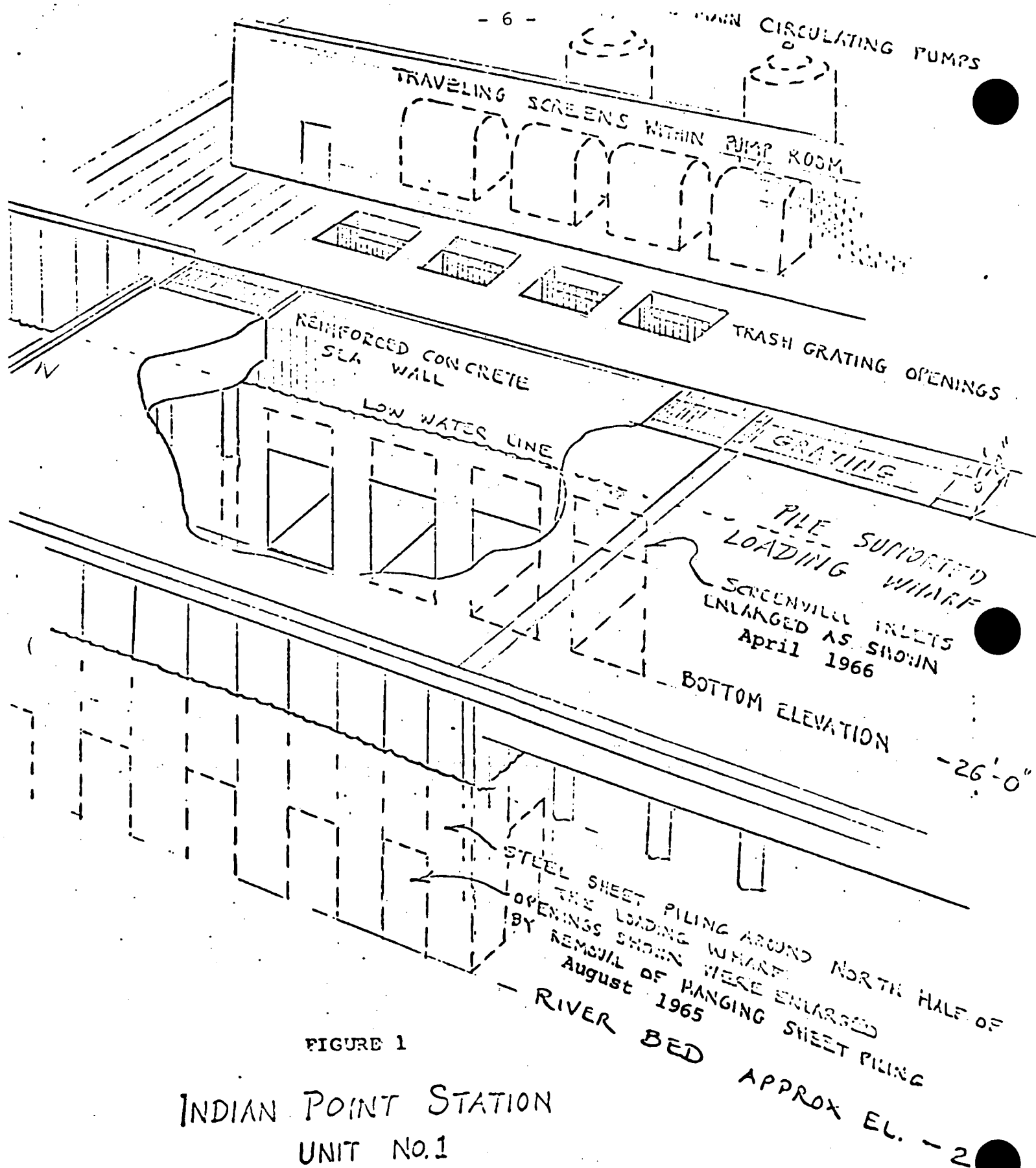
COOLING WATER INTAKE CONFIGURATION
