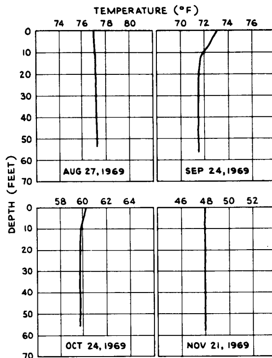
Figure 5-4. Overflight Bathythermograph Profiles Vicinity of Stony Point (Channel Between Stations 15 and 9), Ebb Tide
