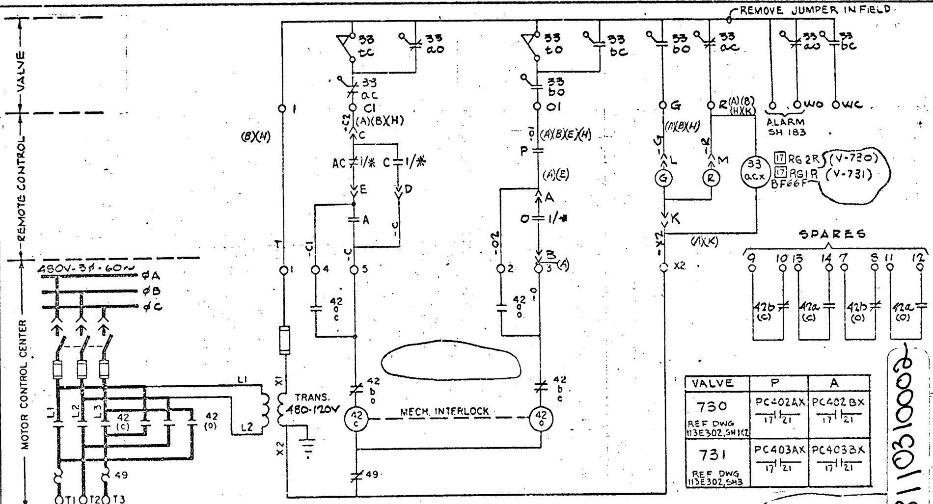
AUTO CLOSE - PERMISSIVE TO OPEN FIGURE #10
