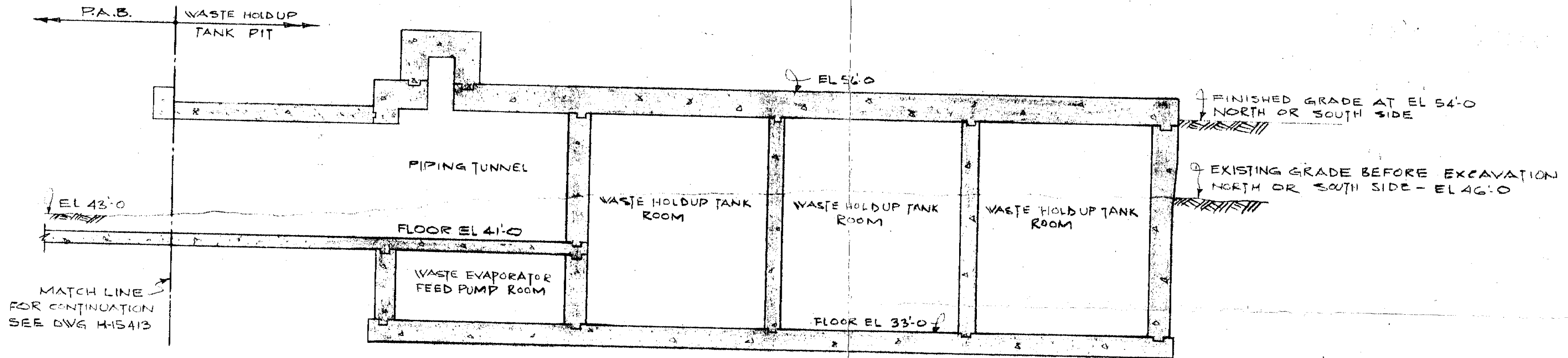
WASTE HOLDUP TANK PIT SECTION LOOKING NORTH SCALE 1/8" = 1'-0"
