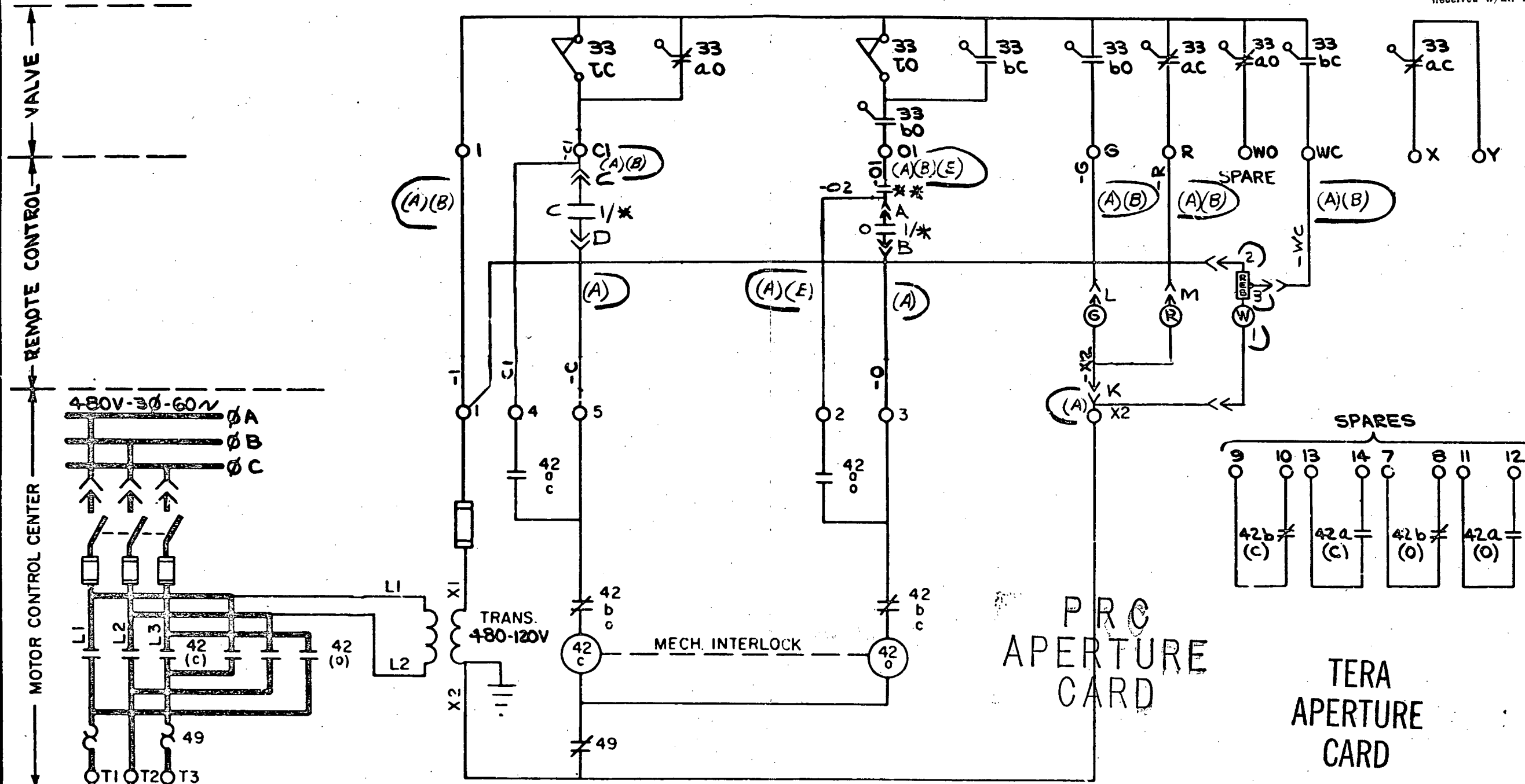
MANUAL OPERATED (PERMISSIVE TO OPEN) MONITOR LIGHT-CLOSED FIGURE # 4
