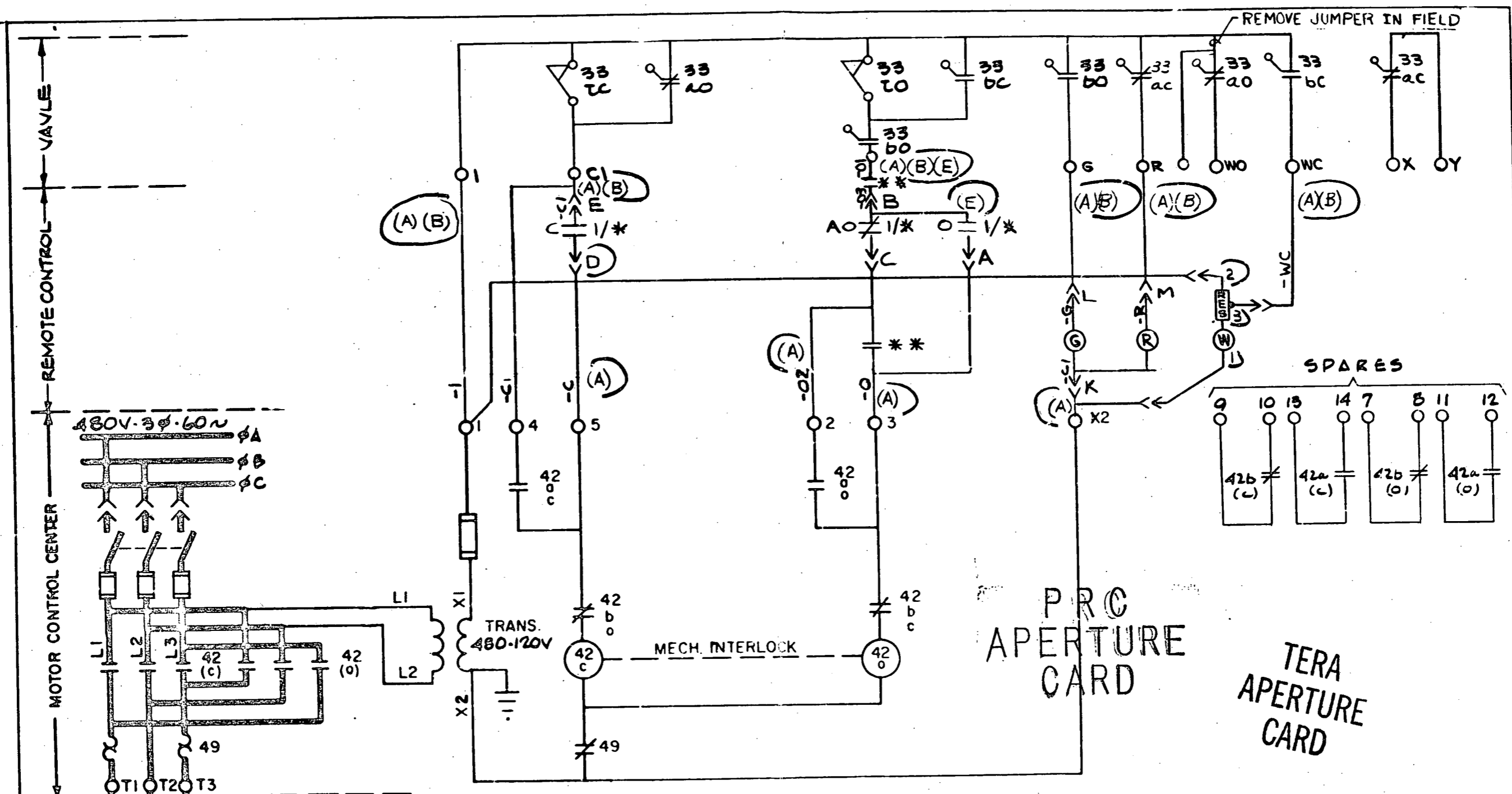
AUTO OPEN (PERMISSIVE TO OPEN) MONITOR LIGHT-CLOSED VALUE SHOWN IN FULL OPEN POSITION FIGURE # 3
