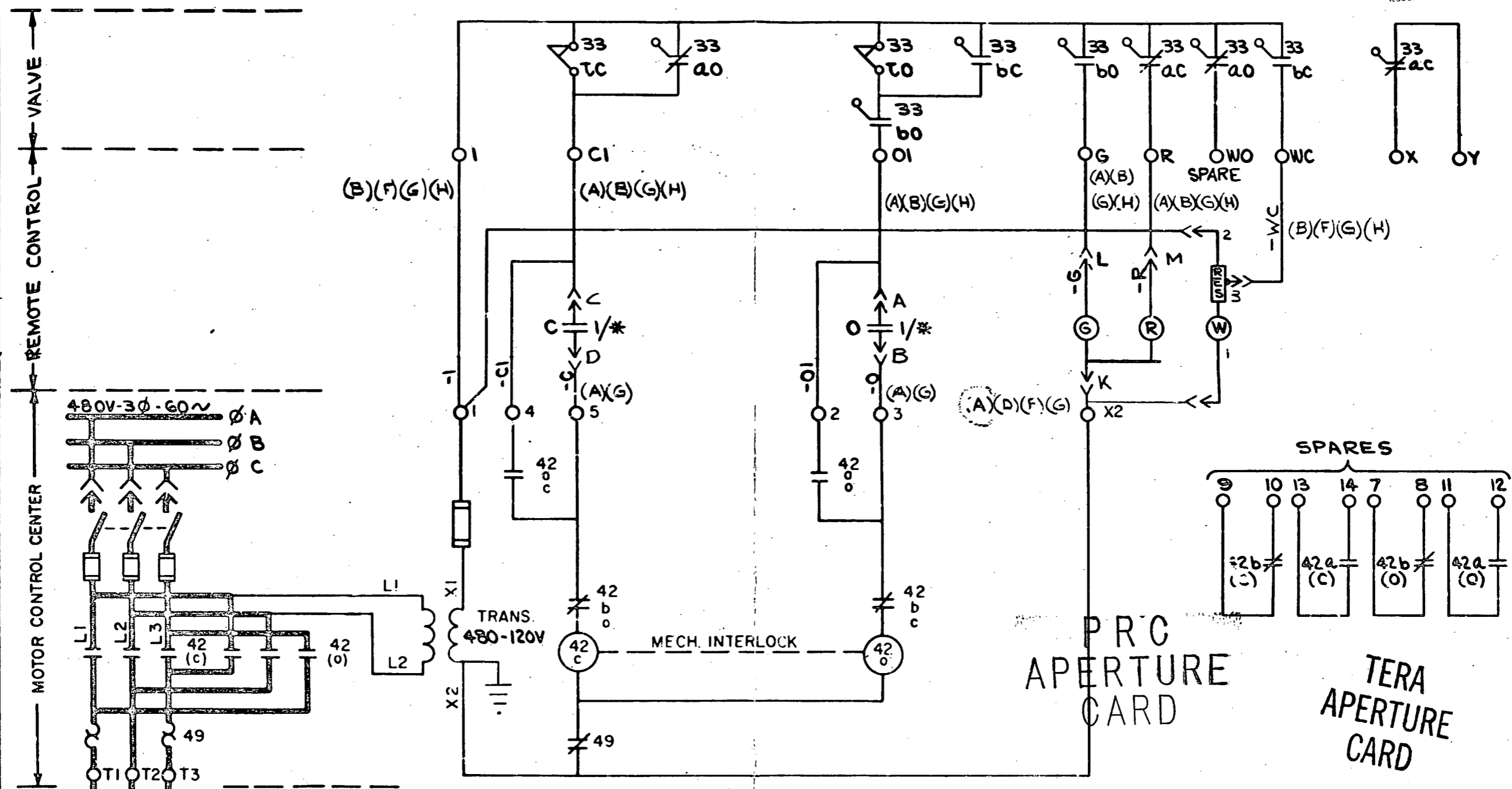
MANUAL OPERATED (SAFEGUARDS) MONITOR LIGHT - CLOSED FIGURE # 2 VALVE SHOWN IN FULL OPEN POSITION
