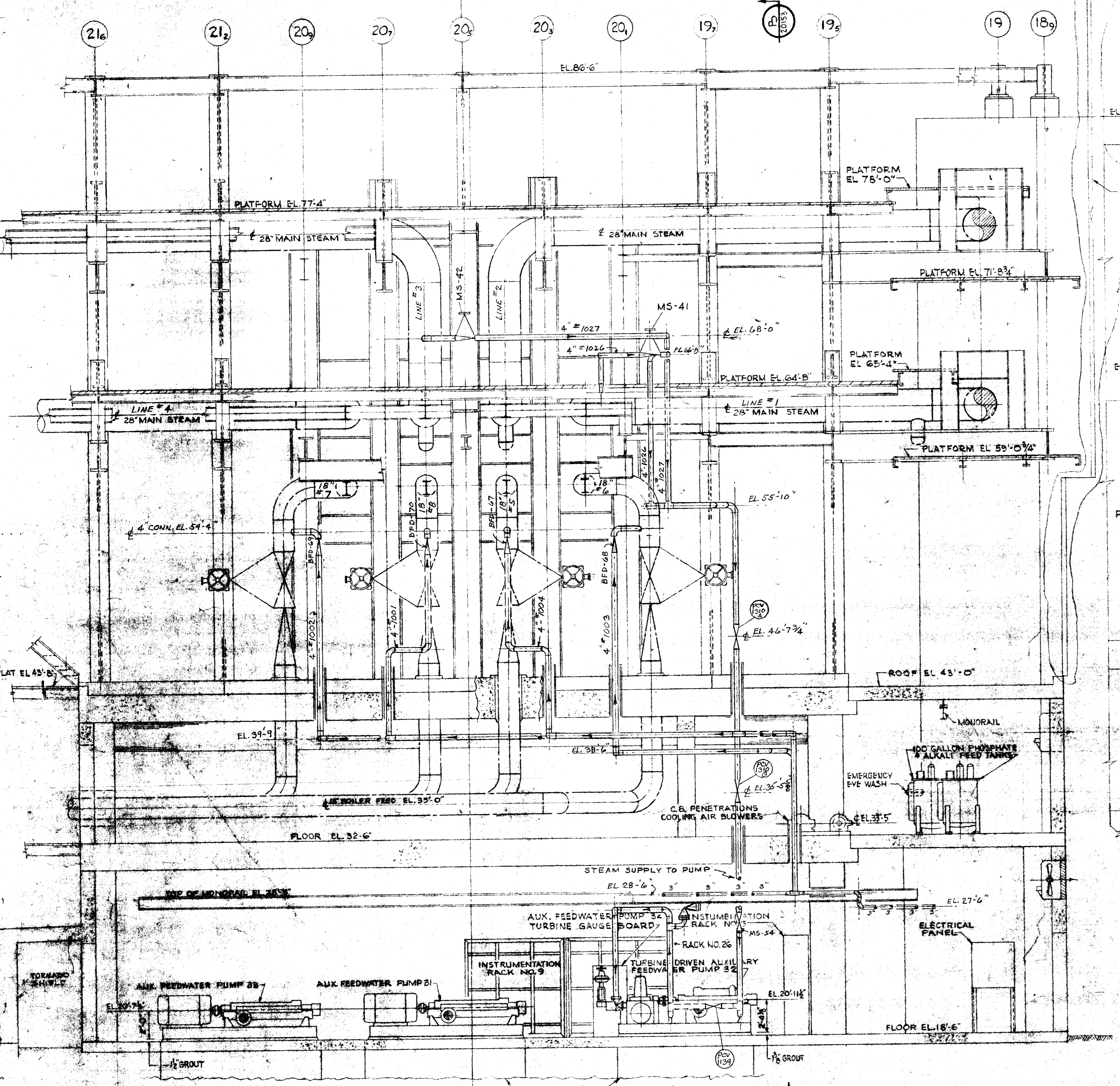
SECTION A-A SCALE 1/4" = 1'-0" SEE DWG. 9321-F-20143
