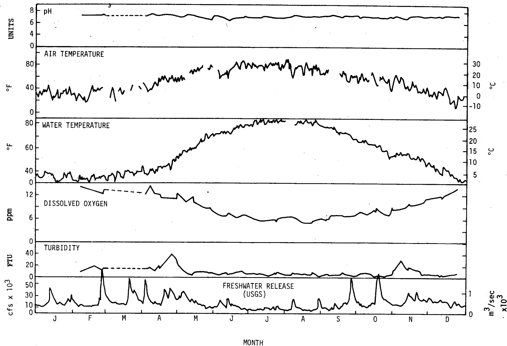
Figure III-12. Seasonal Variation of Water Temperature, pH, Dissolved Oxygen Concentration, Turbidity, and Air Temperature with Freshwater Flow in Hudson River at Indian Point. (Water temperatures from TI impingement study; pH and dissolved oxygen values [mid-depth] and turbidity values [surface] measured weekly at standard-station 4)
