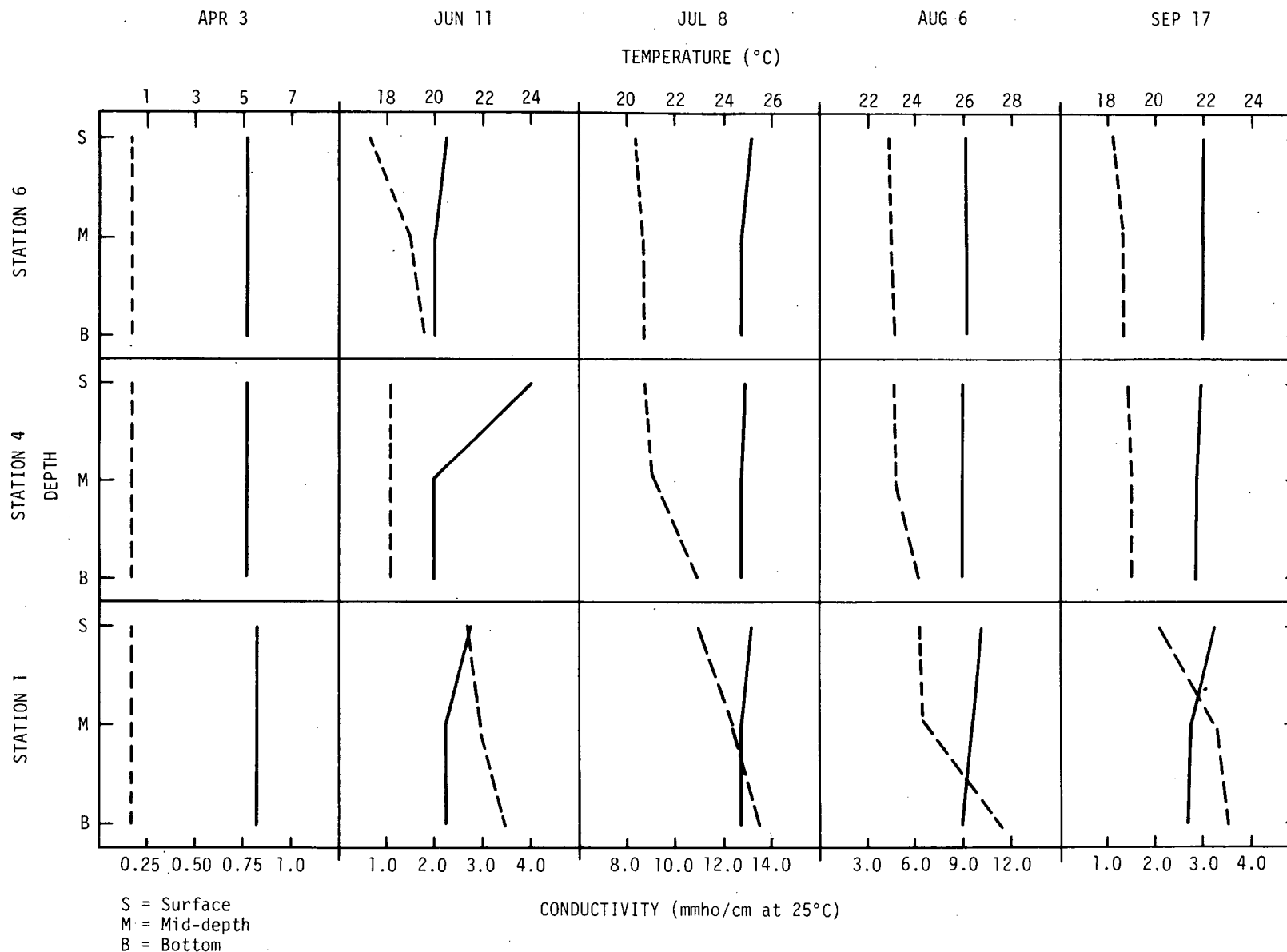
Figure III-11. Vertical Profiles of Temperature (—) and Conductivity (----) in Indian Point Region Determined from Surface, Middle, and Bottom Measurements at Standard Stations 1, 4, and 6 on Selected Days during 1975
