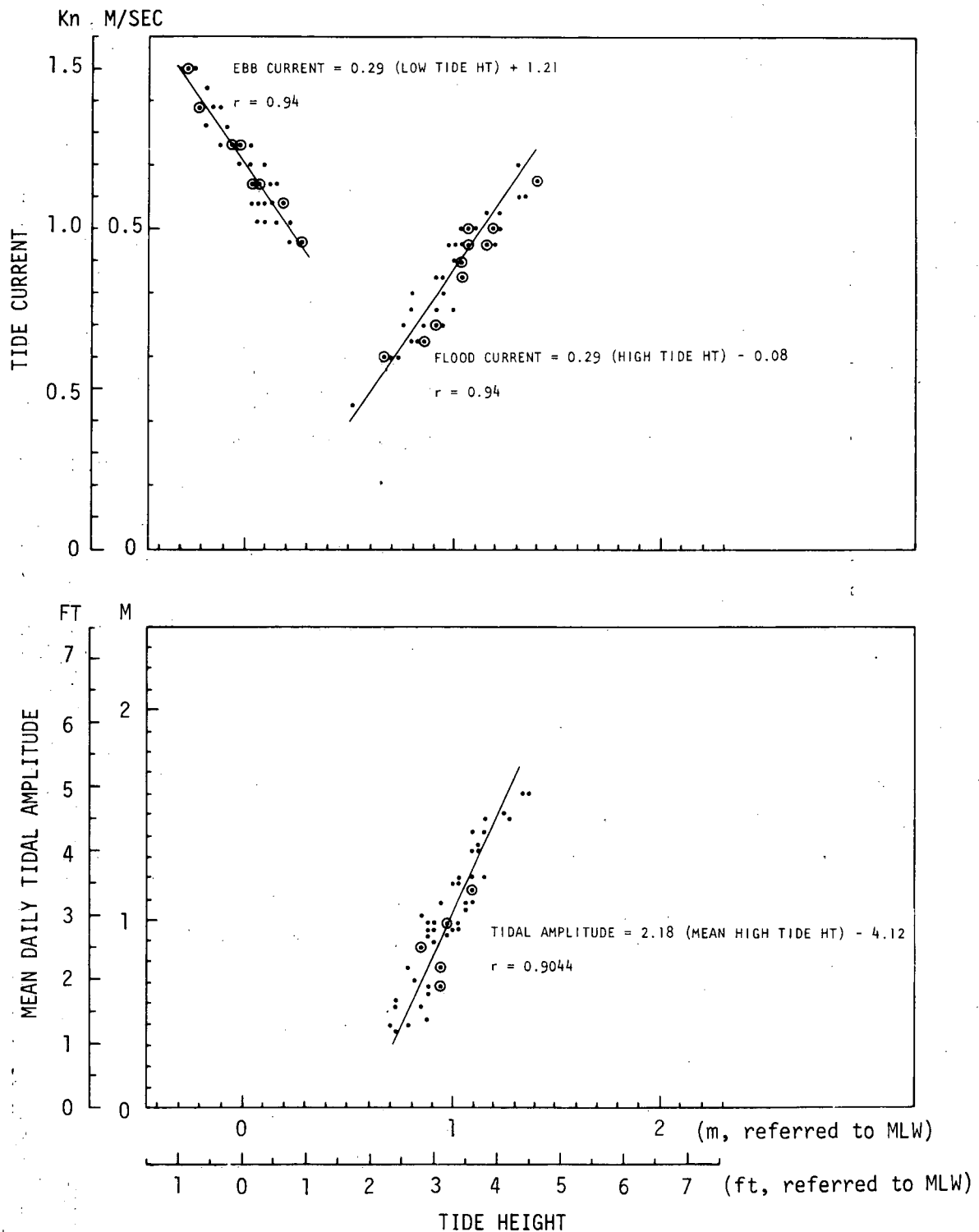
Figure III-4. Relationship among Tidal Elevations, Amplitudes, and Currents in Hudson River at Peekskill, New York, as Described by Regression Analysis. (Data from USGS prediction tables for 1973)
