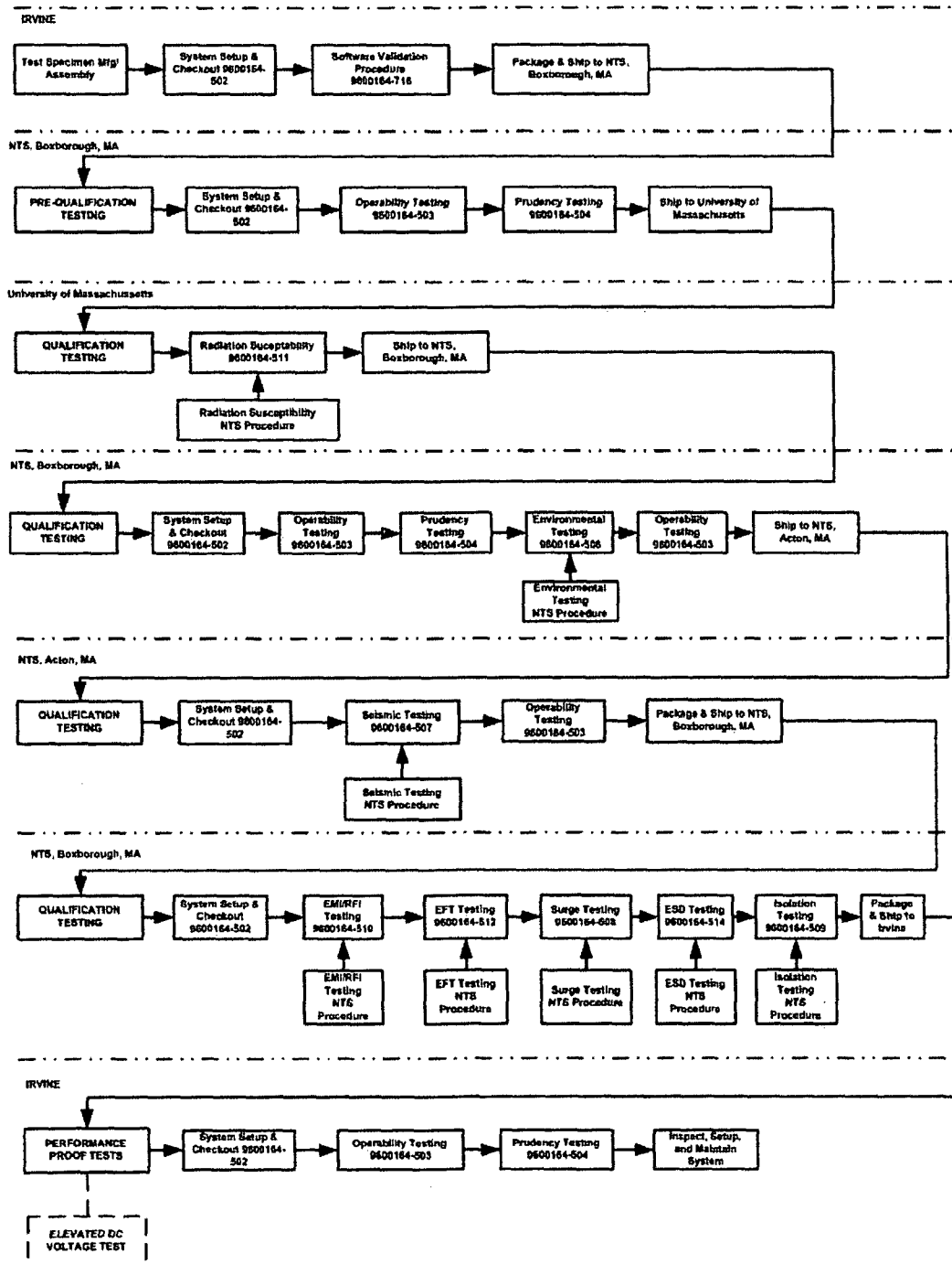
FIGURE 2- MASTER TEST PLAN – FLOW DIAGRAM
