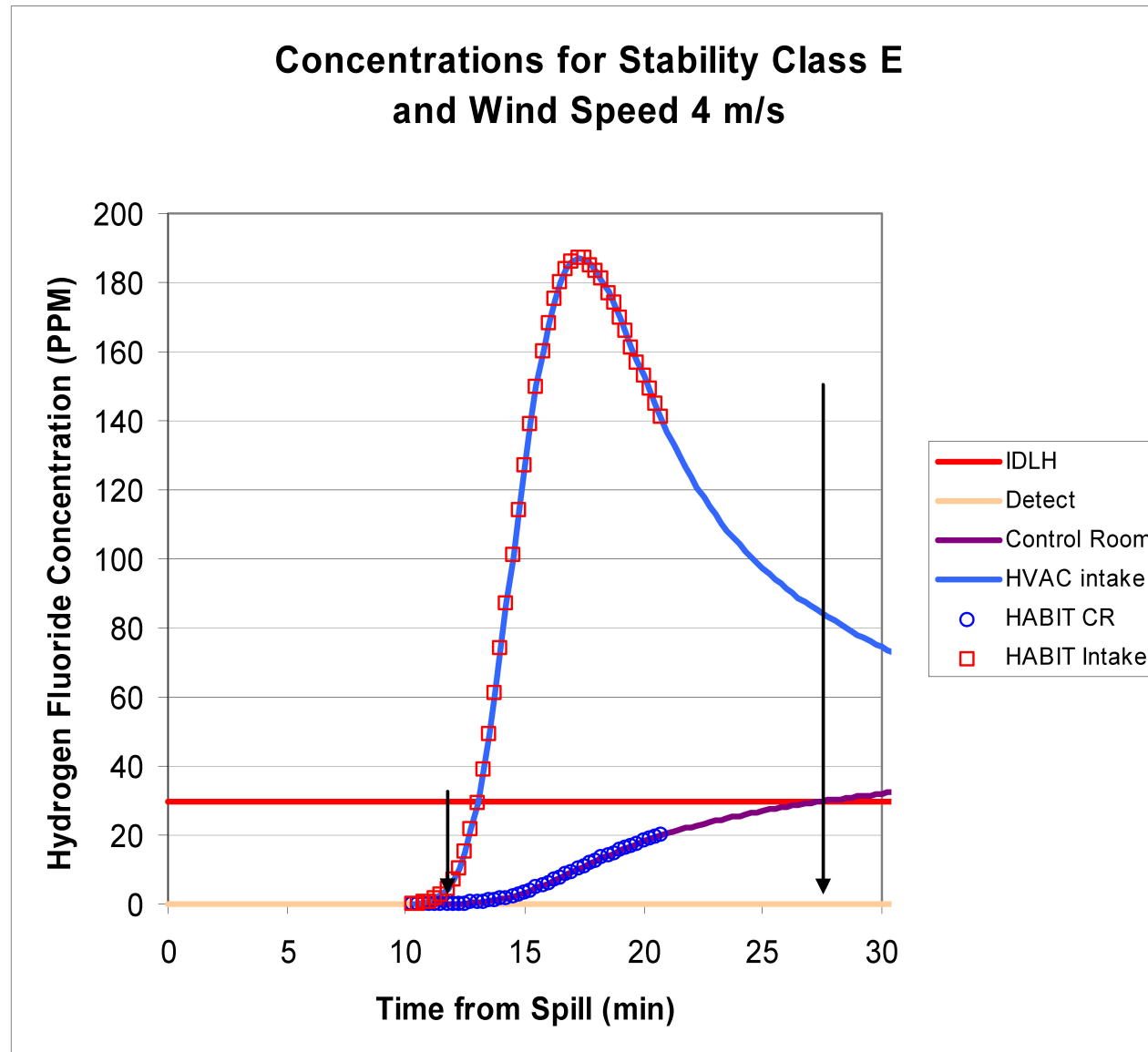
FIGURE 6.4-202 Hydrogen Fluoride Concentrations at the Control Room HVAC Intake and Inside the Control Room for Stability Class E and the Wind Speed of 4 m/sec case
