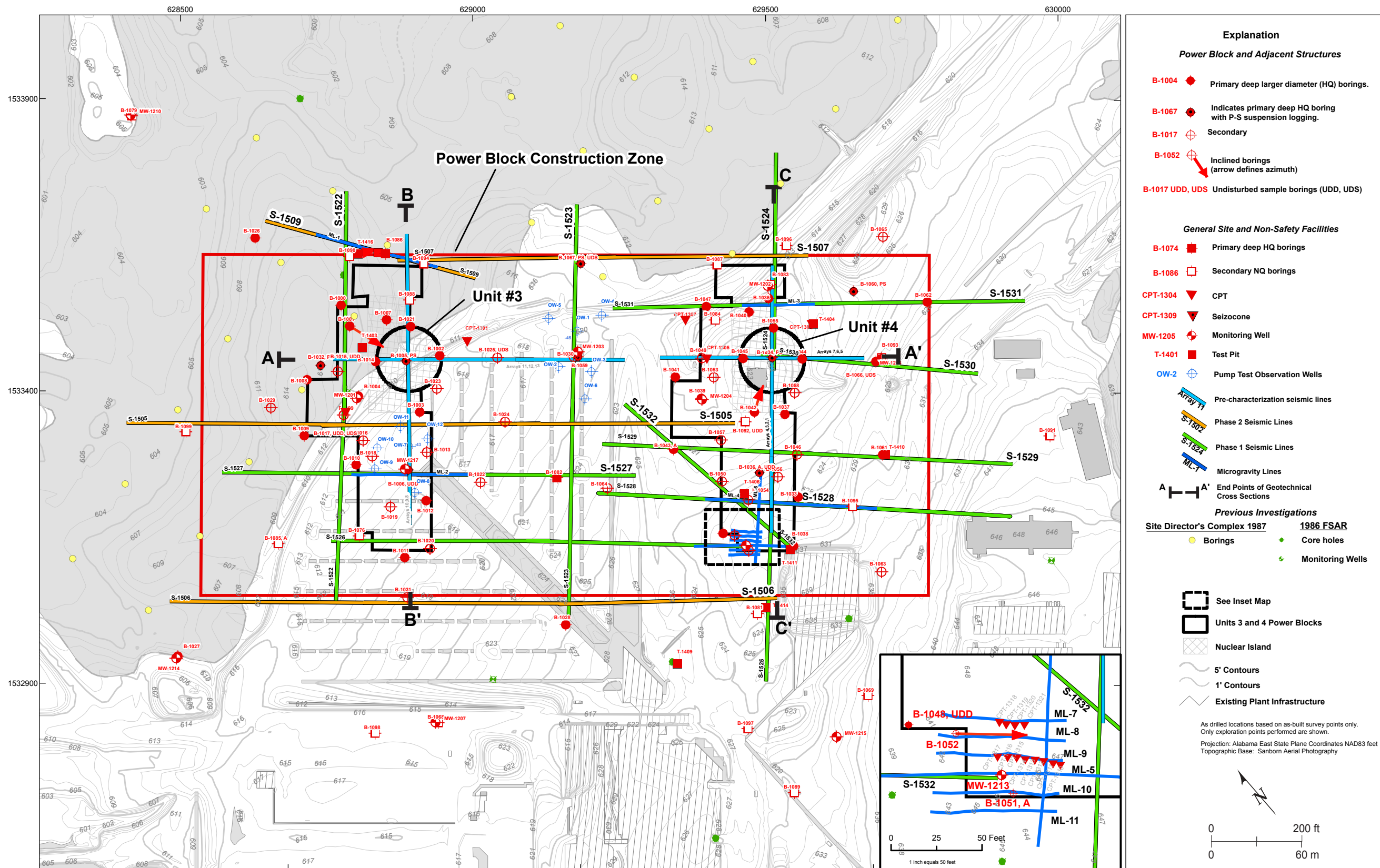
FIGURE 2.5-324 Exploration Program, BLN Power Block Construction Zone (with Cross Section Locations)
