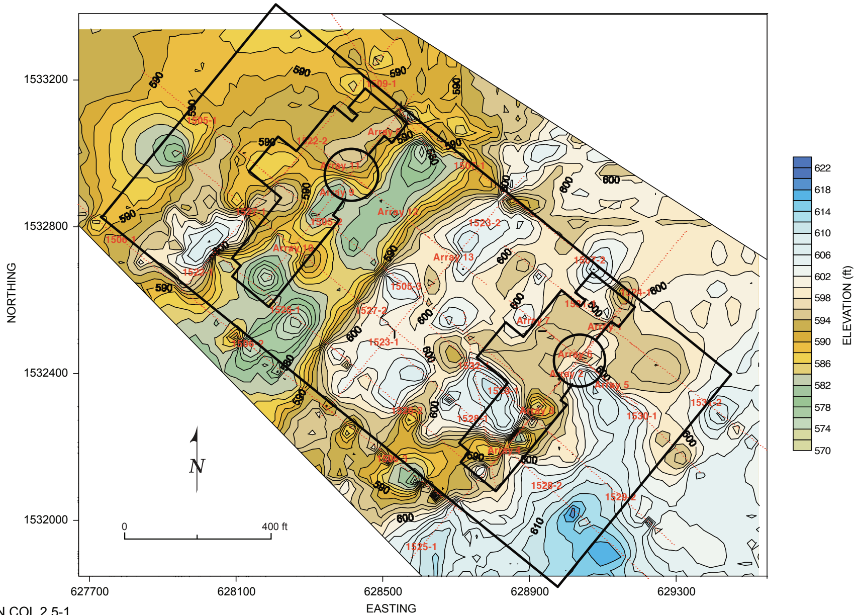
FIGURE 2.5-313 Seismic 3D Model: Top of 14,000 fps Vp Layer
