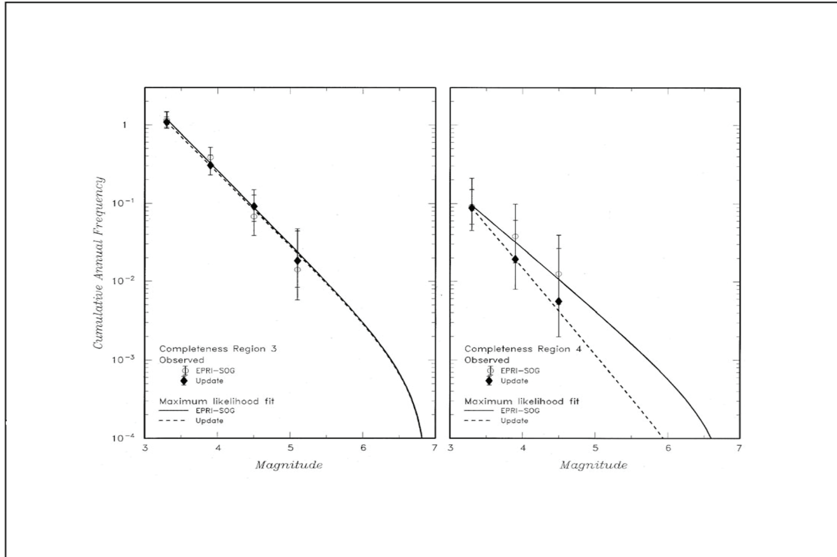
FIGURE 2.5-248 Earthquake Recurrence Rates Estimated for the “Equivalent Period of Completeness” for the Portions of EPRI-SOG Completeness Regions 3 and 4 within 200 Miles of the Bellefonte Site
