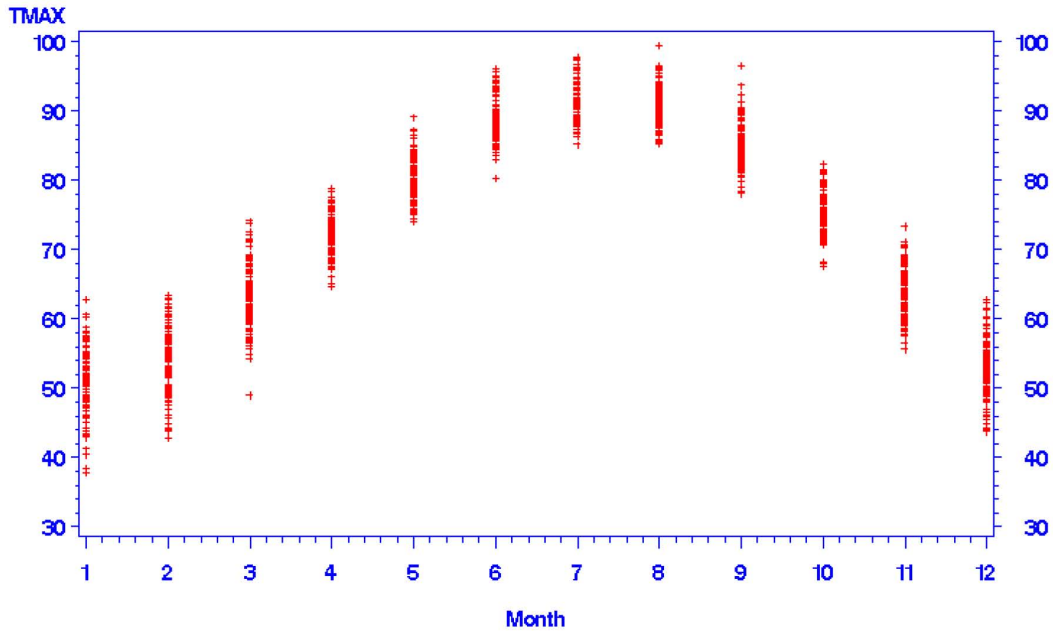
USHCN 017304, SCOTTSBORO, AL Monthly mean maximum temperature (F) 1882 – 2002
