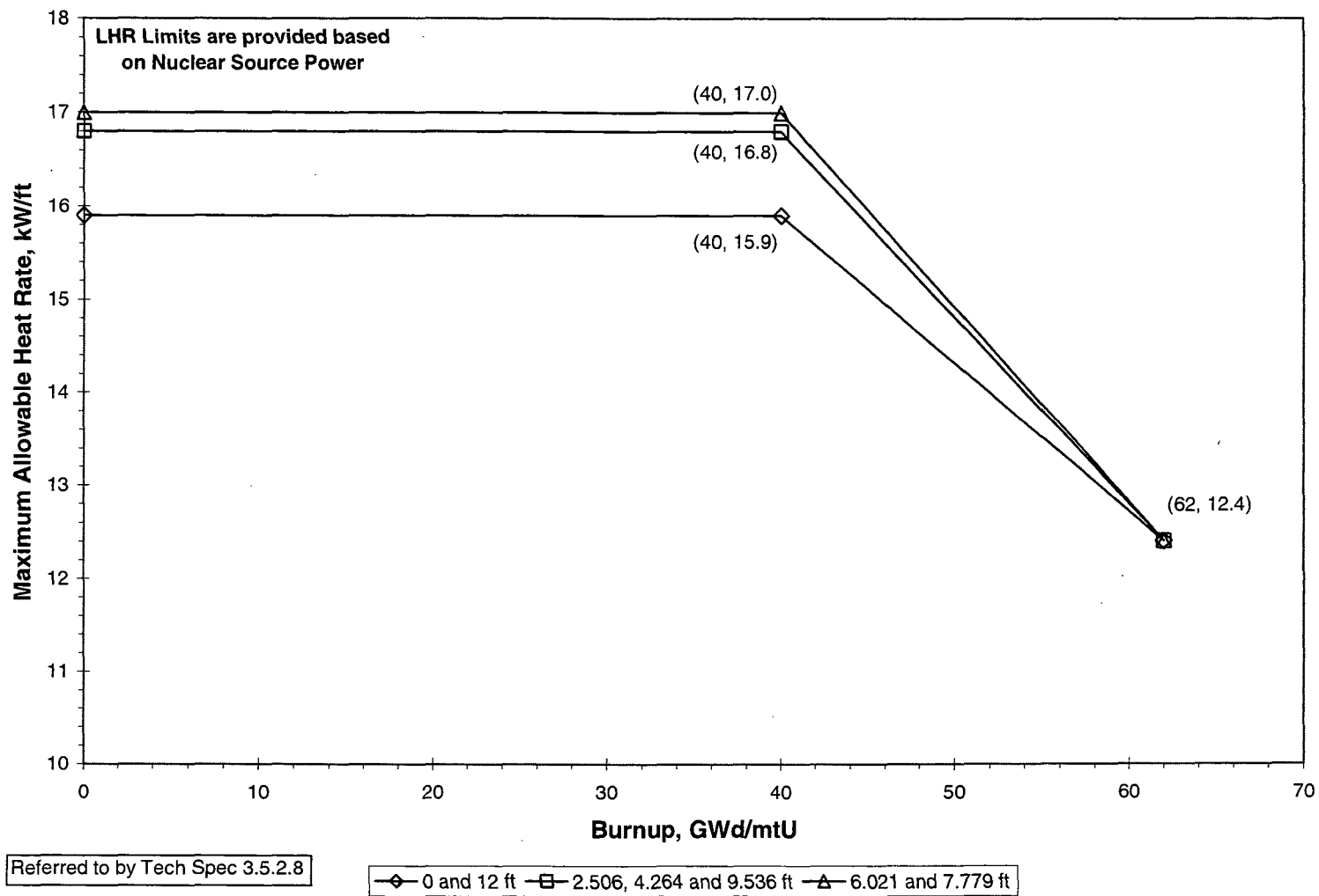
Figure 9 (Page 1 of 5) LOCA Limited Maximum Allowable Linear Heat Rates Mark-B12 Fuel Assemblies (UO 2 Fuel Rods)
