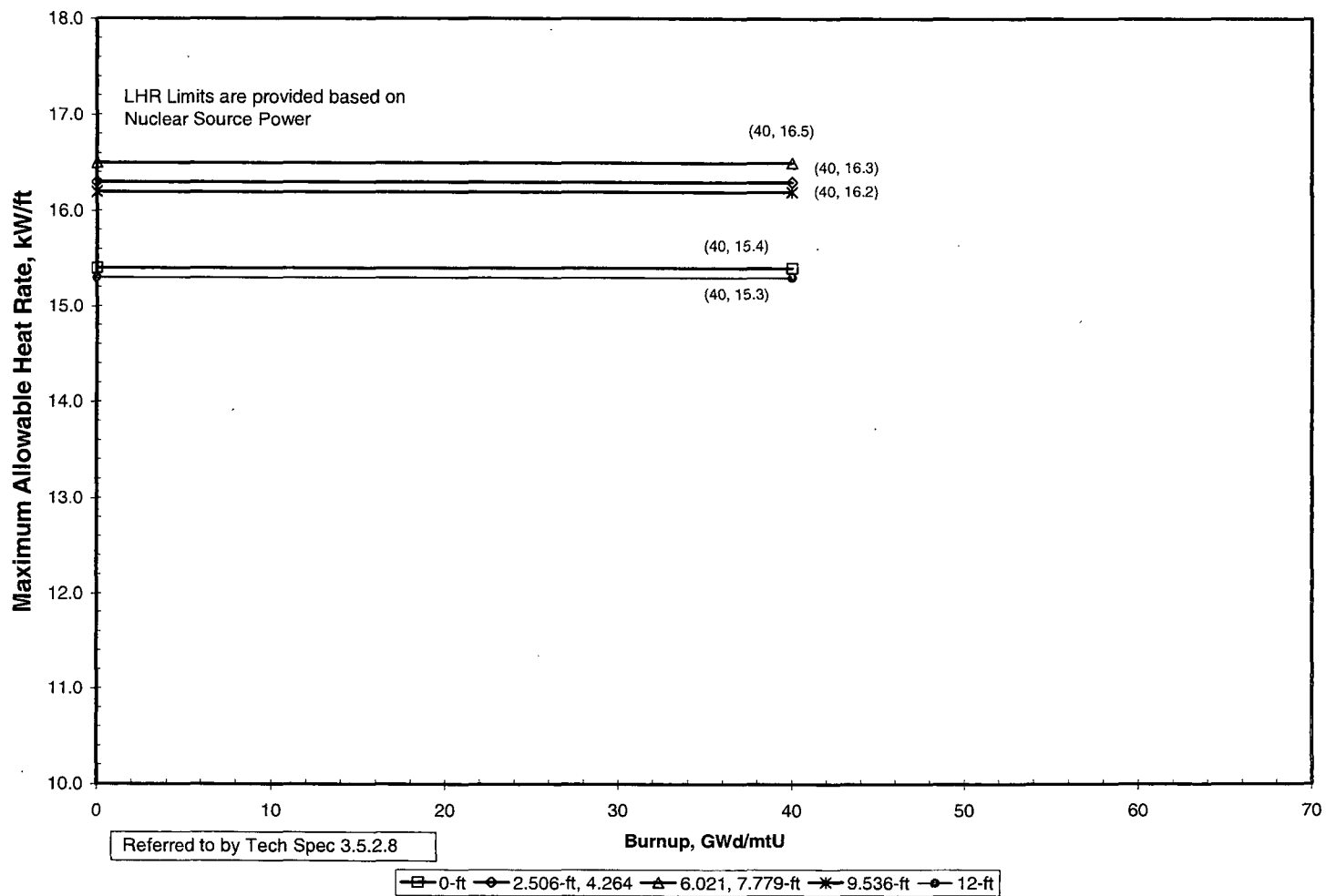
Figure 9 (Page 3 of 5) LOCA Limited Maximum Allowable Linear Heat Rates Mark-B-HTP Fuel Assemblies, Batch 20A (UO 2 Fuel Rods)
