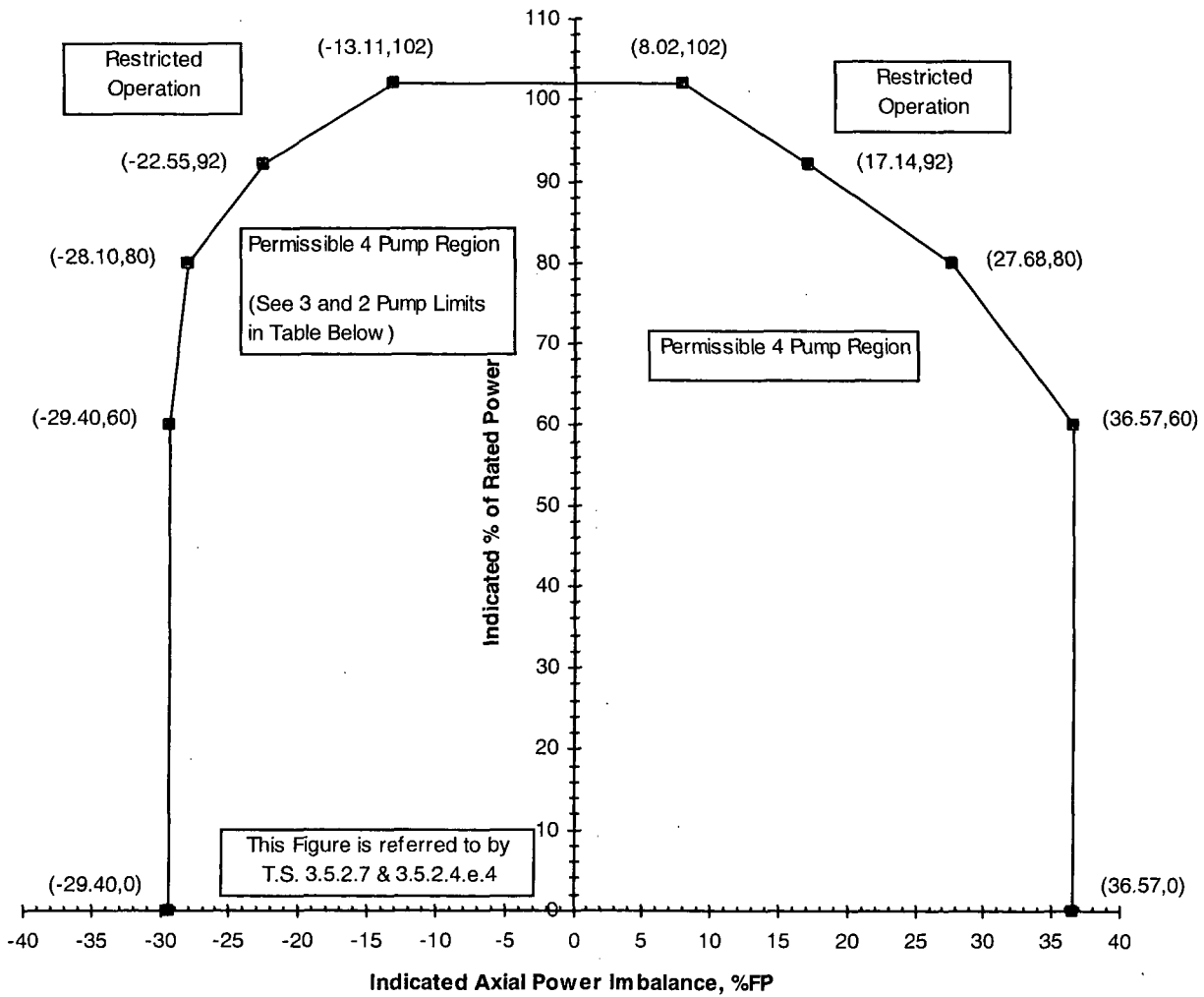
Figure 8 Minimum Incore System Error Adjusted Imbalance Limits (0 EFPD to EOC)
