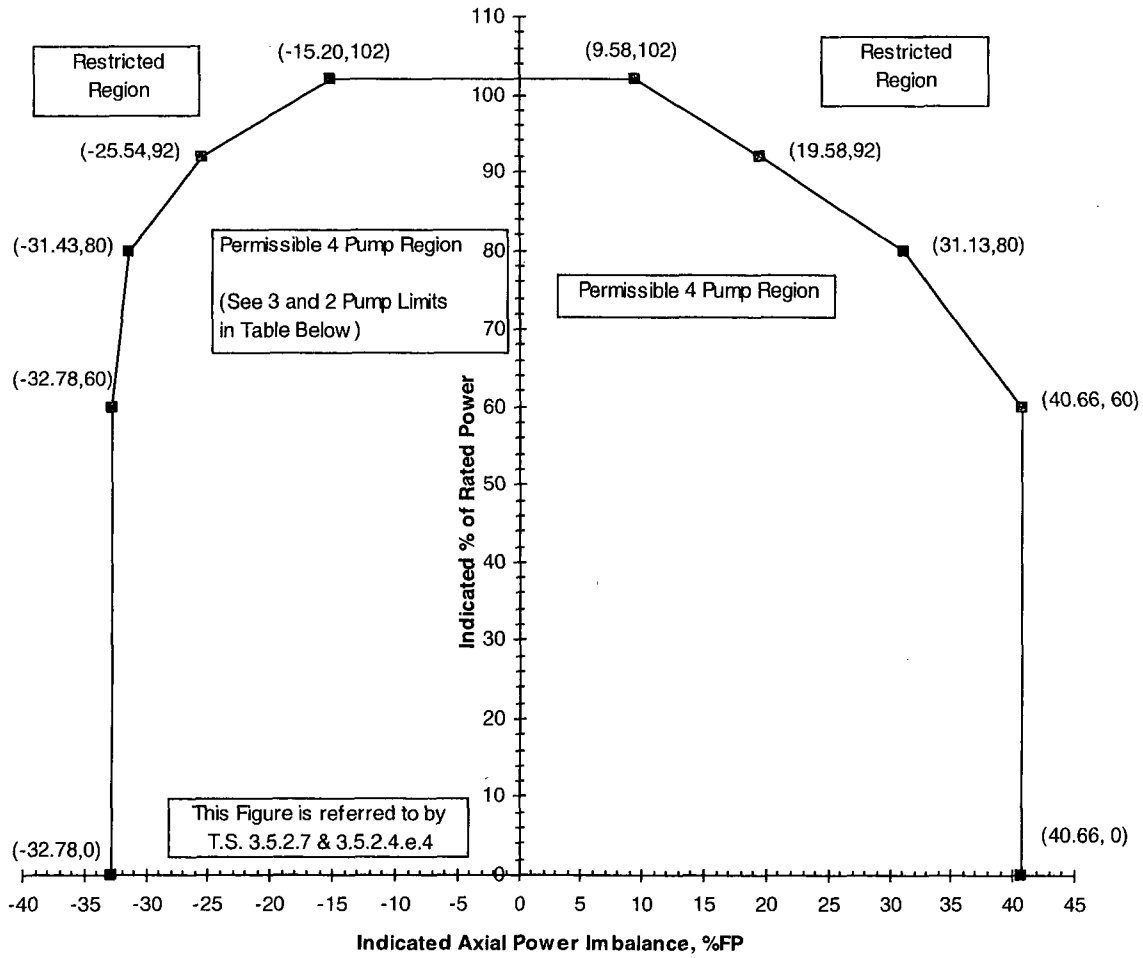
Figure 7 Out-of-Core Detector System Error Adjusted Imbalance Limits (0 EFPD to EOC)
