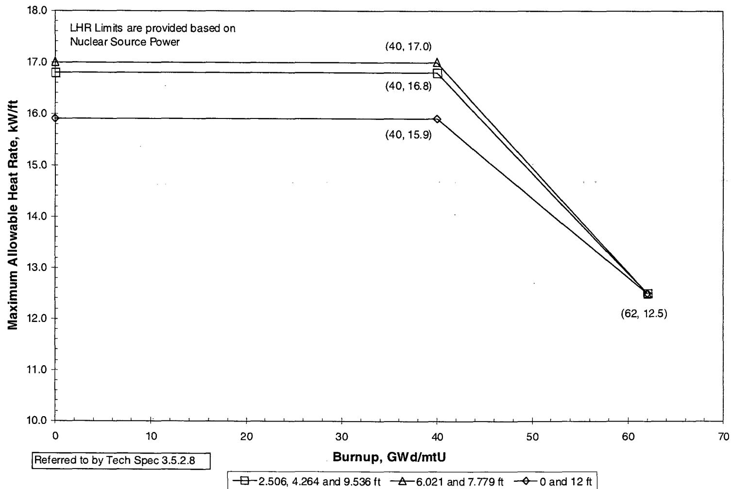
Figure 9 (Page 2 of 5) LOCA Limited Maximum Allowable Linear Heat Rates Mark-B-HTP Fuel Assemblies, Except Batches 20A and 20B (UO 2 Fuel Rods)
