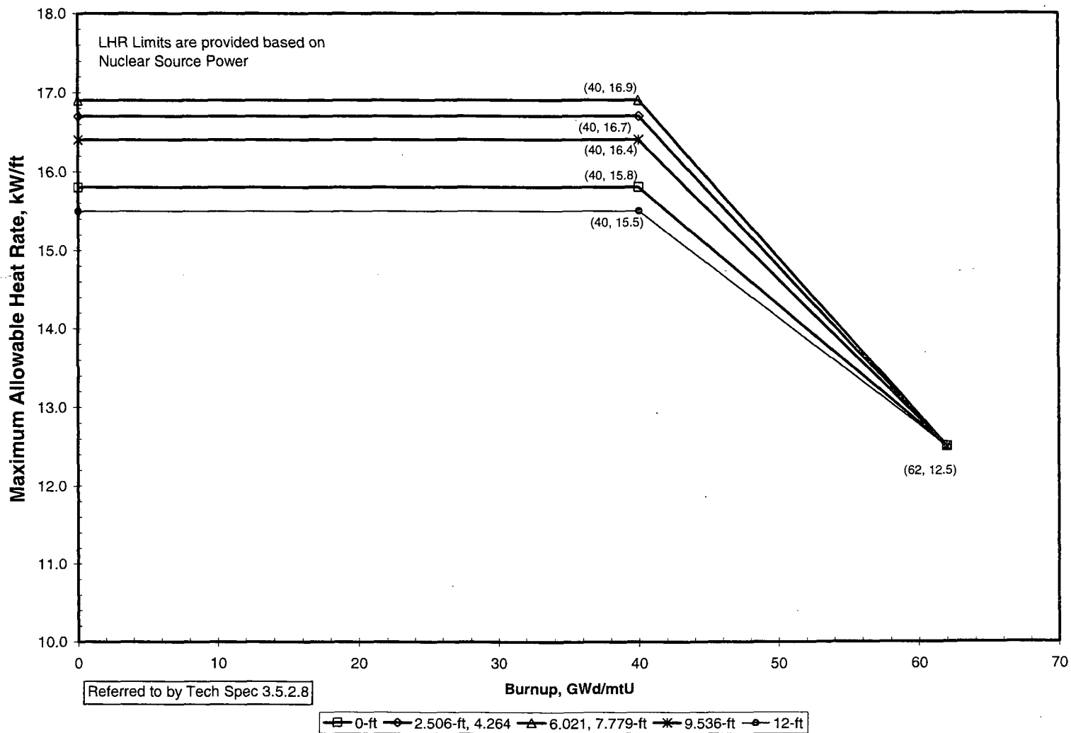
Figure 9 (Page 4 of 5) LOCA Limited Maximum Allowable Linear Heat Rates Mark-B-HTP Fuel Assemblies, Batch 20B (UO 2 Fuel Rods)
