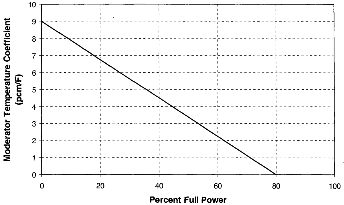
Figure 9 (Page 5 of 5) MTC Limit vs. Power Level
