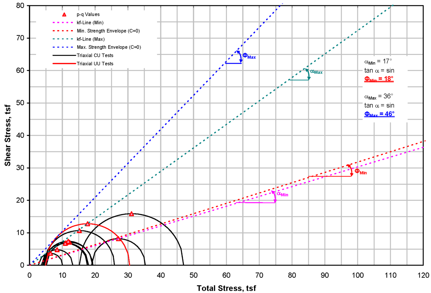
Figure 2.5.4-234 Ultimate Strength of Shale from Consolidated-Undrained and Unconsolidated-Undrained Triaxial Tests
