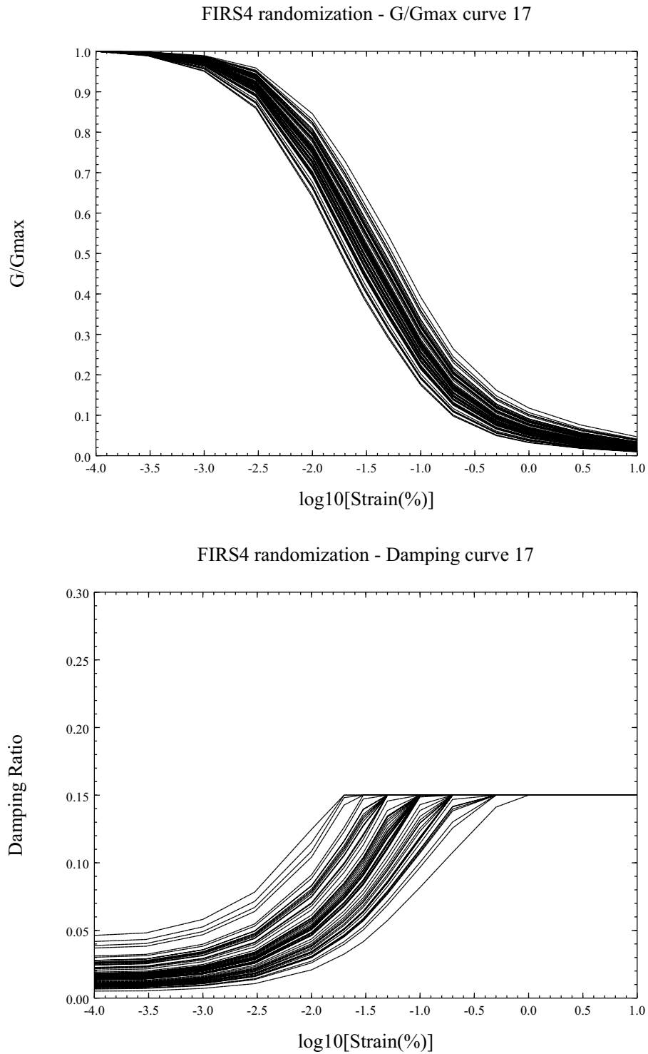
Figure 2.5.2-245 G/Gmax and Damping Ratios vs. Strain for the Fill (0-20 ft depth) in the 60 Synthetic Profiles for FIRS4 Site Column
