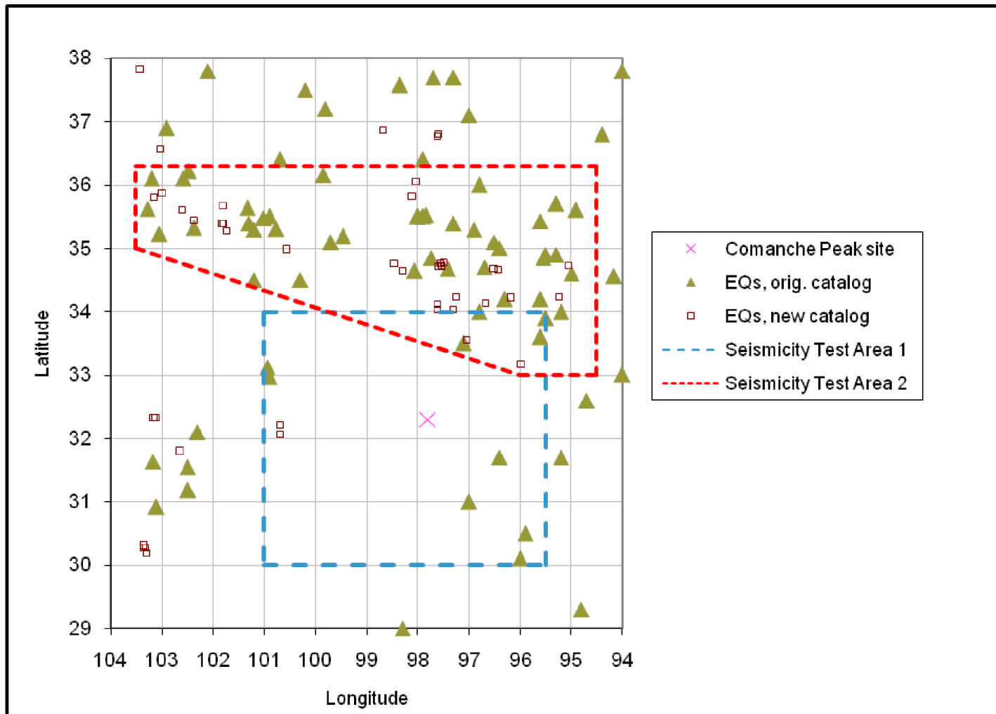
Figure 2.5.2-209 Seismicity from Original Catalog (through 1984), Seismicity from New Catalog (1985-2006) and Regions Used for Test Areas
