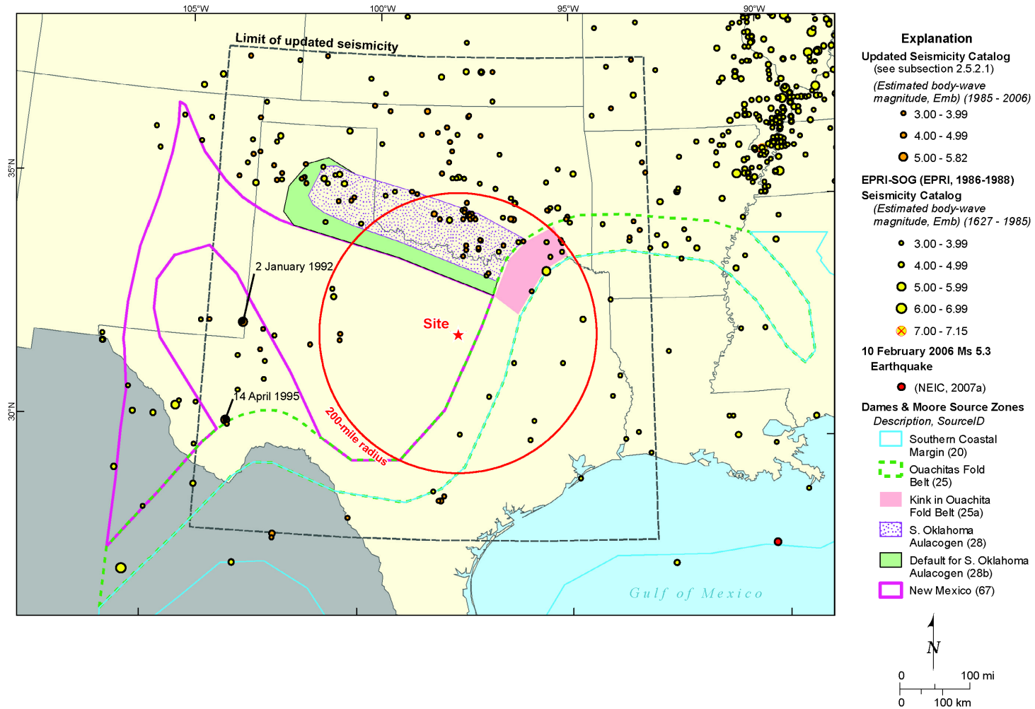
Figure 2.5.2-204 Dames & Moore Contributing EPRI Seismic Source Zones
