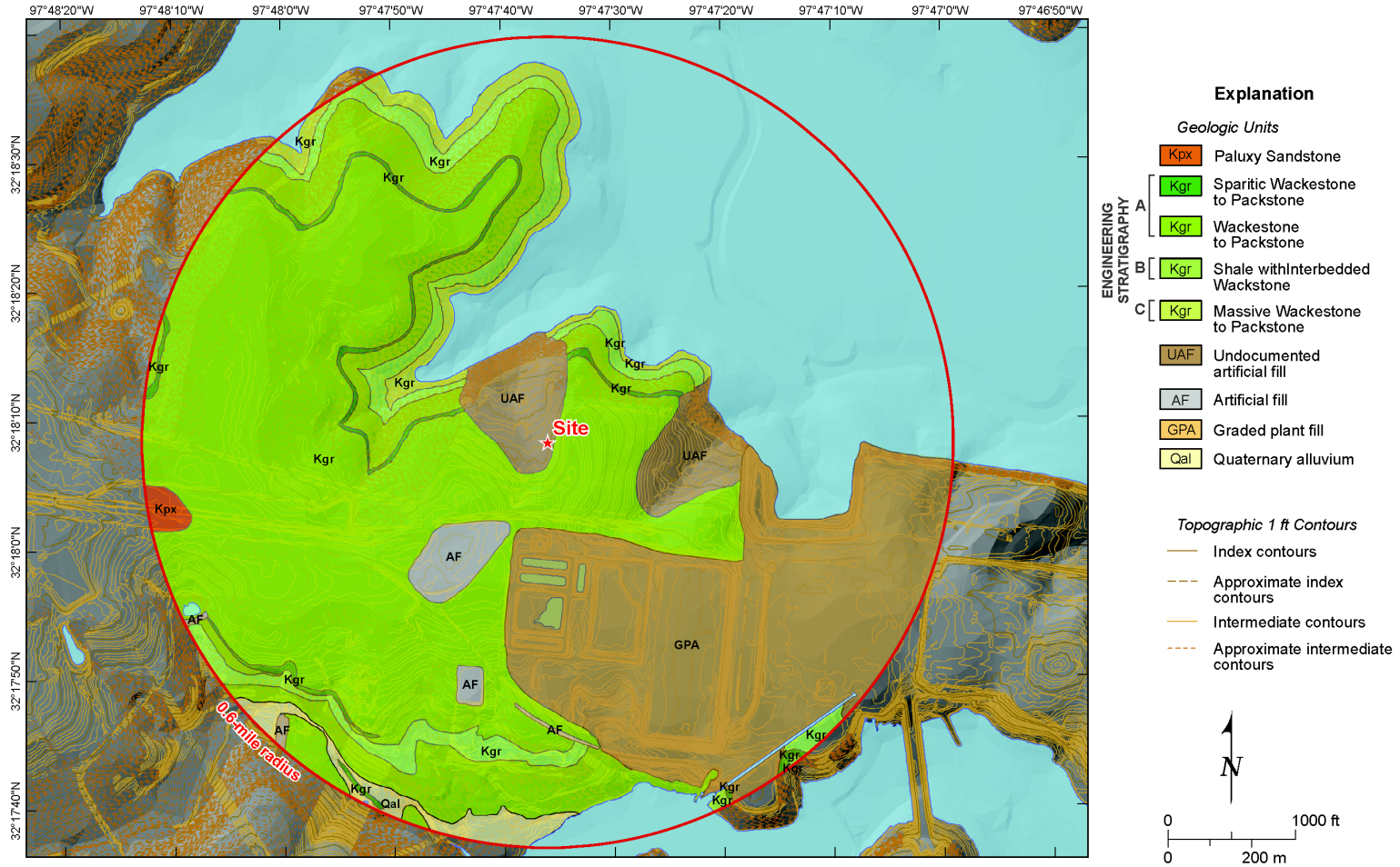
Figure 2.5.1-218 Site Geologic Map (0.6-mile radius)
