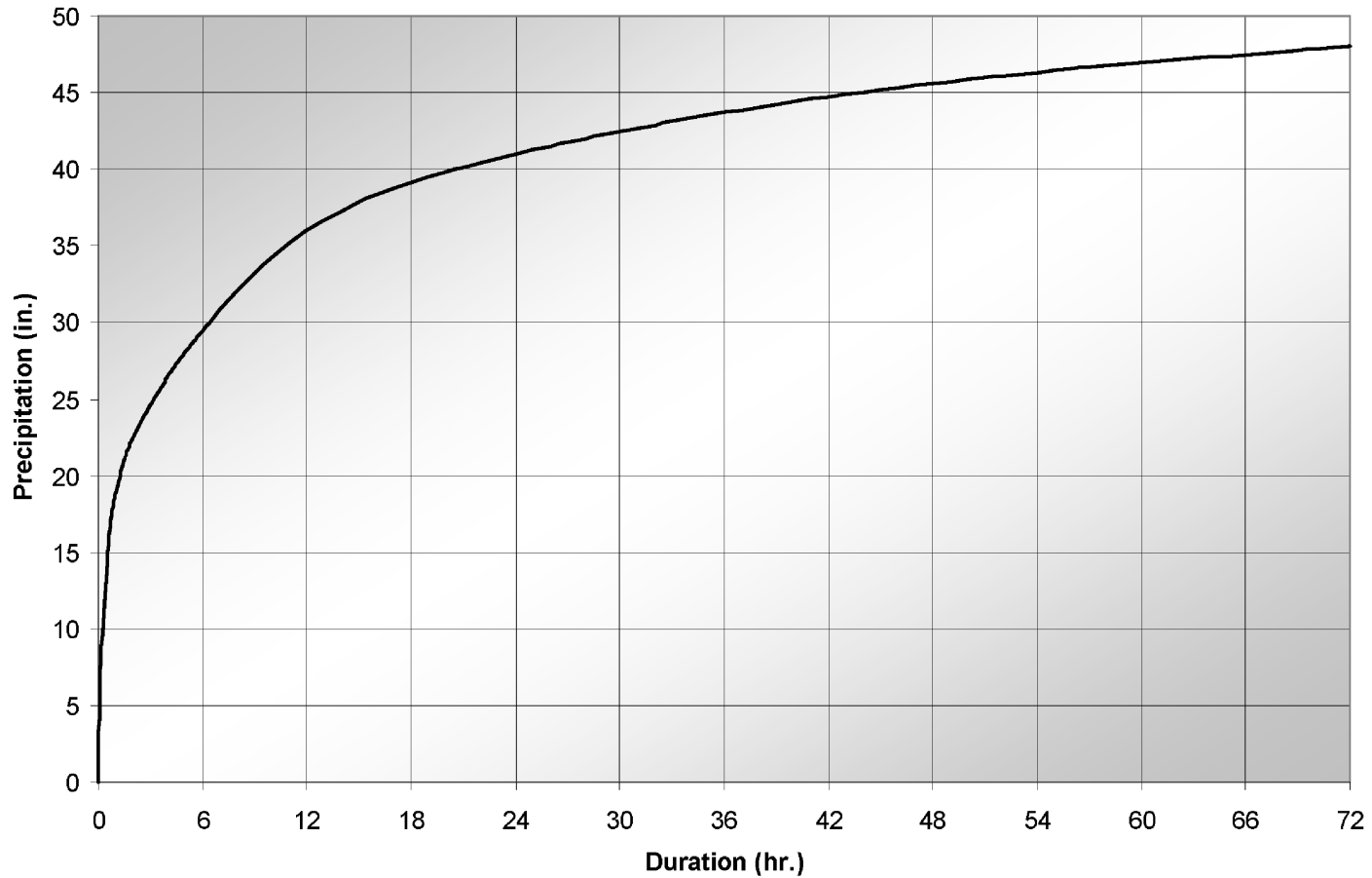
Figure 2.4.2-203 PMP Depth Duration Curve
