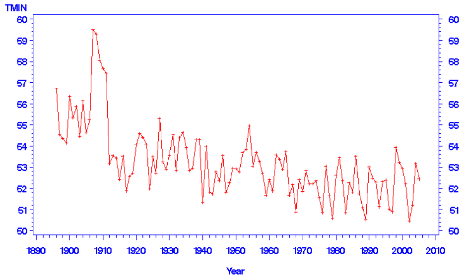
USHCN 412598, DUBLIN, TX Annual mean of Monthly mean minimum temperature (F) 1895 - 2005
