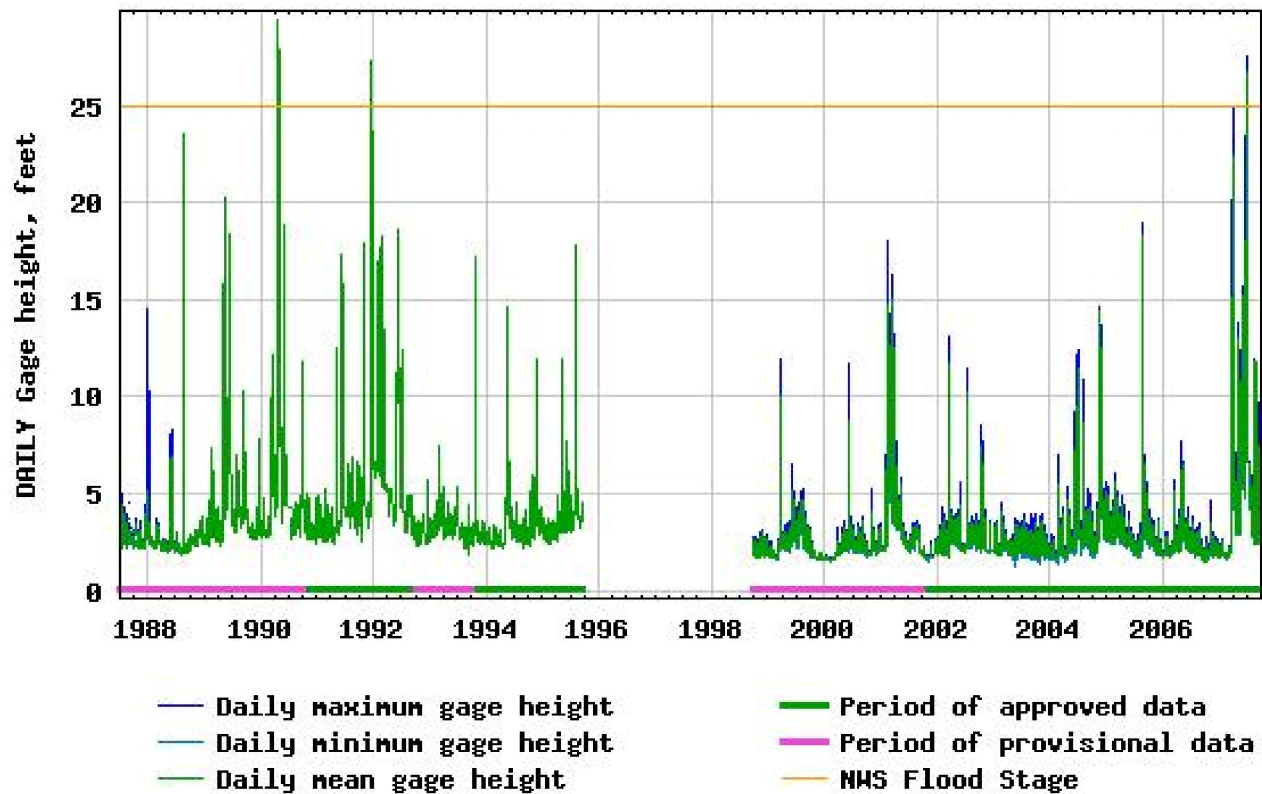
Figure 2.3-7 Floods at USGS 08090800, Brazos River near Dennis, Tx
