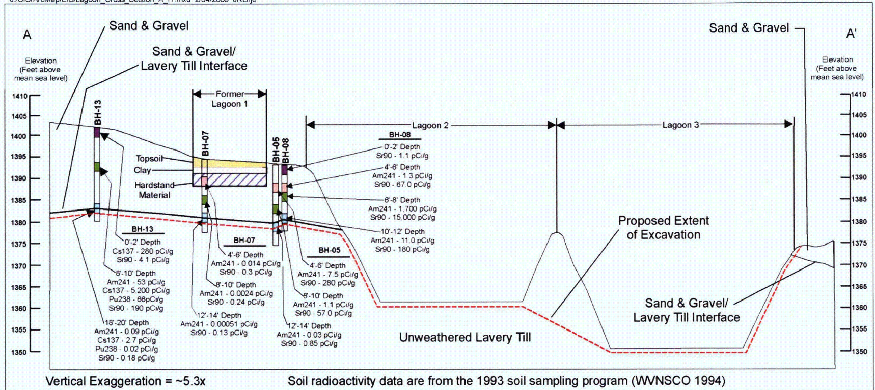
Figure 7-12. Conceptual Arrangement of WMA 2 Excavation, Cross Section
