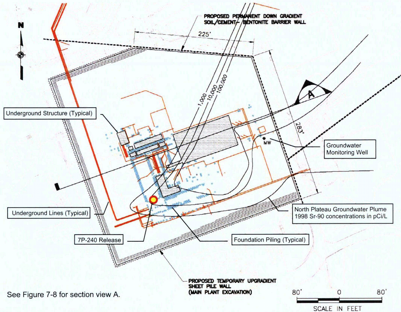
Figure 7-6. Conceptual Layout of WMA 1 Excavation
