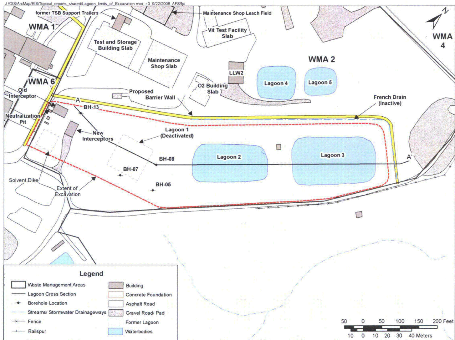
Figure 7-11. Conceptual Arrangement of WMA 2 Excavation, Plan View
